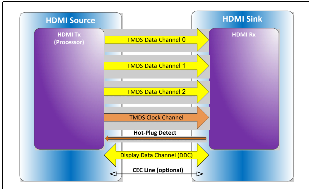
Figure 2-9. HDMI Overview
