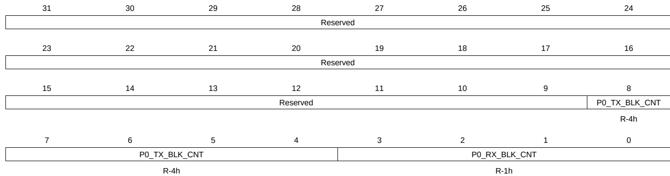
Figure 14-123. P0_BLK_CNT Register
