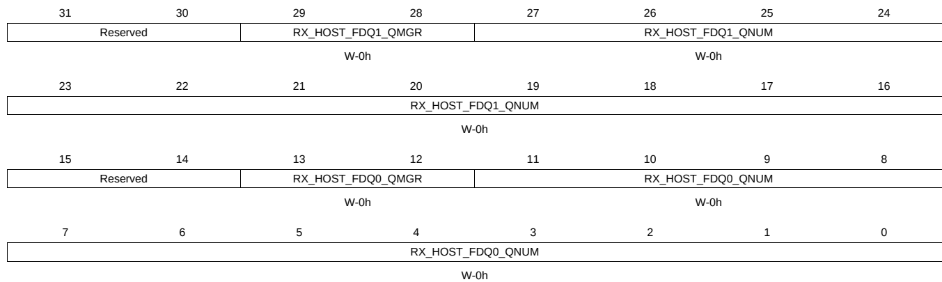
Figure 16-221. RXHPCRA16 Register
