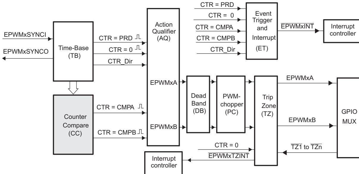
Figure 15-17. Counter-Compare Submodule
