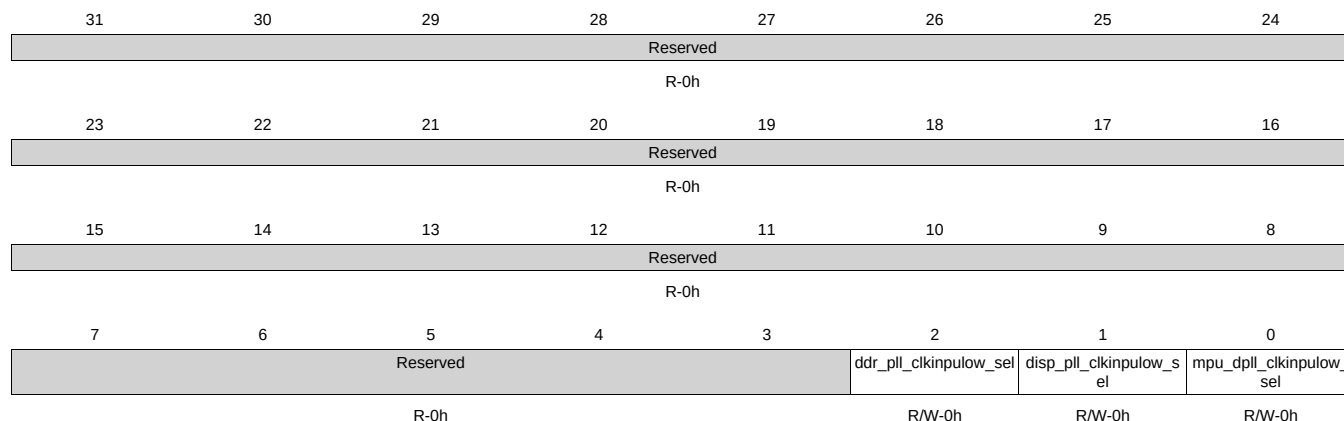
Figure 9-14. pll_clkinpulow_ctrl Register
