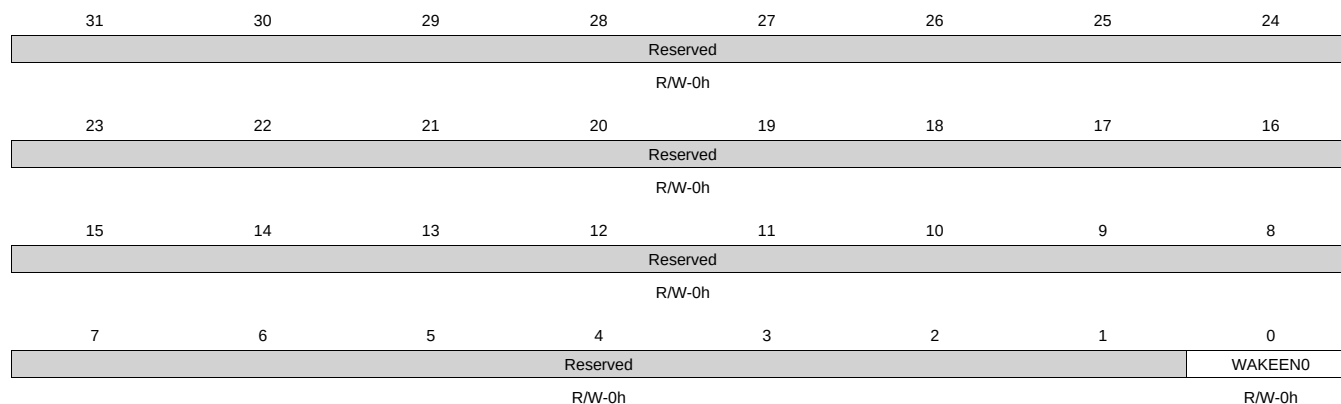
Figure 12-11. IRQWAKEUP Register
