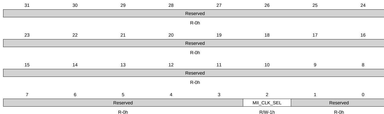
Figure 8-142. CM_MAC_CLKSEL Register
