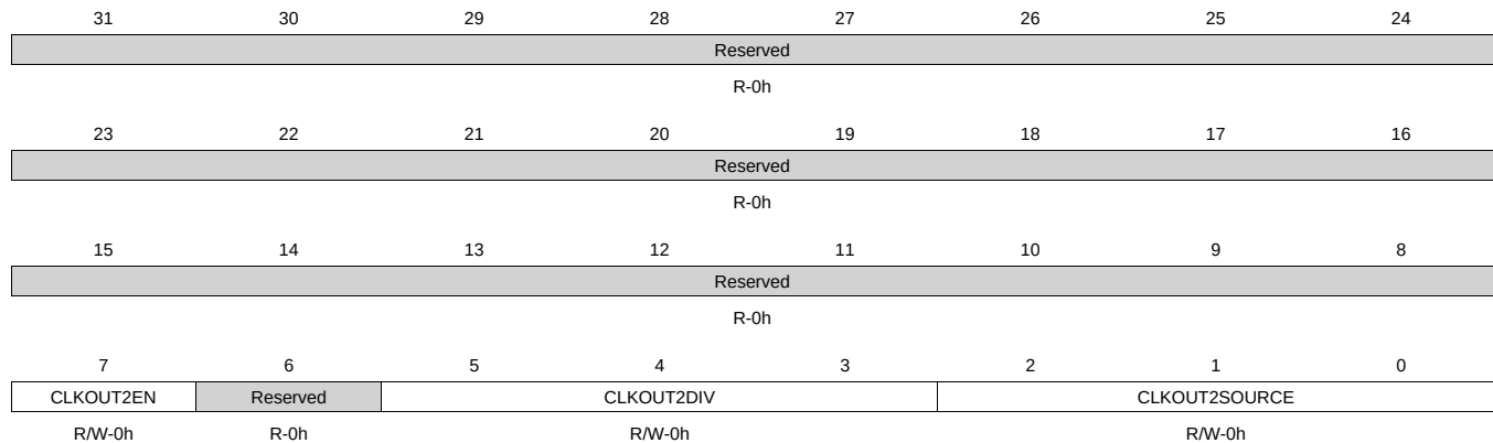
Figure 8-154. CM_CLKOUT_CTRL Register
