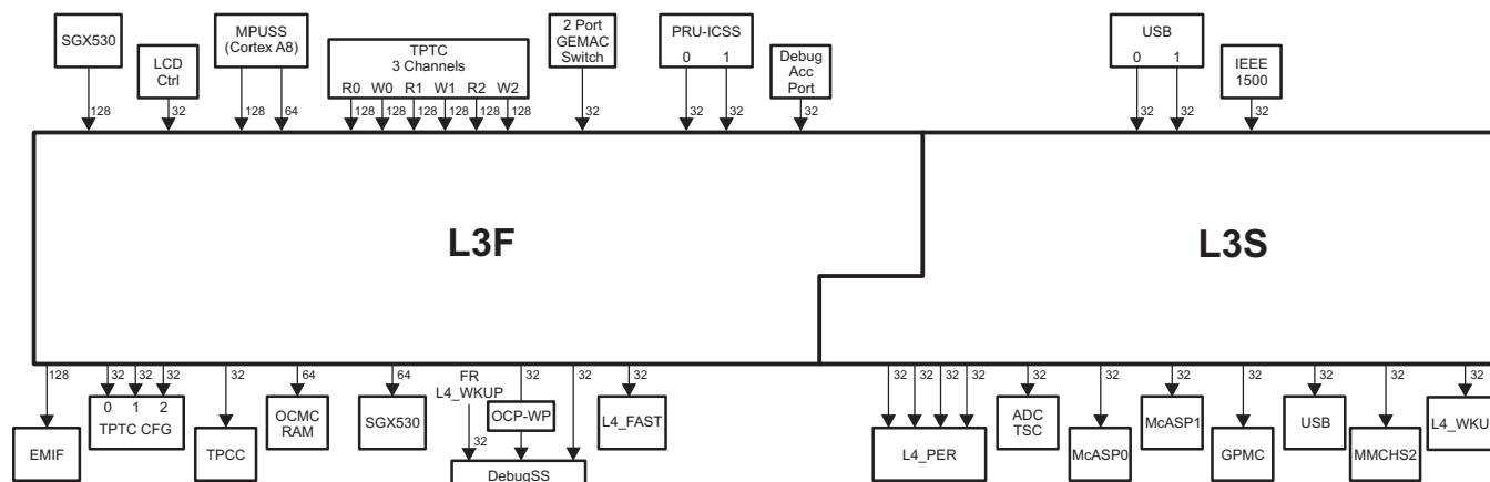
Figure 10-1. L3 Topology
