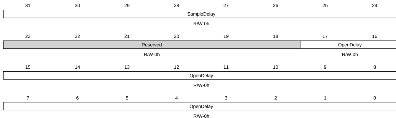
Figure 12-34. STEPDELAY6 Register
