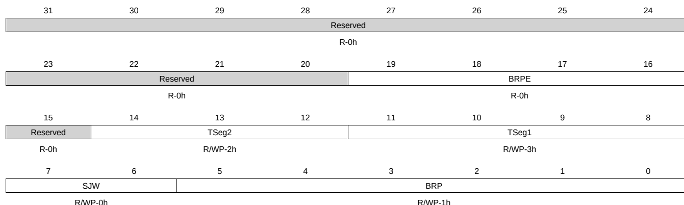
Figure 23-22. BTR Register
