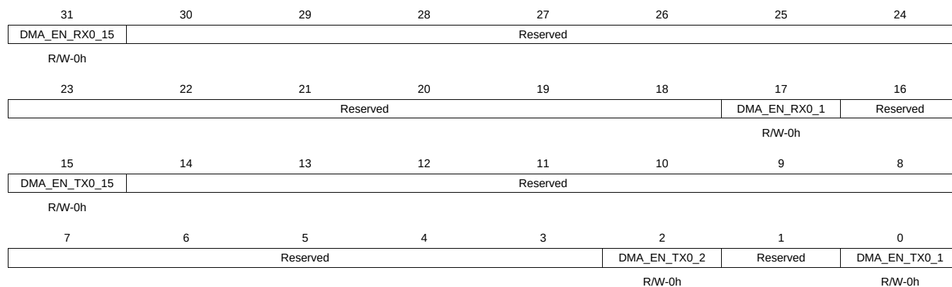
Figure 16-44. IRQDMAENABLE0 Register
