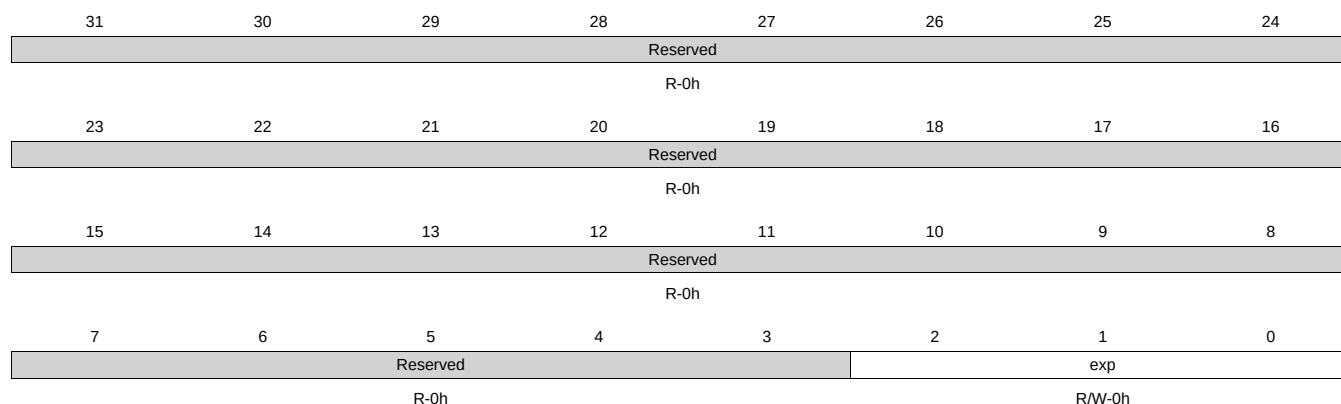
Figure 9-37. mreqprio_1 Register
