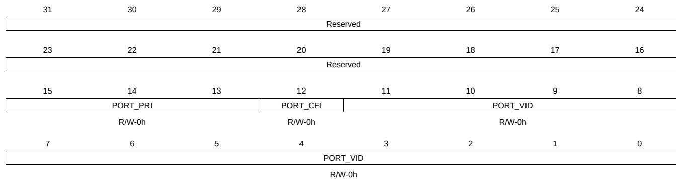
Figure 14-141. P1_PORT_VLAN Register
