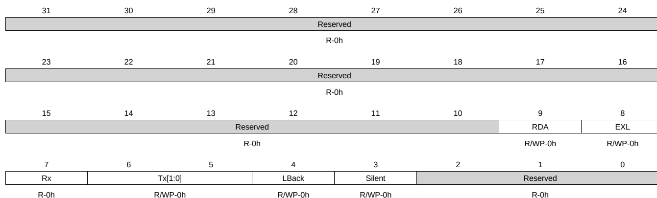
Figure 23-24. TEST Register
