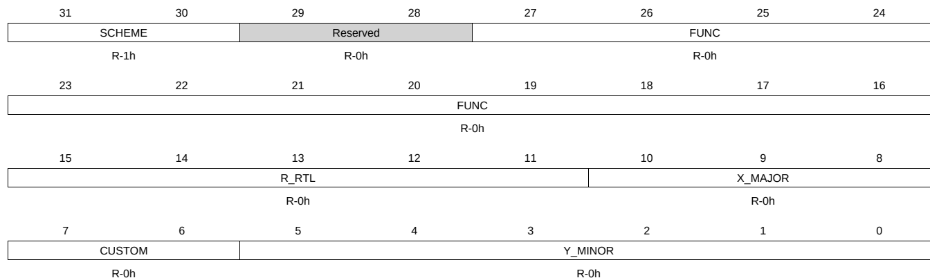
Figure 15-2. IDVER Register
