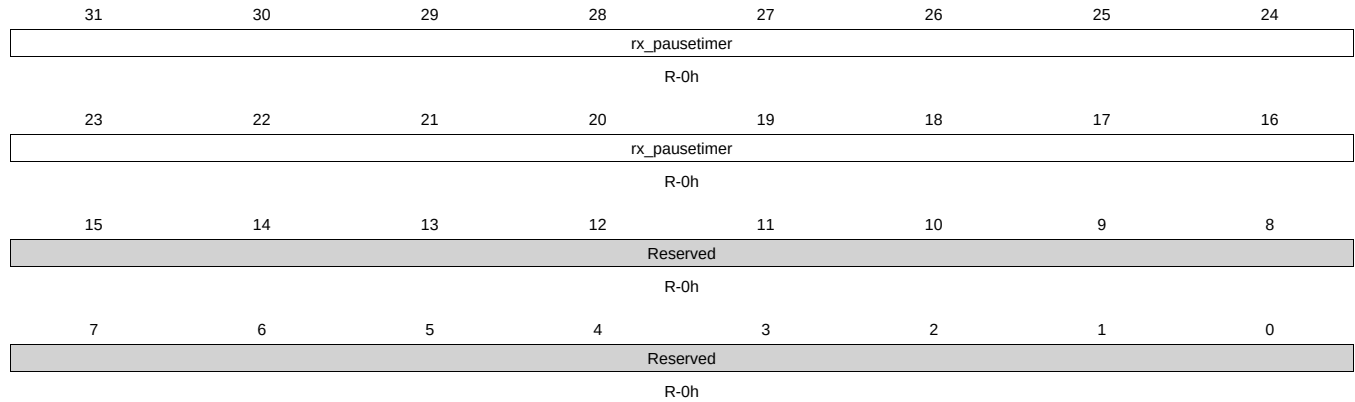
Figure 14-179. RX_PAUSE Register
