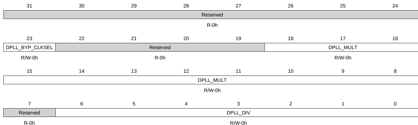
Figure 8-95. CM_CLKSEL_DPLL_MPU Register
