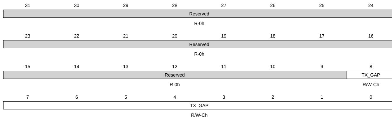
Figure 14-183. TX_GAP Register
