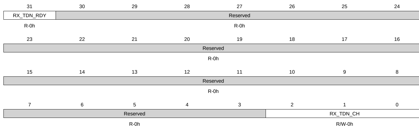
Figure 14-34. RX_TEARDOWN Register
