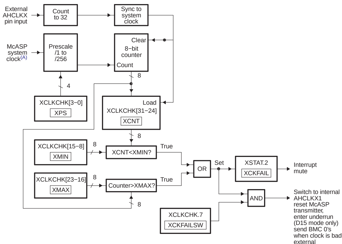
Figure 22-31. Transmit Clock Failure Detection Circuit Block Diagram
