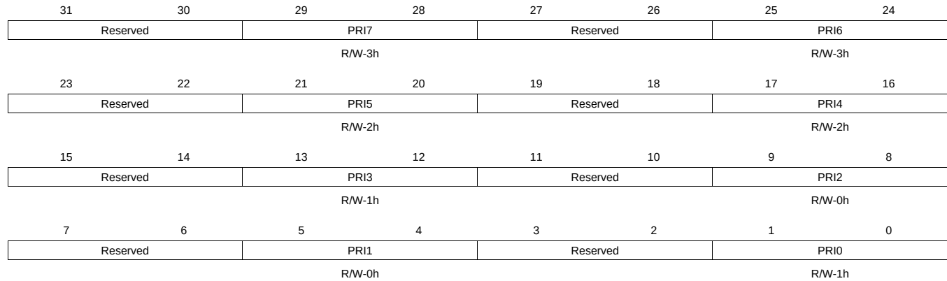
Figure 14-142. P1_TX_PRI_MAP Register
