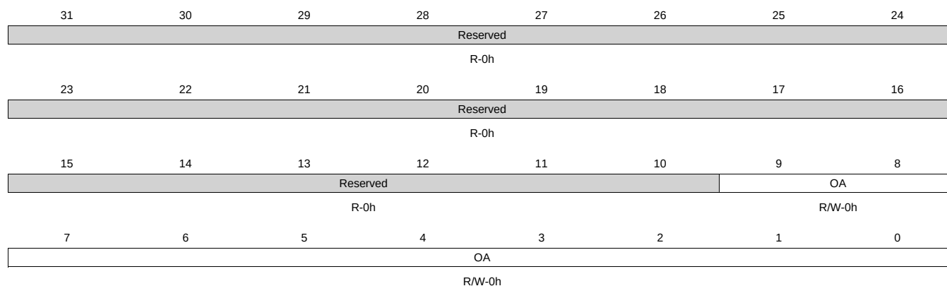
Figure 21-35. I2C_OA Register
