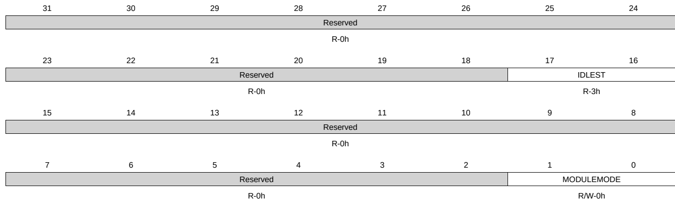
Figure 8-32. CM_PER_OCMCRAM_CLKCTRL Register
