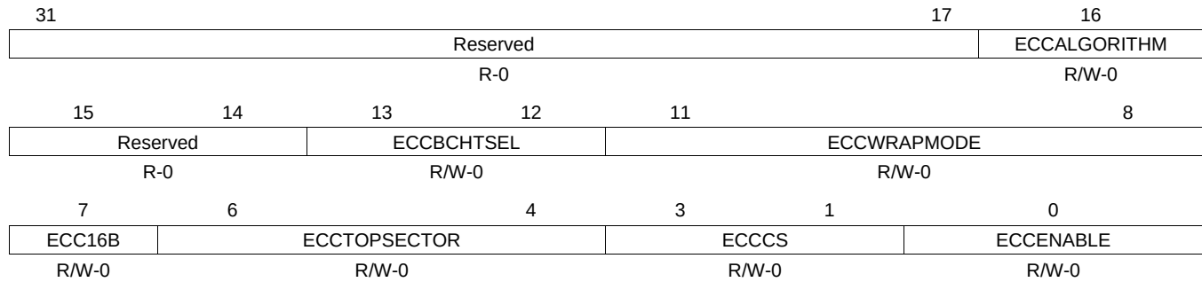
Figure 7-75. GPMC_ECC_CONFIG
