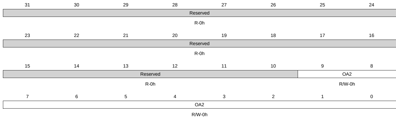
Figure 21-43. I2C_OA2 Register
