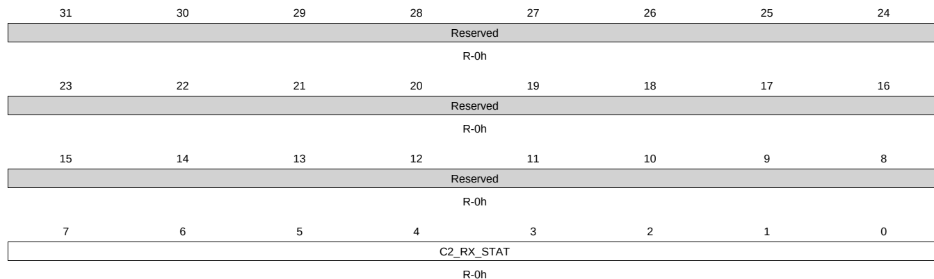
Figure 14-222. C2_RX_STAT Register
