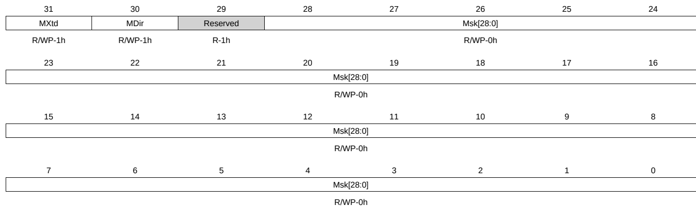
Figure 23-58. IF2MSK Register
