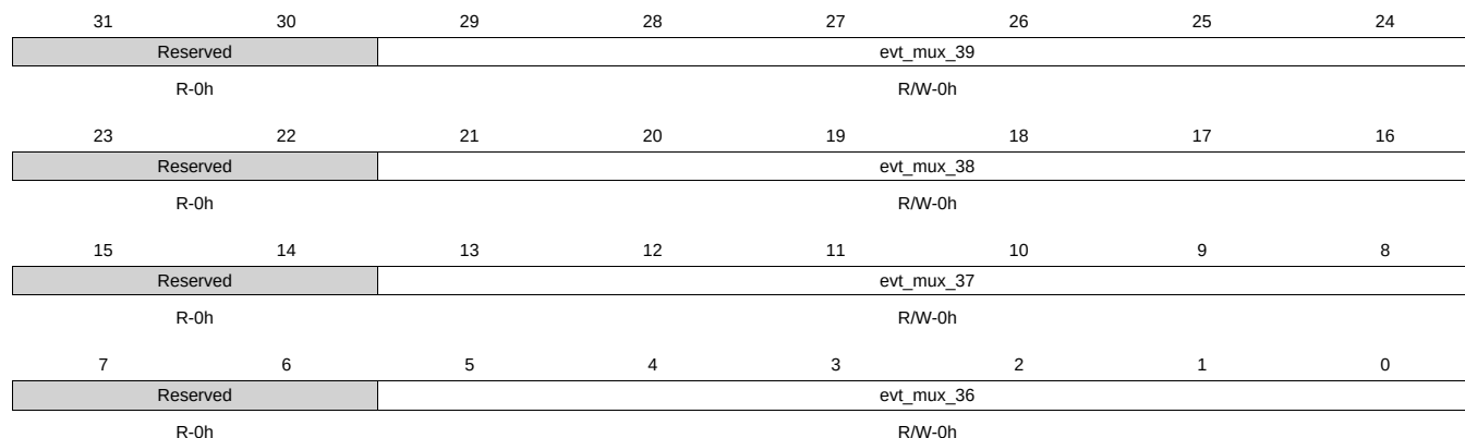
Figure 9-68. tpcc_evt_mux_36_39 Register
