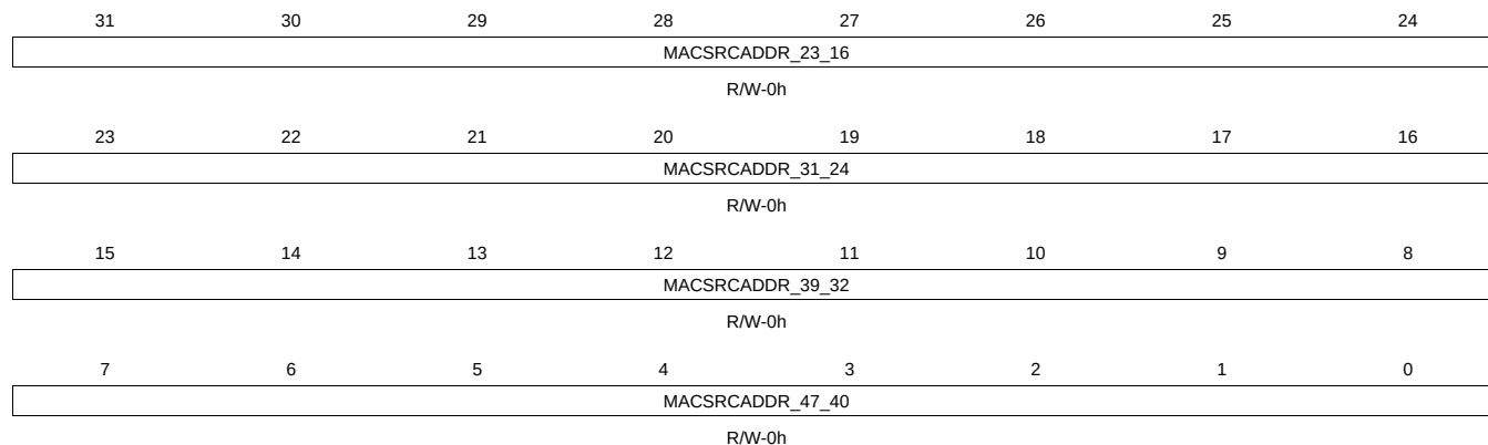
Figure 14-145. P1_SA_HI Register
