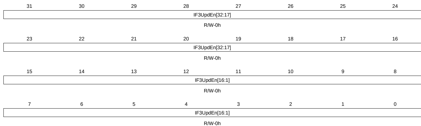
Figure 23-69. IF3UPD12 Register
