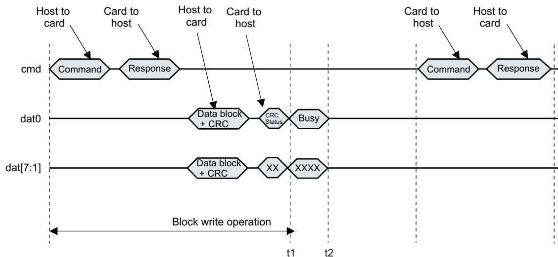
Figure 18-22. Busy Timeout After Write CRC Status
