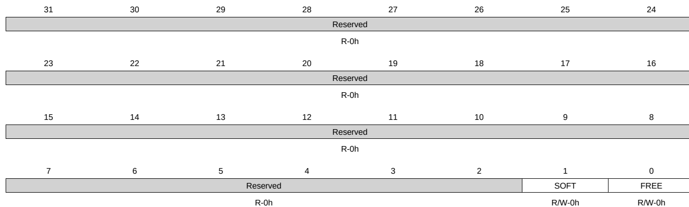
Figure 14-39. EMCONTROL Register
