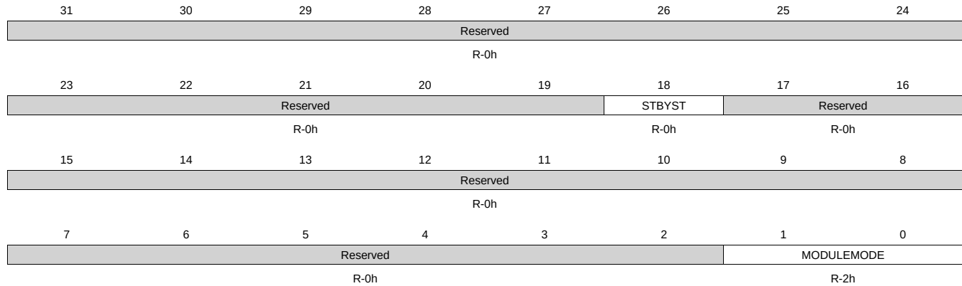
Figure 8-128. CM_WKUP_WKUP_M3_CLKCTRL Register
