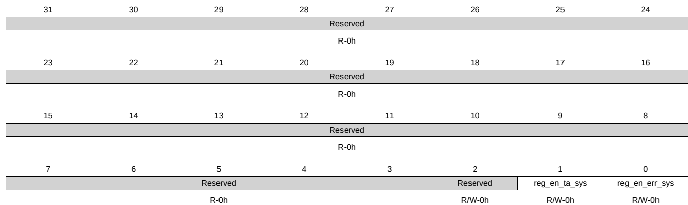
Figure 7-117. IRQENABLE_SET_SYS Register
