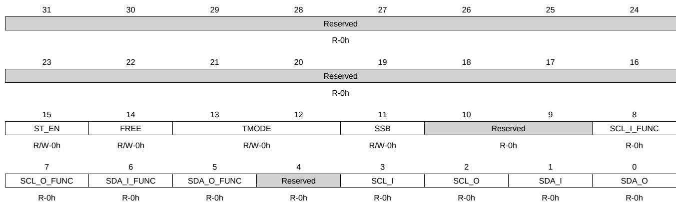
Figure 21-40. I2C_SYSTEST Register
