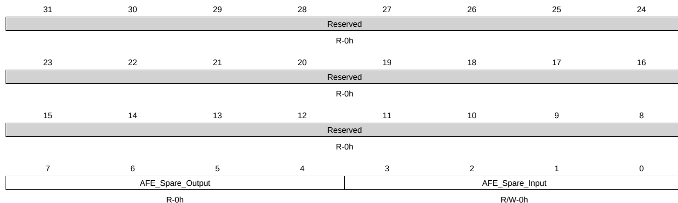
Figure 12-18. ADC_MISC Register
