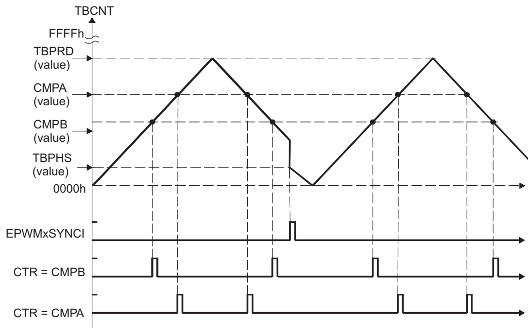
Figure 15-21. Counter-Compare Events in Up-Down-Count Mode, TBCTL[PHSDIR = 0] Count Down on Synchronization Event
