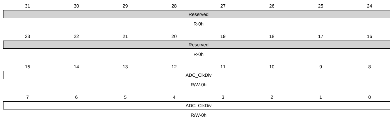
Figure 12-17. ADC_CLKDIV Register
