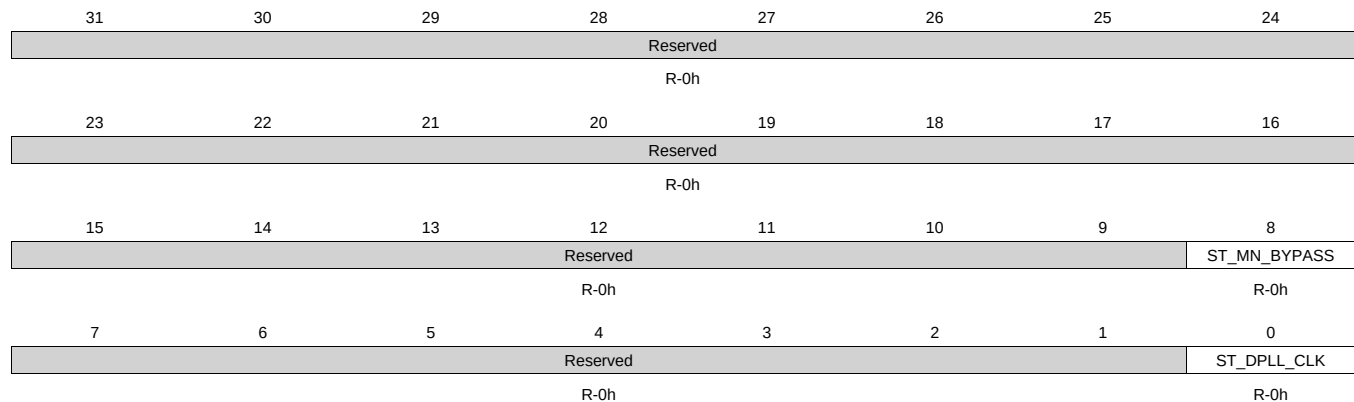
Figure 8-112. CM_IDLEST_DPLL_PER Register
