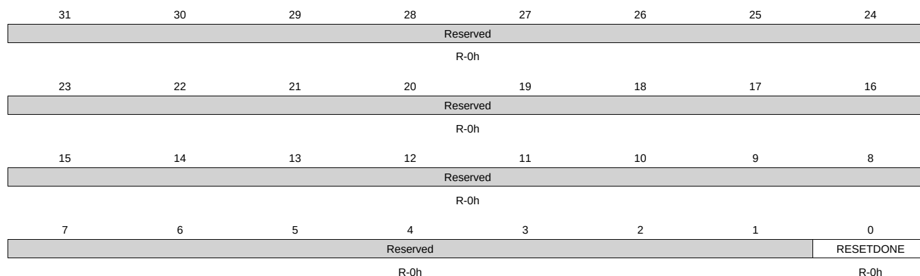
Figure 25-20. GPIO_SYSSTATUS Register
