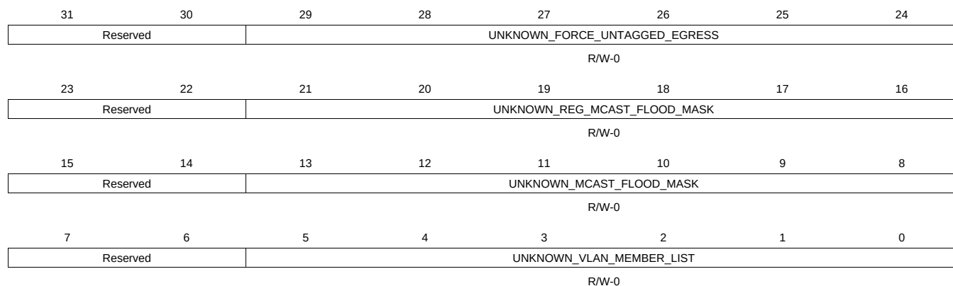
Figure 14-18. UNKNOWN_VLAN Register
