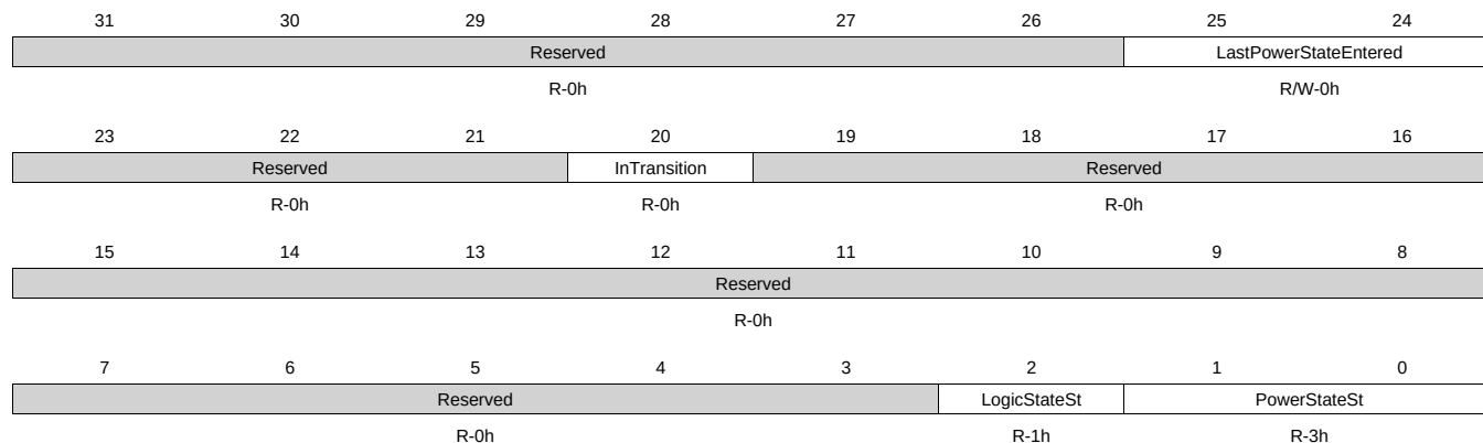
Figure 8-194. PM_CEFUSE_PWRSTST Register
