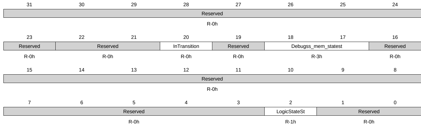
Figure 8-174. PM_WKUP_PWRSTST Register
