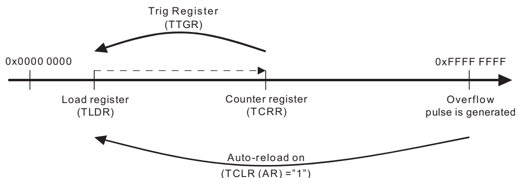
Figure 20-28. TCRR Timing Value
