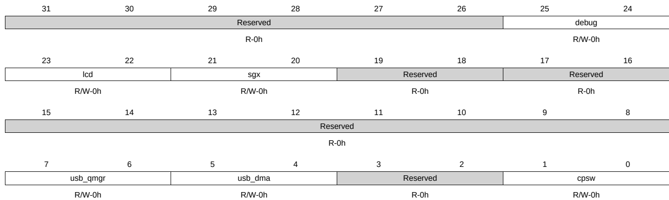
Figure 9-21. init_priority_1 Register
