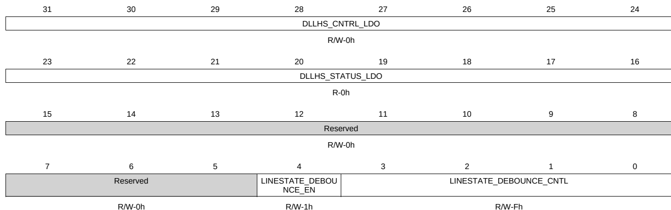
Figure 16-136. DLLHS_2 Register
