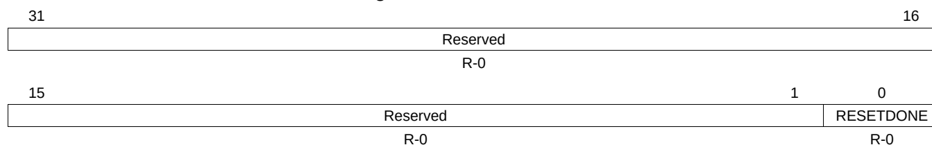
Figure 7-53. GPMC_SYSSTATUS
