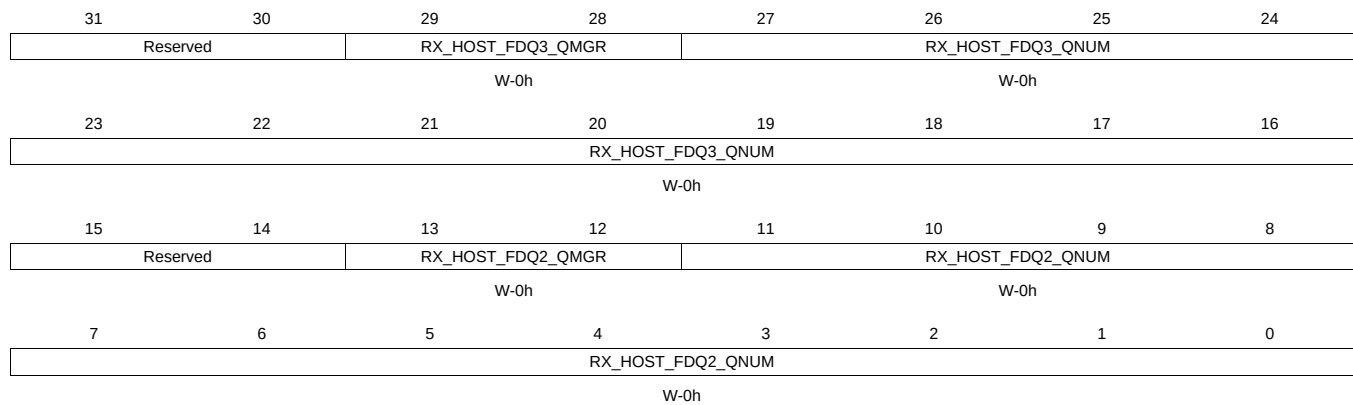
Figure 16-170. RXHPCRB3 Register
