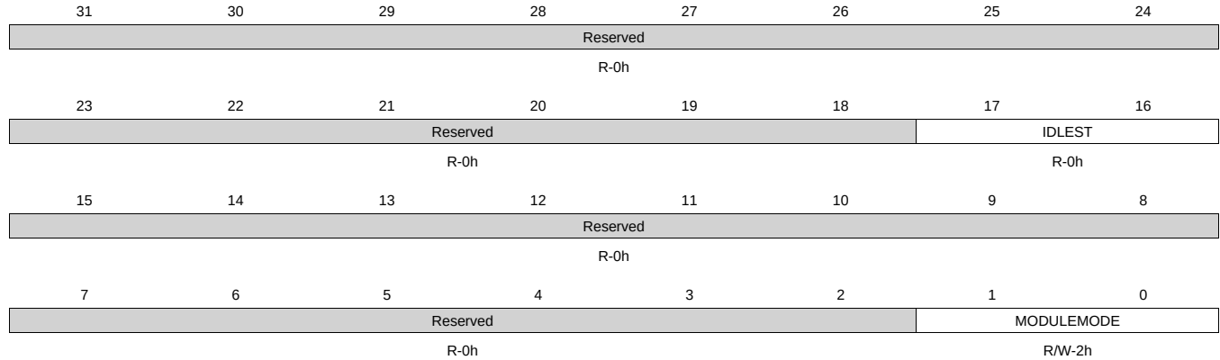
Figure 8-63. CM_PER_L3_INSTR_CLKCTRL Register
