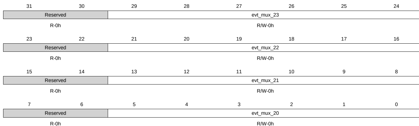
Figure 9-64. tpcc_evt_mux_20_23 Register
