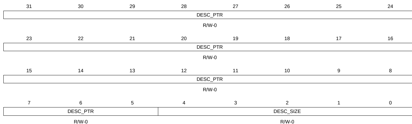
Figure 16-722. QUEUE_102_D Register
