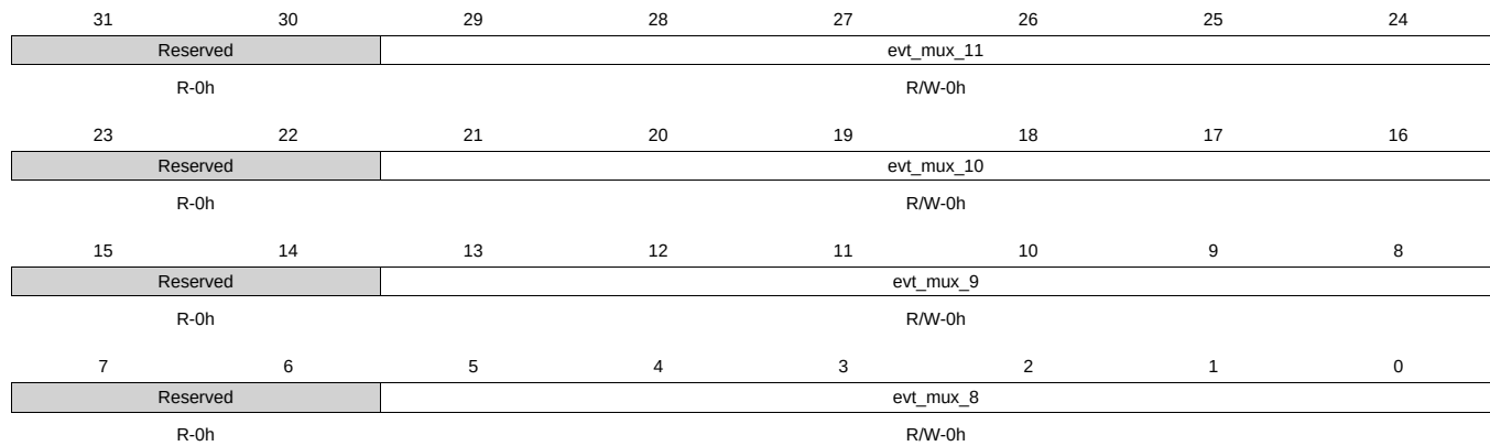
Figure 9-61. tpcc_evt_mux_8_11 Register
