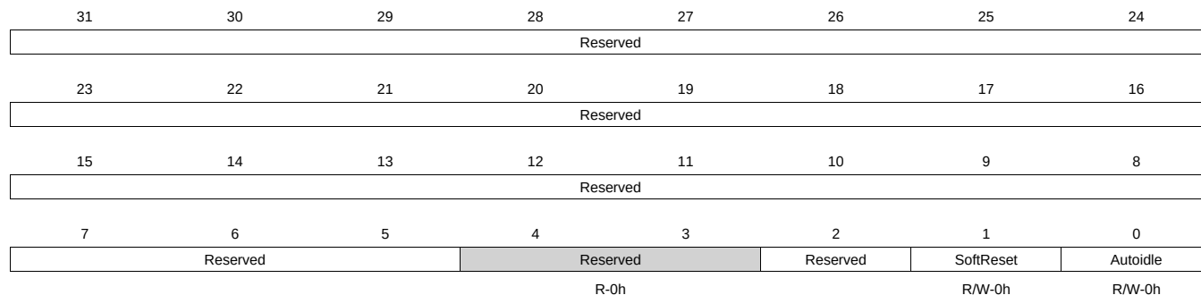
Figure 6-5. INTC_SYSCONFIG Register
