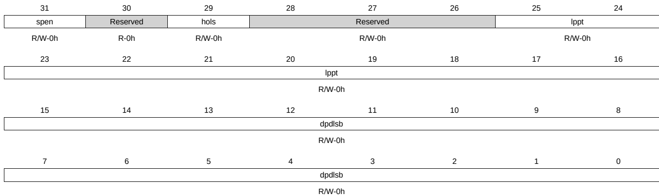
Figure 13-32. RASTER_SUBPANEL Register
