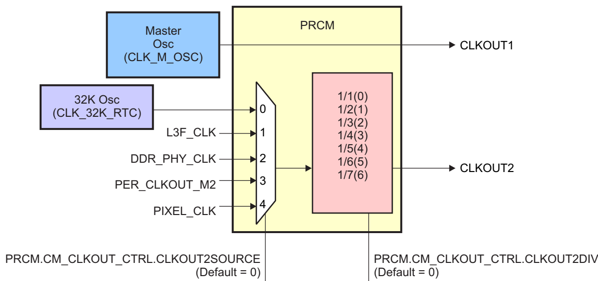
Figure 8-15. CLKOUT Signals
