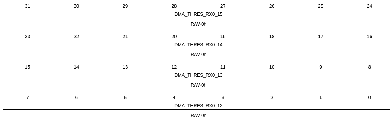
Figure 16-35. IRQDMATHOLDRX03 Register
