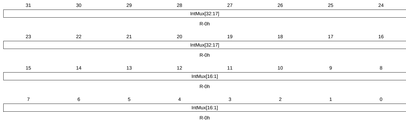
Figure 23-47. INTMUX12 Register
