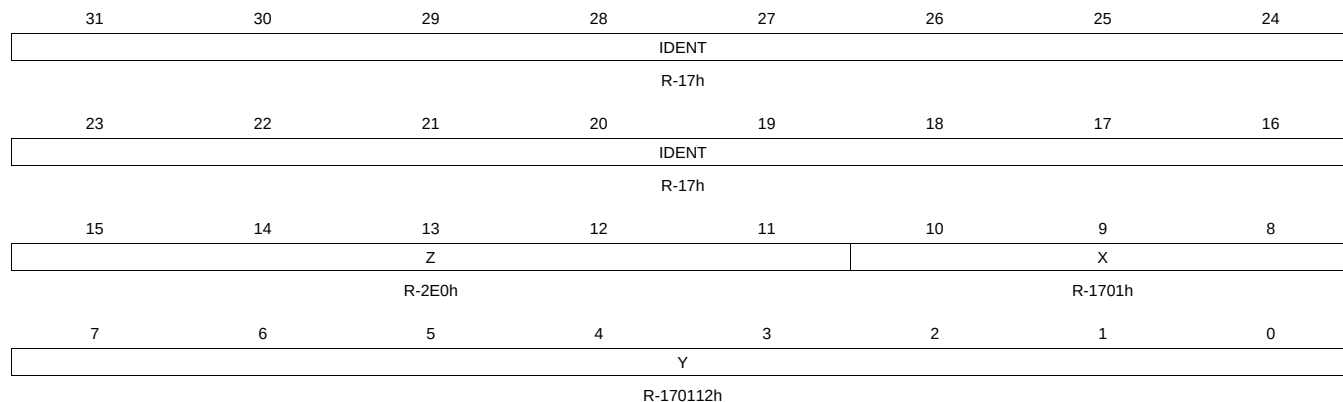
Figure 14-173. IDVER Register
