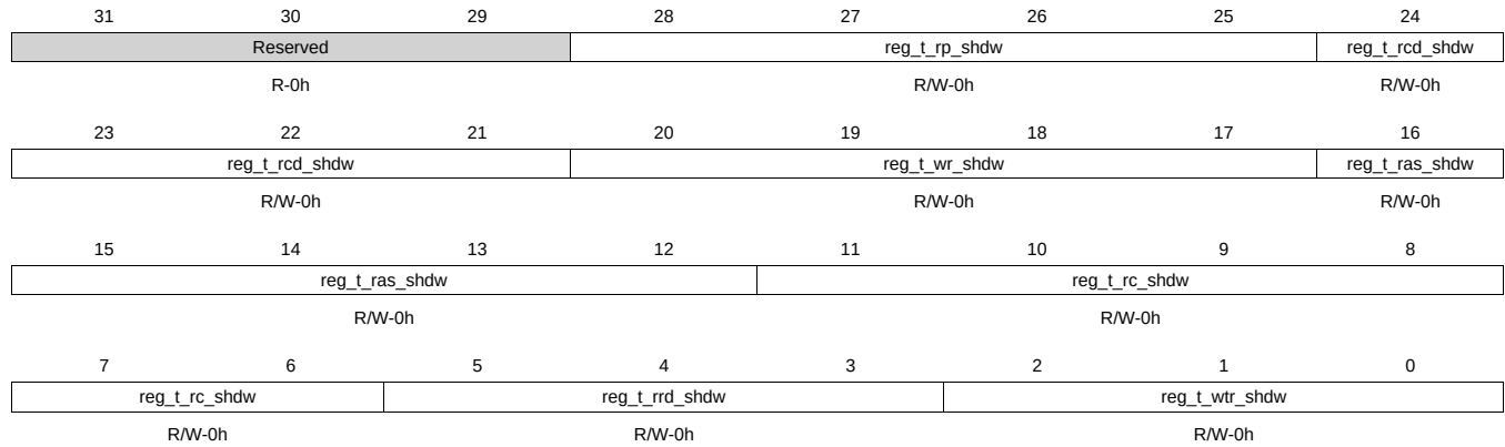
Figure 7-98. SDRAM_TIM_1_SHDW Register
