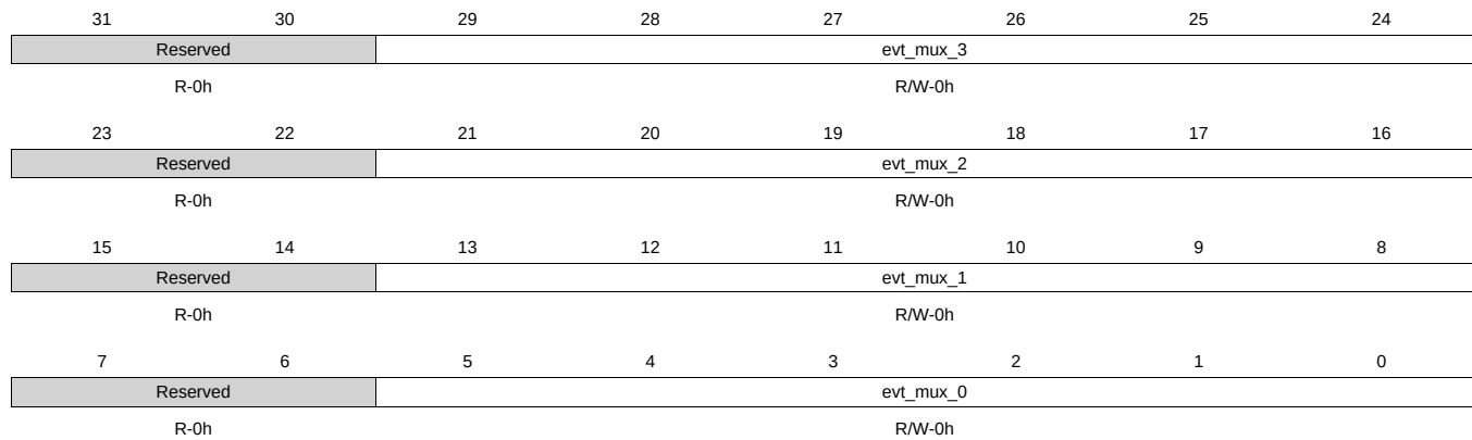
Figure 9-59. tpcc_evt_mux_0_3 Register
