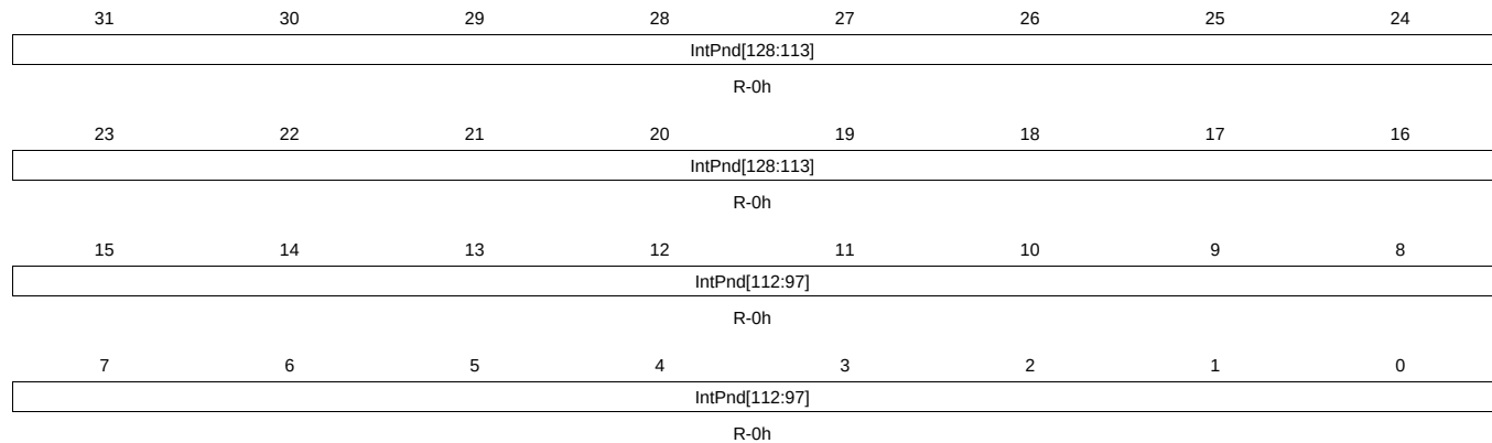
Figure 23-41. INTPND78 Register
