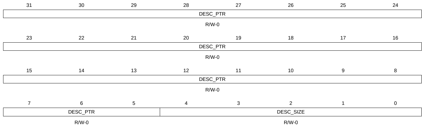
Figure 16-806. QUEUE_123_D Register
