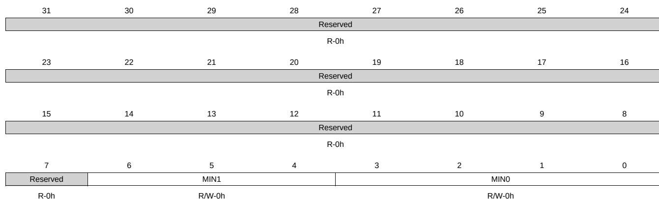
Figure 20-62. MINUTES_REG Register
