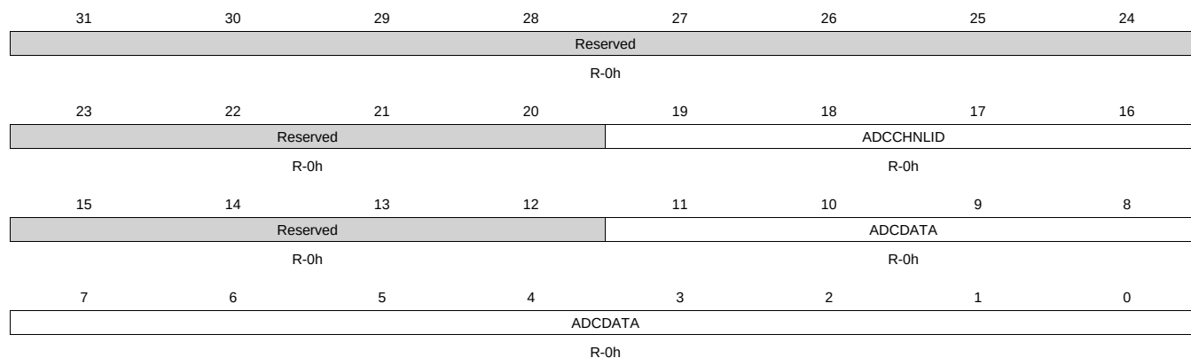
Figure 12-61. FIFO0DATA Register
