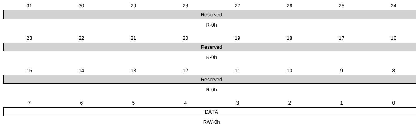
Figure 21-33. I2C_DATA Register
