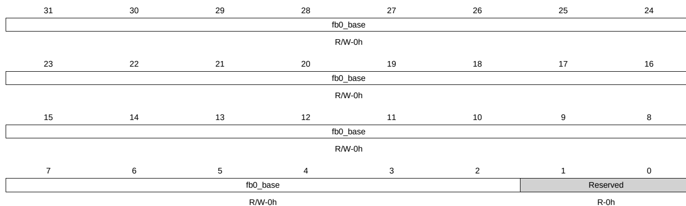
Figure 13-35. LCDDMA_FB0_BASE Register
