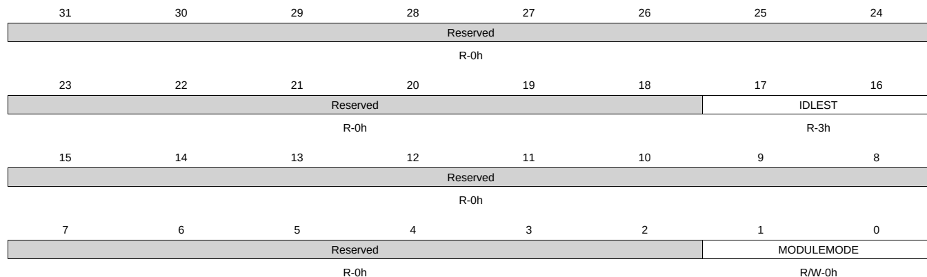
Figure 8-131. CM_WKUP_ADC_TSC_CLKCTRL Register
