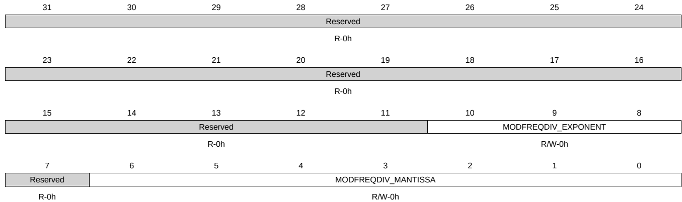
Figure 8-99. CM_SSC_MODFREQDIV_DPLL_DDR Register
