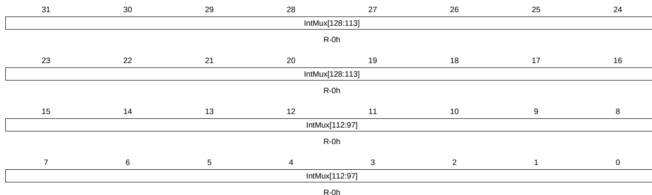
Figure 23-50. INTMUX78 Register
