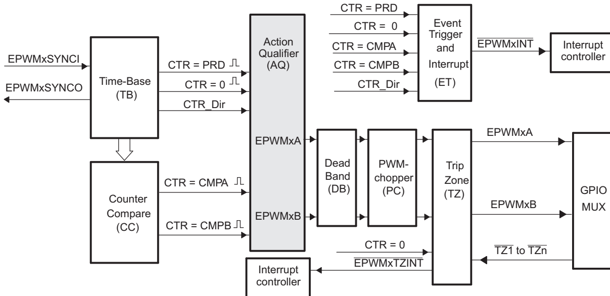
Figure 15-23. Action-Qualifier Submodule
