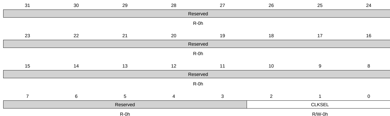
Figure 8-146. CLKSEL_TIMER1MS_CLK Register
