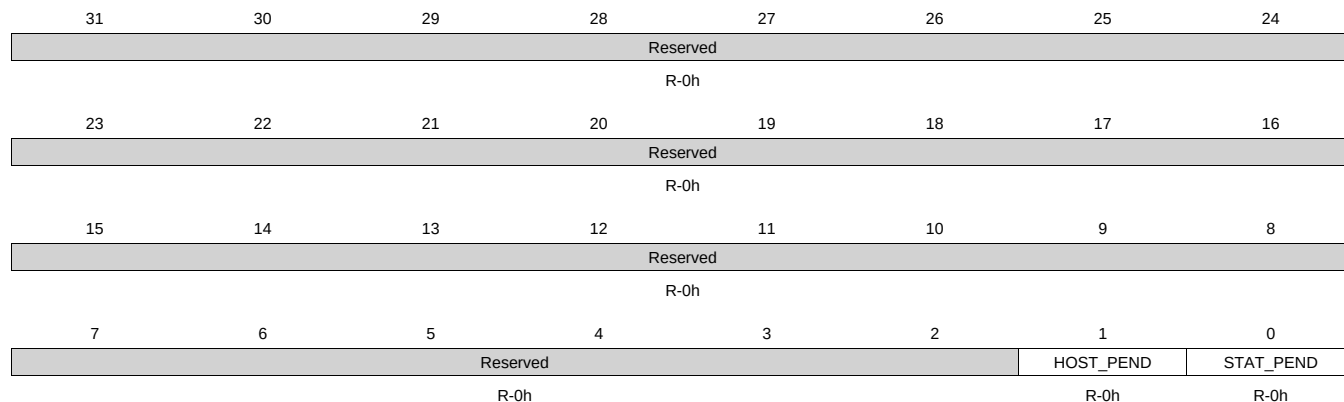
Figure 14-59. DMA_INTSTAT_MASKED Register
