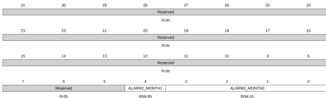
Figure 20-92. ALARM2_MONTHS_REG Register
