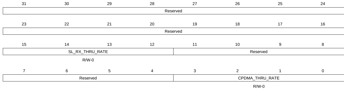
Figure 14-190. THRU_RATE Register
