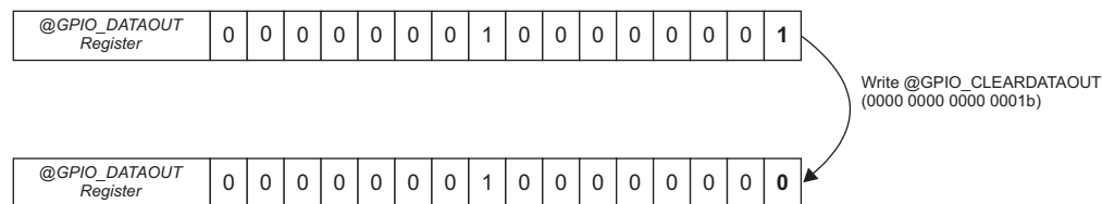
Figure 25-4. Write @ GPIO_CLEARDATAOUT Register Example
