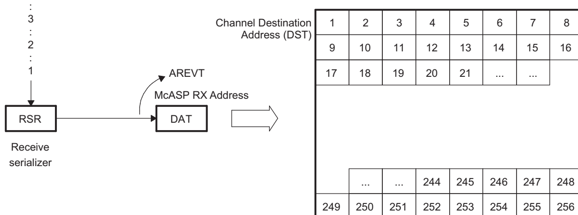
Figure 11-29. Servicing Incoming McASP Data Example PaRAM Configuration
