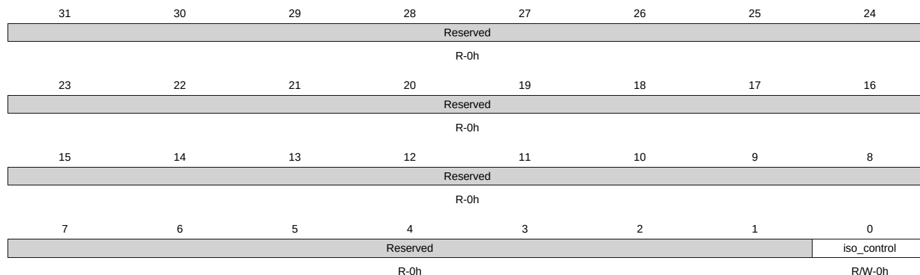
Figure 9-78. reset_iso Register
