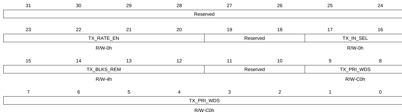
Figure 14-124. P0_TX_IN_CTL Register
