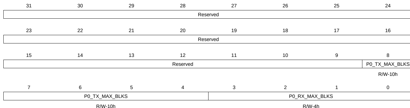
Figure 14-122. P0_MAX_BLKs Register
