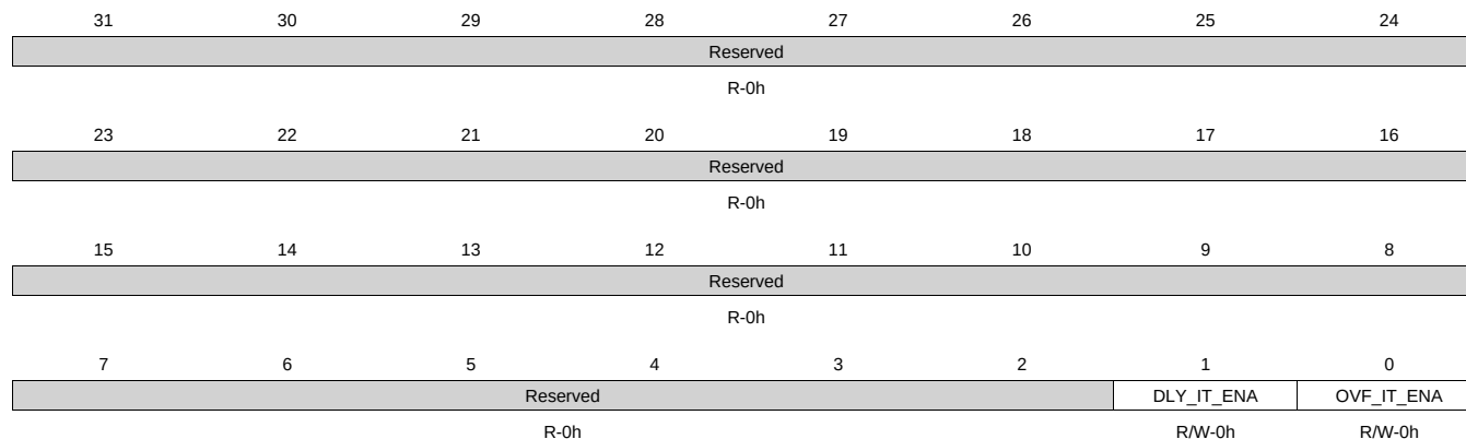
Figure 20-103. WDT_WIER Register
