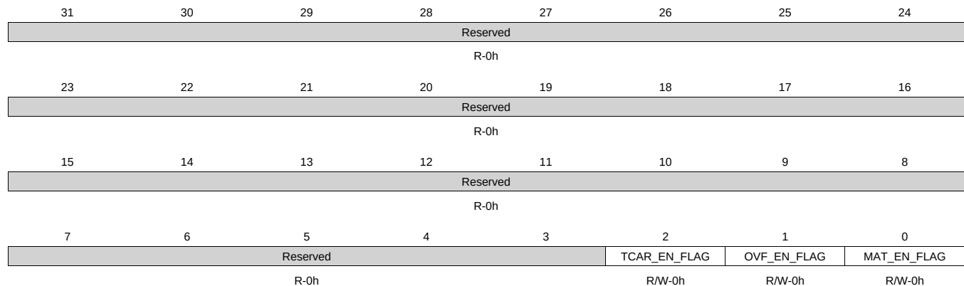
Figure 20-15. IRQENABLE_CLR Register
