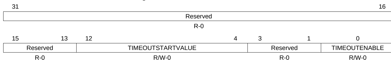
Figure 7-56. GPMC_TIMEOUT_CONTROL
