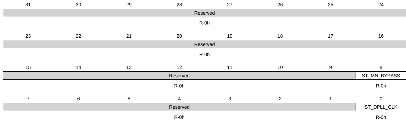
Figure 8-102. CM_IDLEST_DPLL_DISP Register
