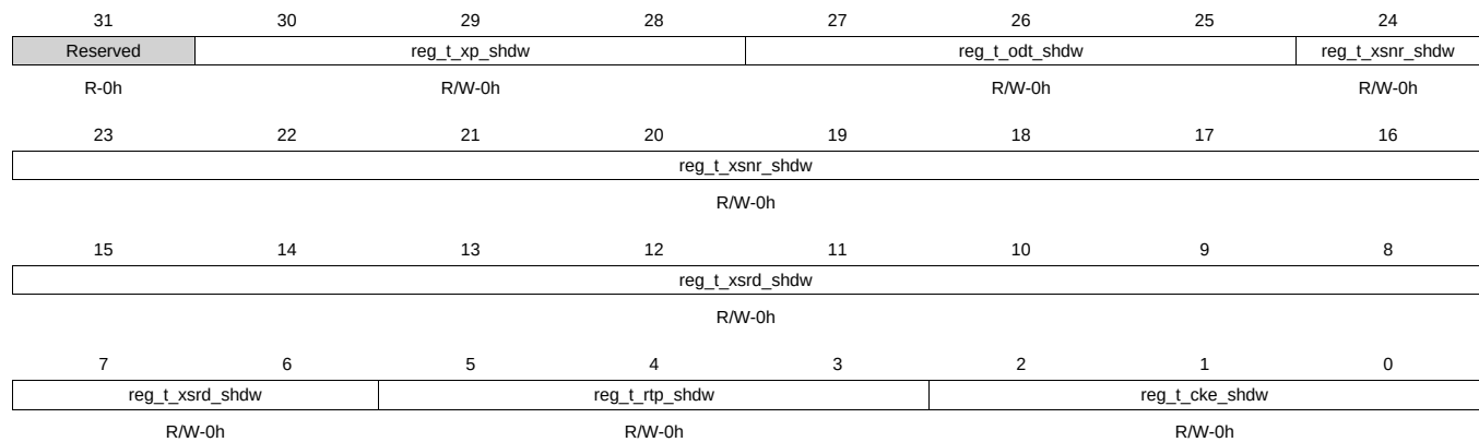
Figure 7-100. SDRAM_TIM_2_SHDW Register
