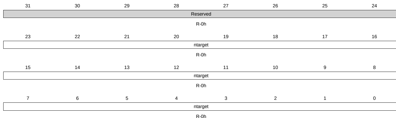
Figure 9-48. vdd_mpu_opp_turbo Register
