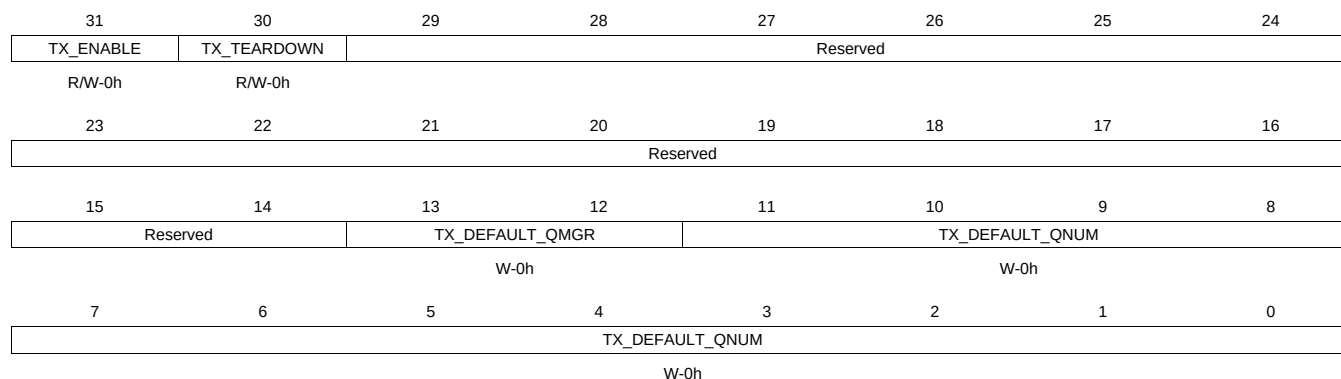
Figure 16-251. TXGCR24 Register
