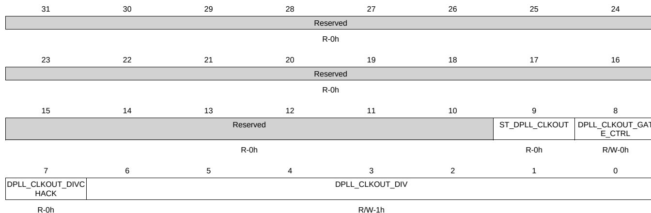
Figure 8-127. CM_DIV_M2_DPLL_PER Register
