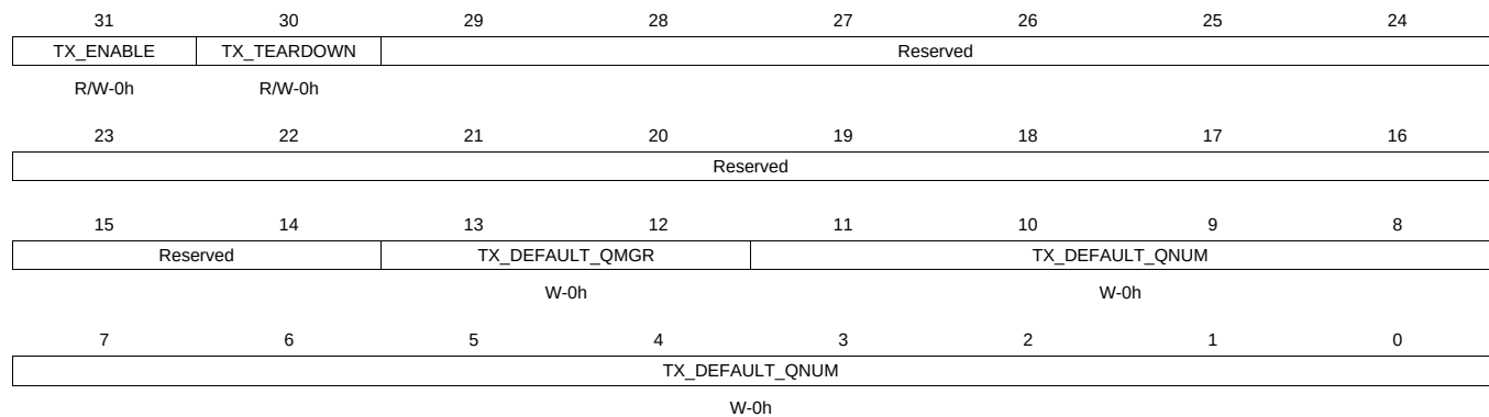
Figure 16-159. TXGCR1 Register
