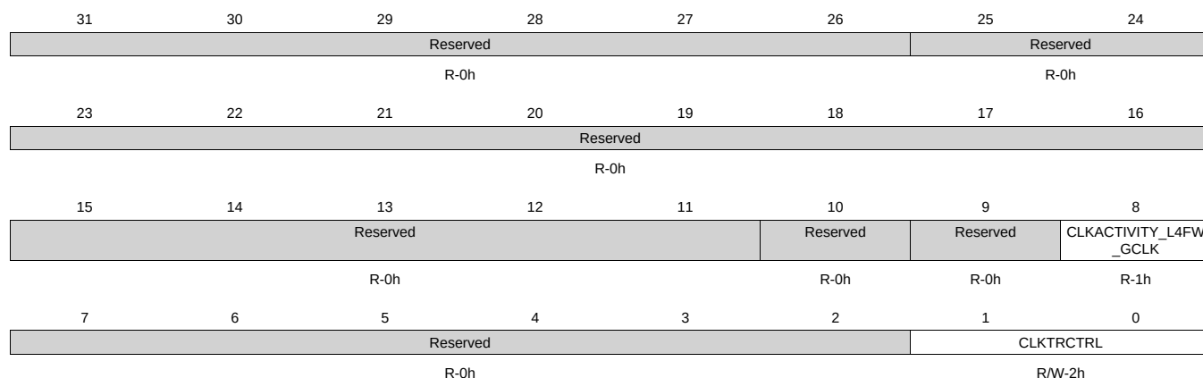
Figure 8-25. CM_PER_L4FW_CLKSTCTRL Register
