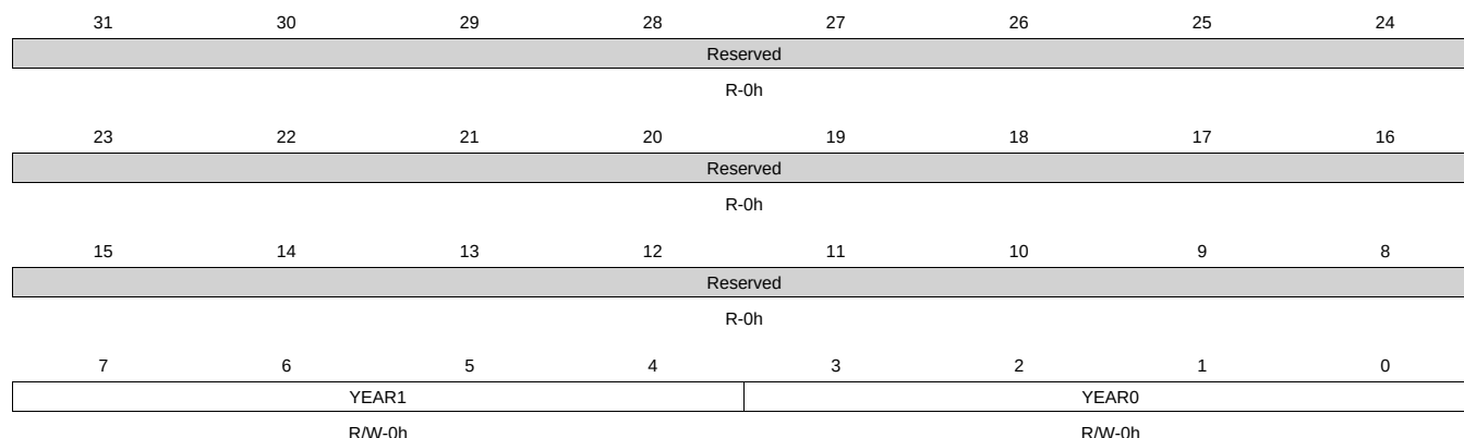
Figure 20-66. YEARS_REG Register
