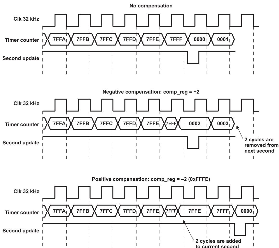
Figure 20-60. Compensation Illustration
