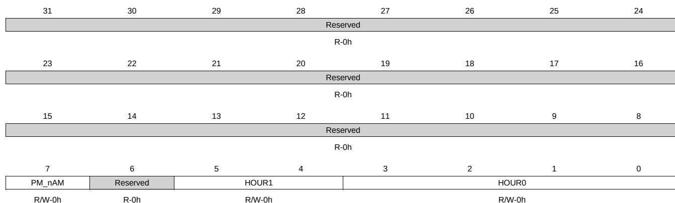
Figure 20-63. HOURS_REG Register
