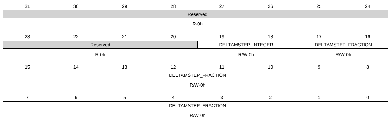
Figure 8-98. CM_SSC_DELTAMSTEP_DPLL_DDR Register
