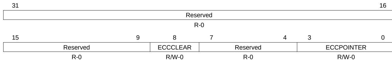
Figure 7-76. GPMC_ECC_CONTROL
