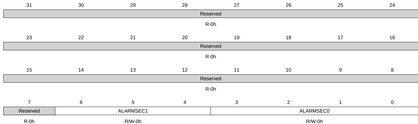
Figure 20-68. ALARM_SECONDS_REG Register
