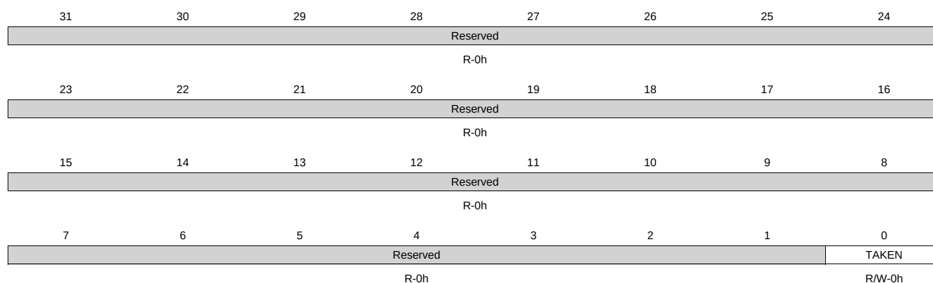
Figure 17-69. LOCK_REG_21 Register
