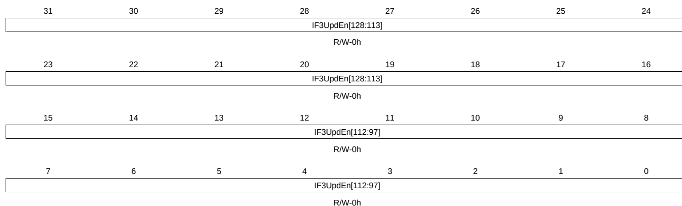
Figure 23-72. IF3UPD78 Register
