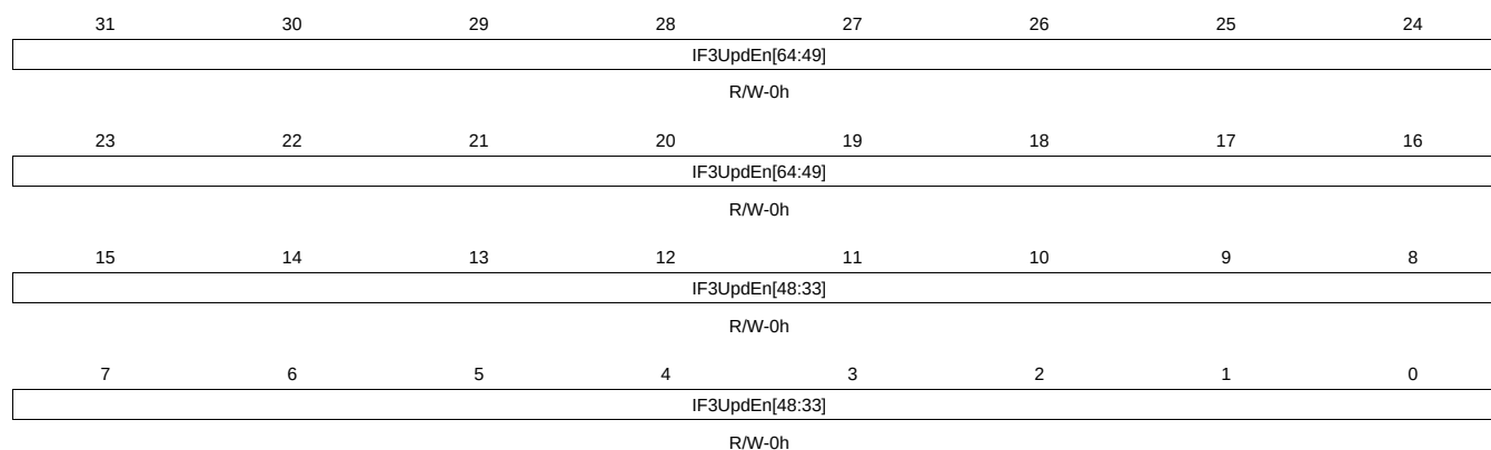
Figure 23-70. IF3UPD34 Register
