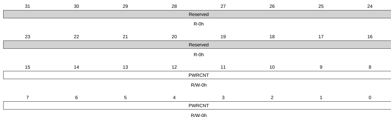
Figure 18-42. SD_PWCNT Register
