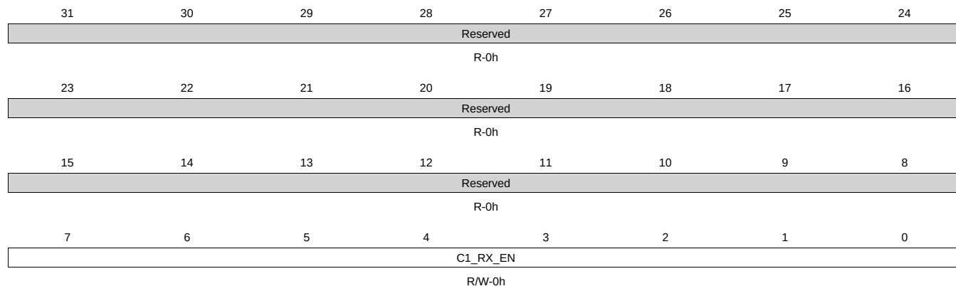
Figure 14-206. C1_RX_EN Register
