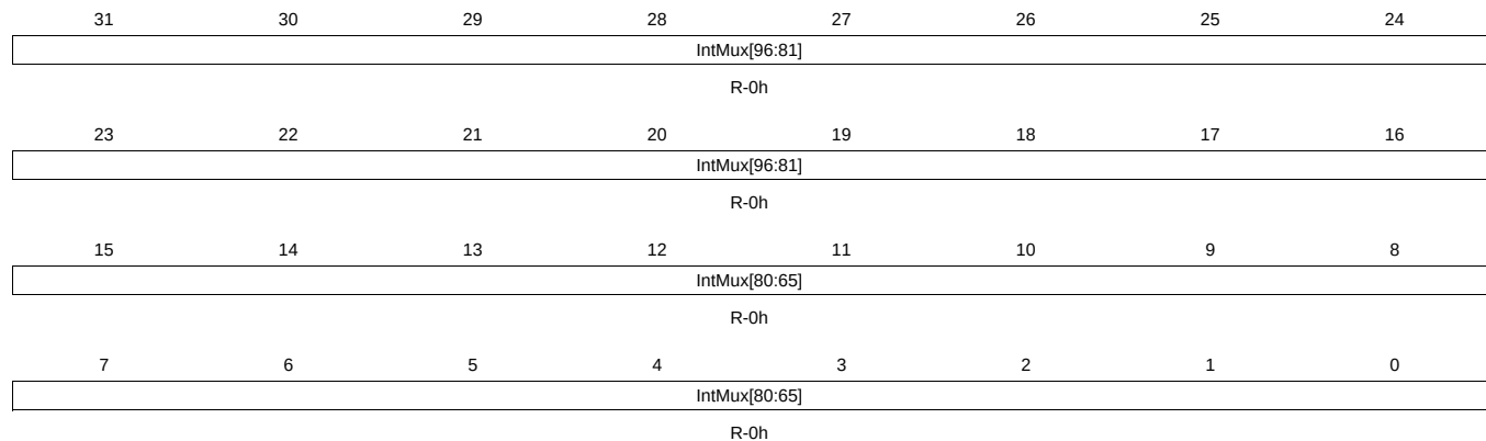
Figure 23-49. INTMUX56 Register
