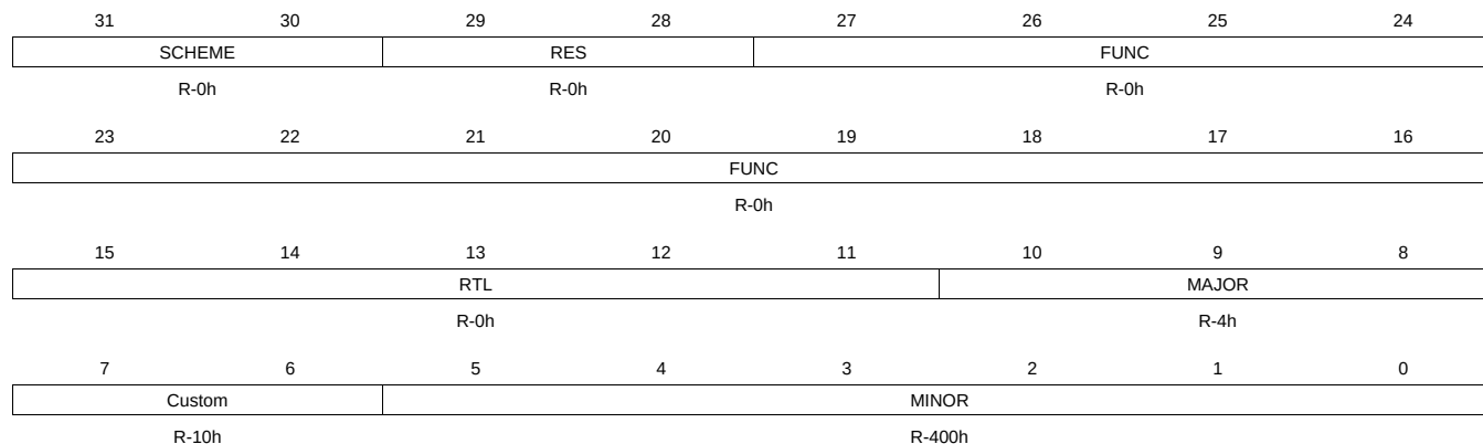
Figure 17-3. REVISION Register
