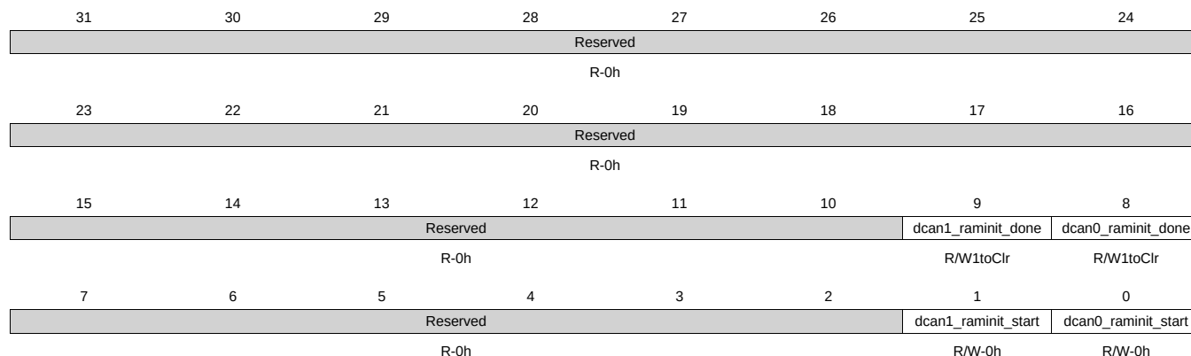
Figure 9-32. dcan_raminit Register
