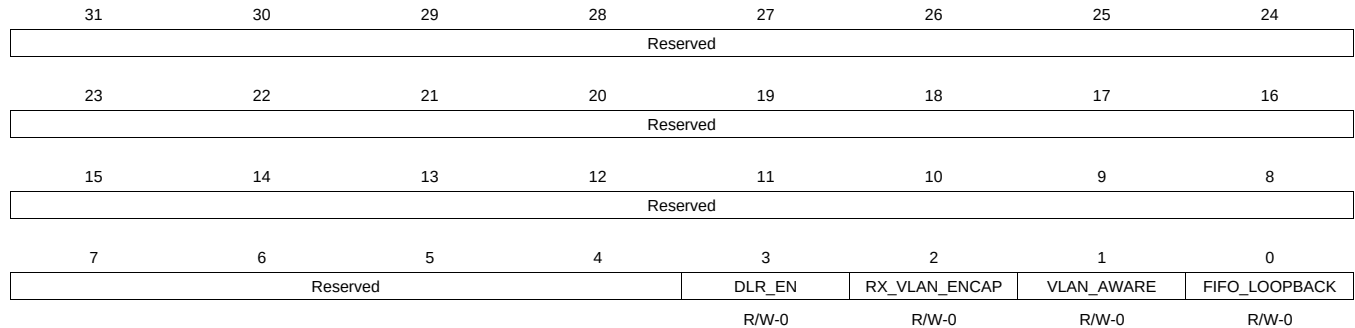
Figure 14-185. CONTROL Register
