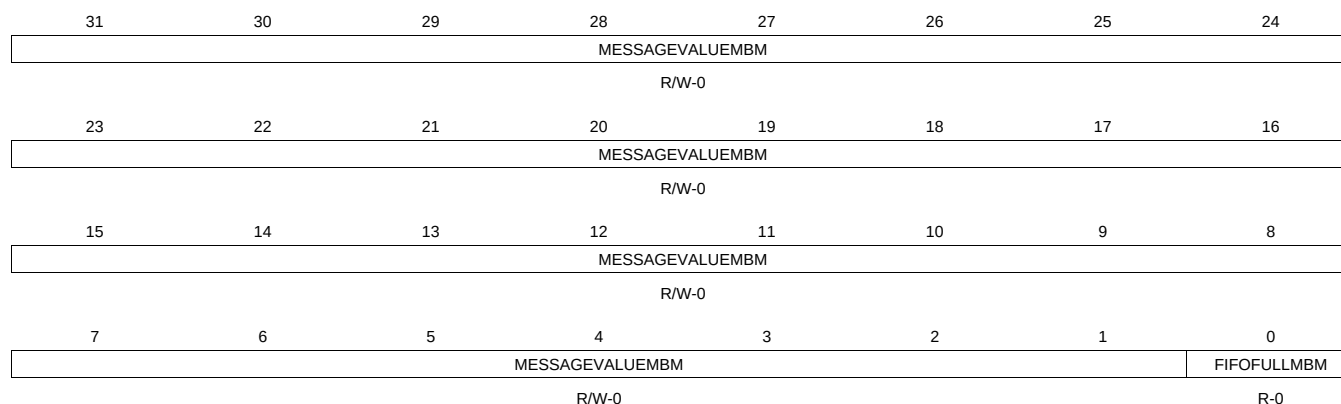
Figure 17-20. FIFOSTATUS_7 Register
