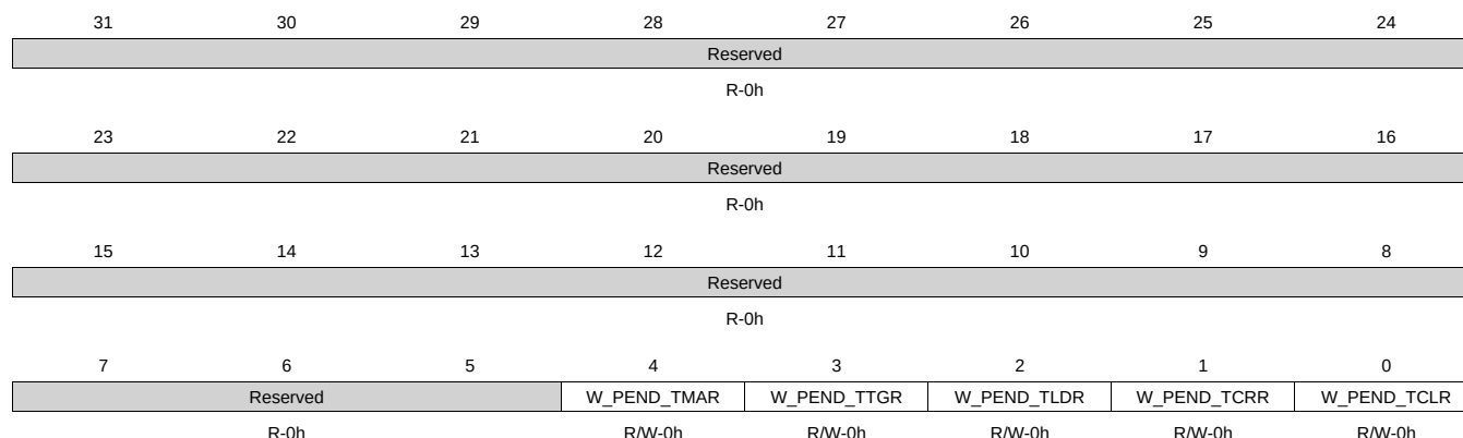
Figure 20-21. TWPS Register
