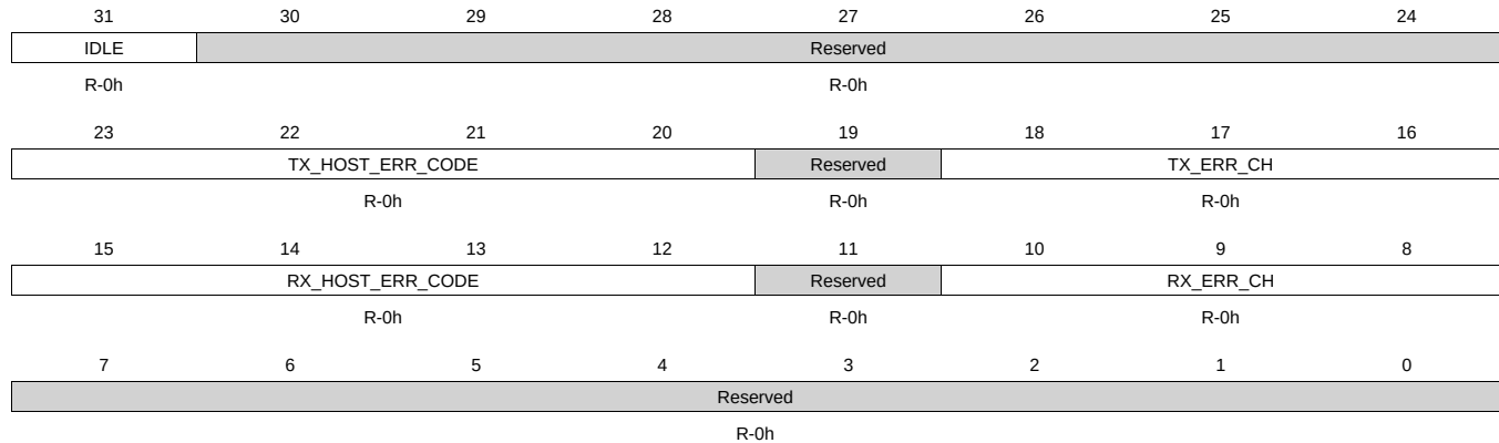
Figure 14-37. DMASTATUS Register
