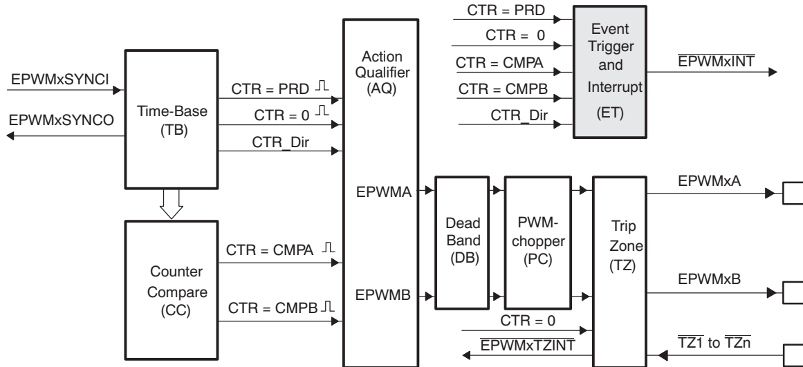
Figure 15-44. Event-Trigger Submodule
