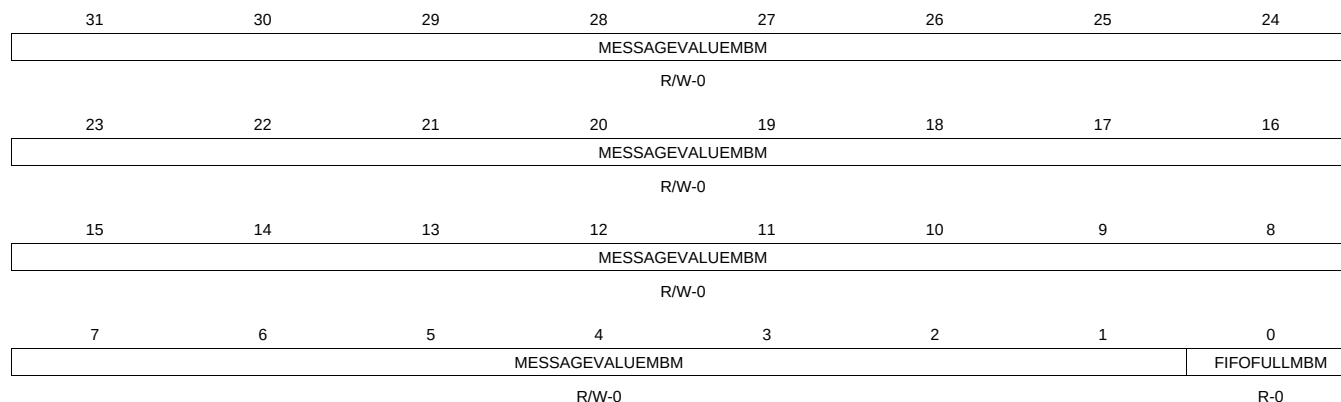
Figure 17-19. FIFOSTATUS_6 Register
