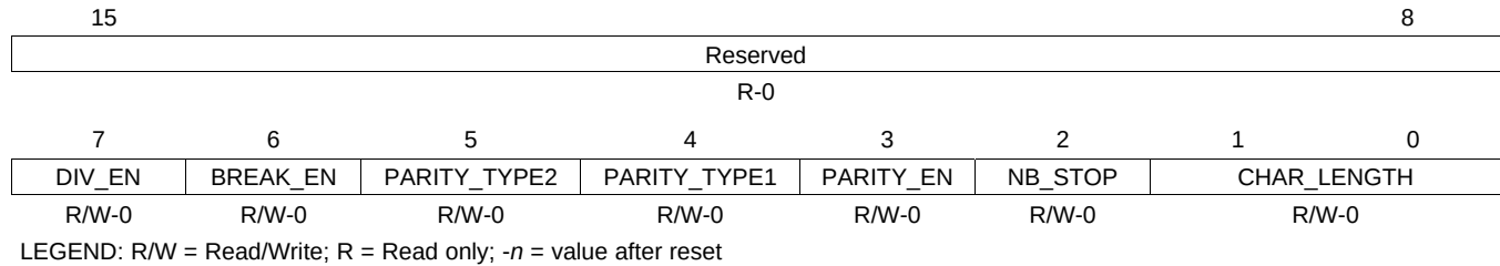
Figure 19-43. Line Control Register (LCR)
