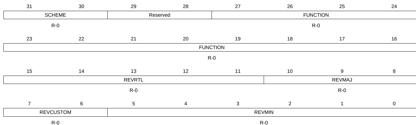
Figure 16-277. QMGRREVID Register
