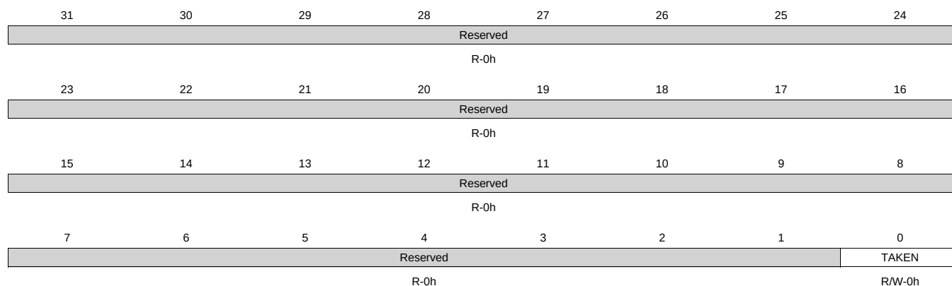
Figure 17-68. LOCK_REG_20 Register
