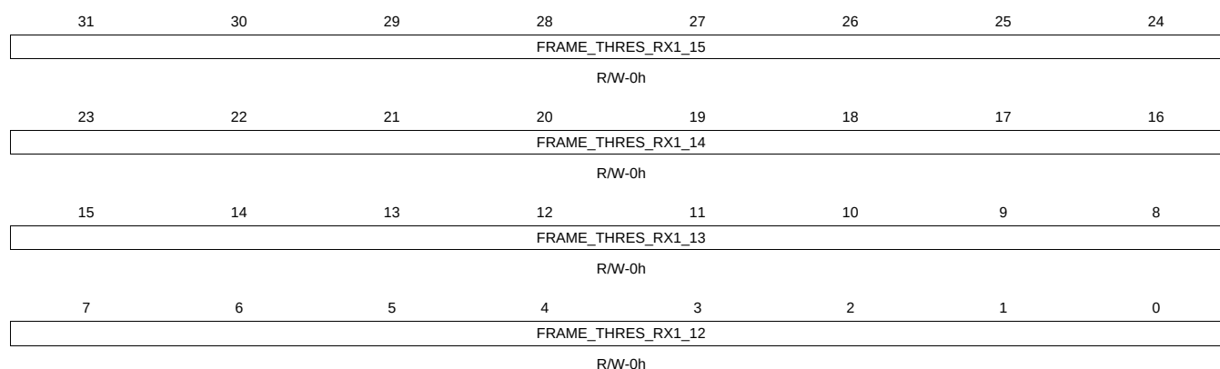
Figure 16-61. IRQFRAMETHOLDRX13 Register
