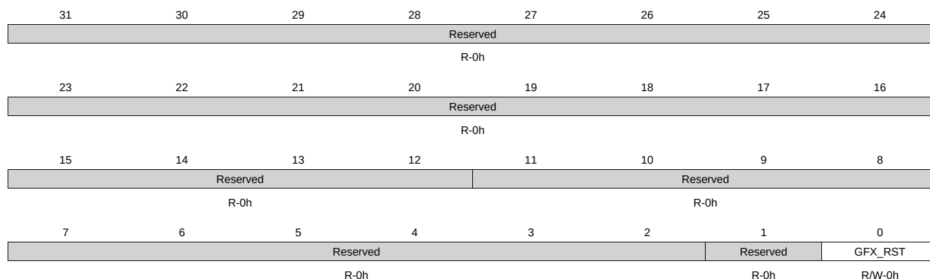
Figure 8-192. RM_GFX_RSTST Register
