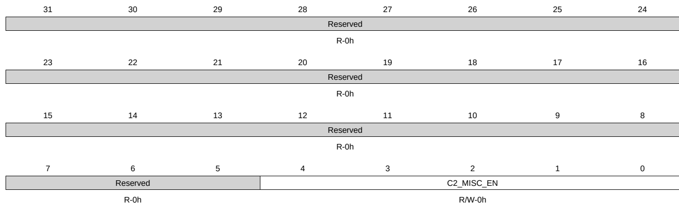
Figure 14-212. C2_MISC_EN Register
