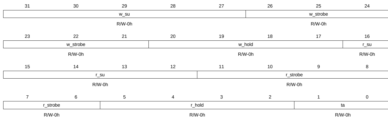
Figure 13-25. LIDD_CS1_CONF Register
