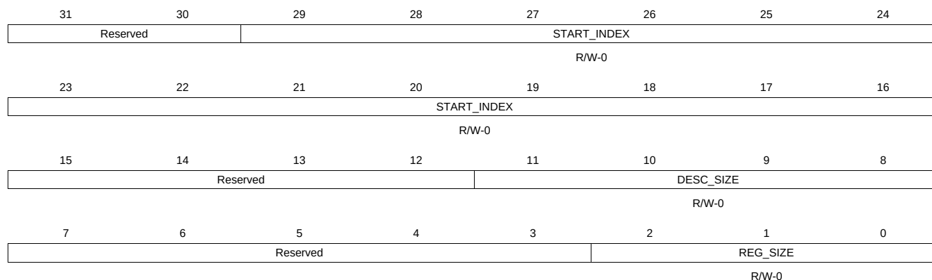
Figure 16-310. QMEMCTRL7 Register
