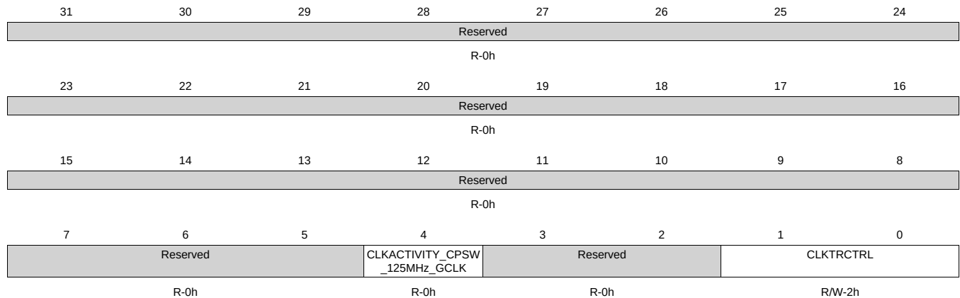
Figure 8-80. CM_PER_CPSW_CLKSTCTRL Register
