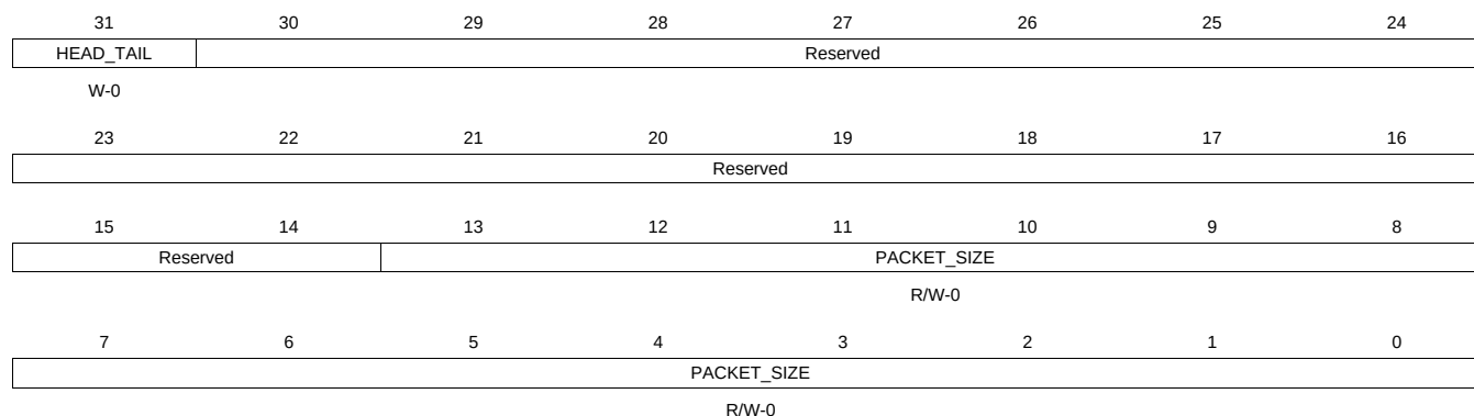
Figure 16-777. QUEUE_116_C Register
