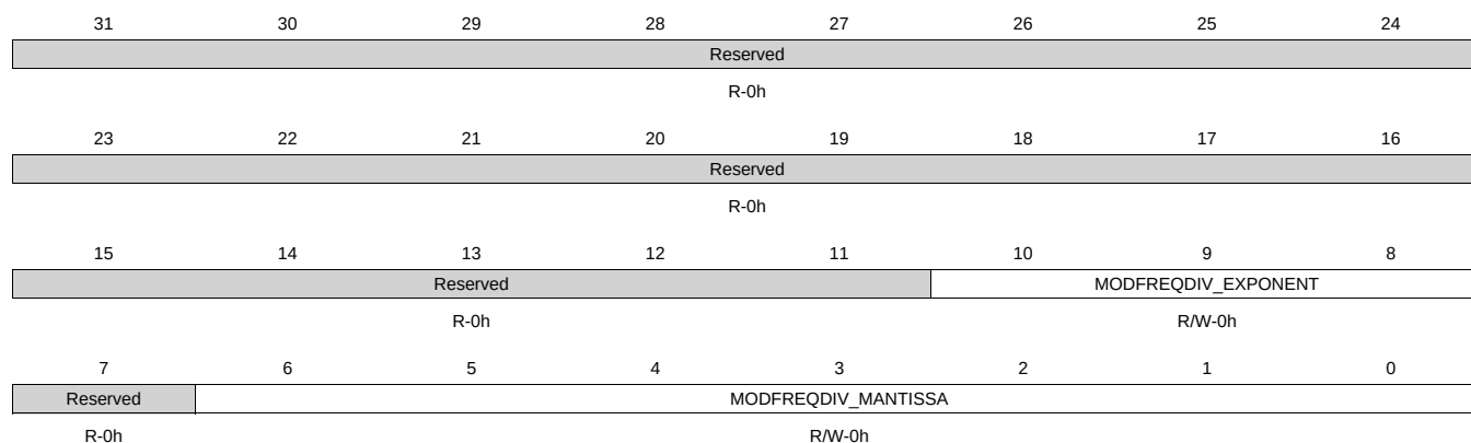
Figure 8-109. CM_SSC_MODFREQDIV_DPLL_CORE Register
