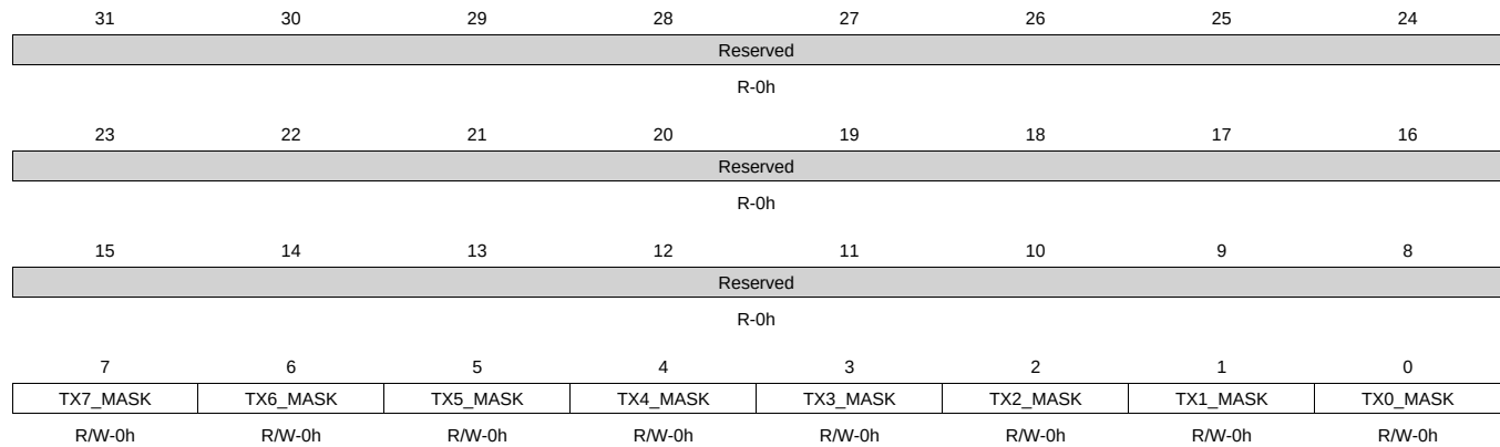
Figure 14-50. TX_INTMASK_SET Register
