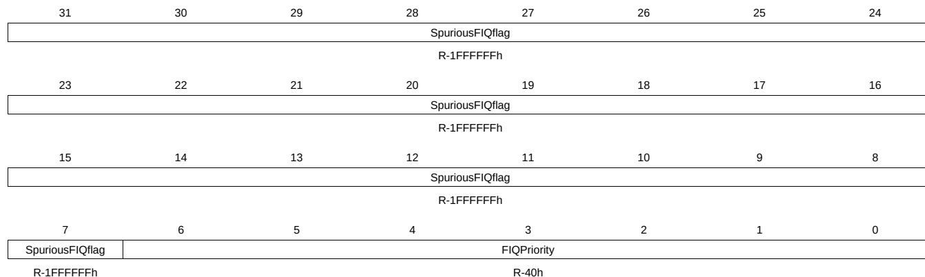
Figure 6-13. INTC_FIQ_PRIORITY Register
