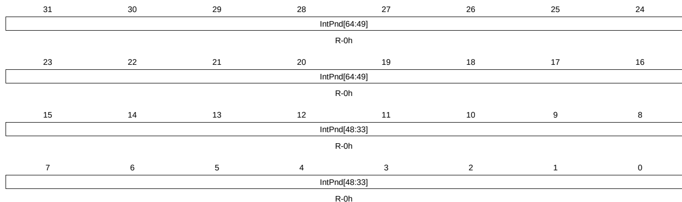
Figure 23-39. INTPND34 Register
