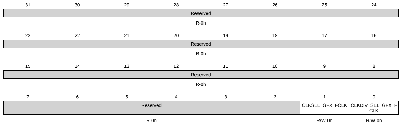
Figure 8-147. CLKSEL_GFX_FCLK Register
