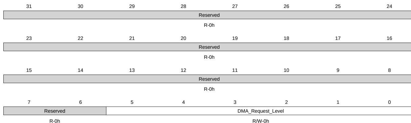
Figure 12-57. DMA0REQ Register
