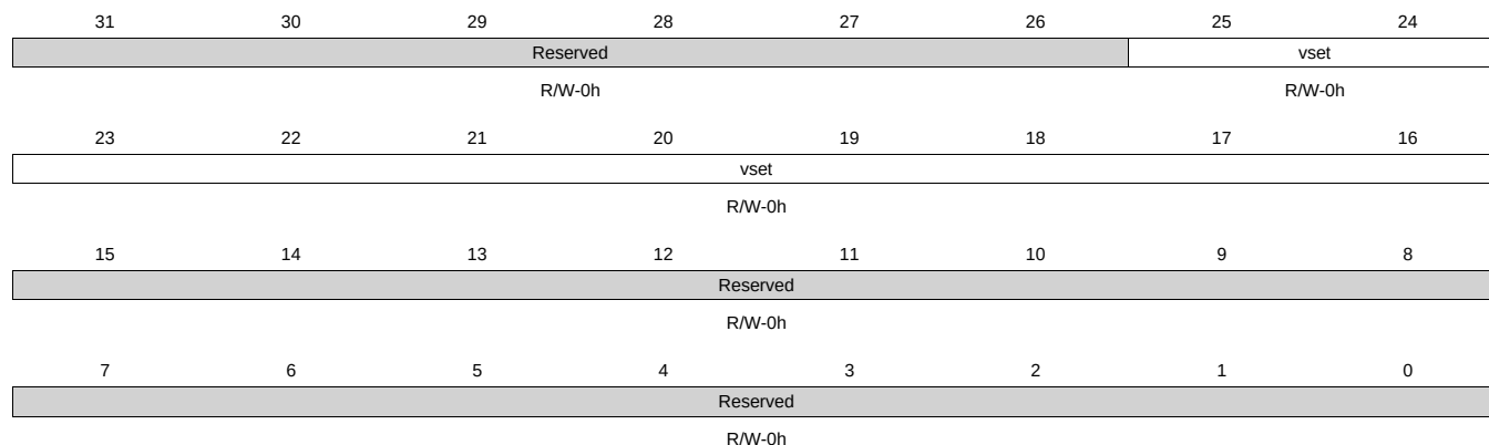
Figure 9-10. mpu_sldo_ctrl Register
