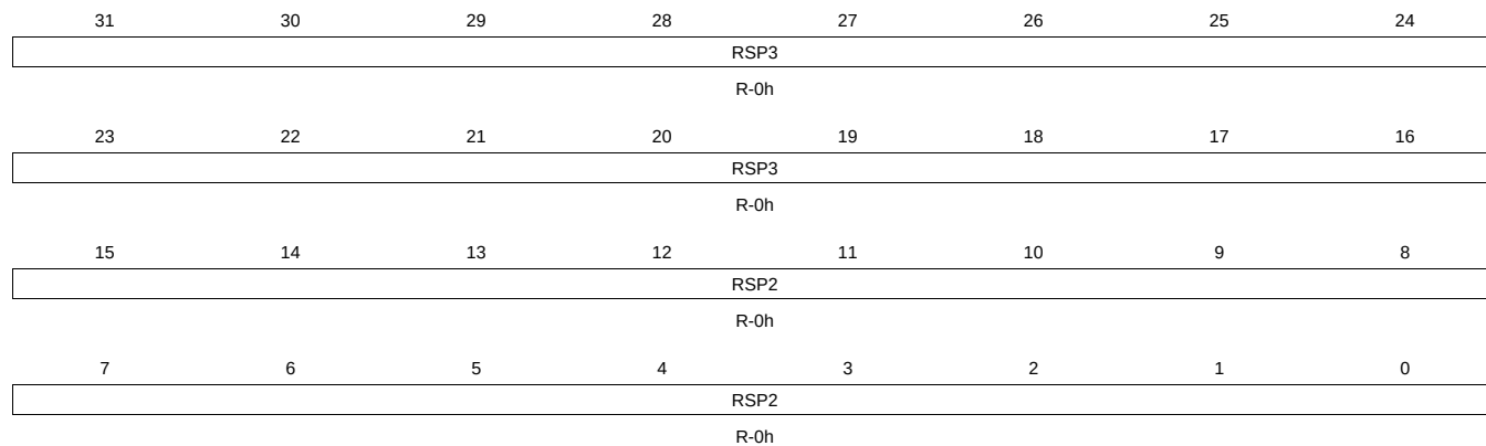
Figure 18-48. SD_RSP32 Register
