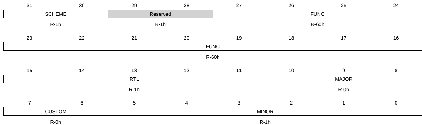
Figure 25-7. GPIO_REVISION Register
