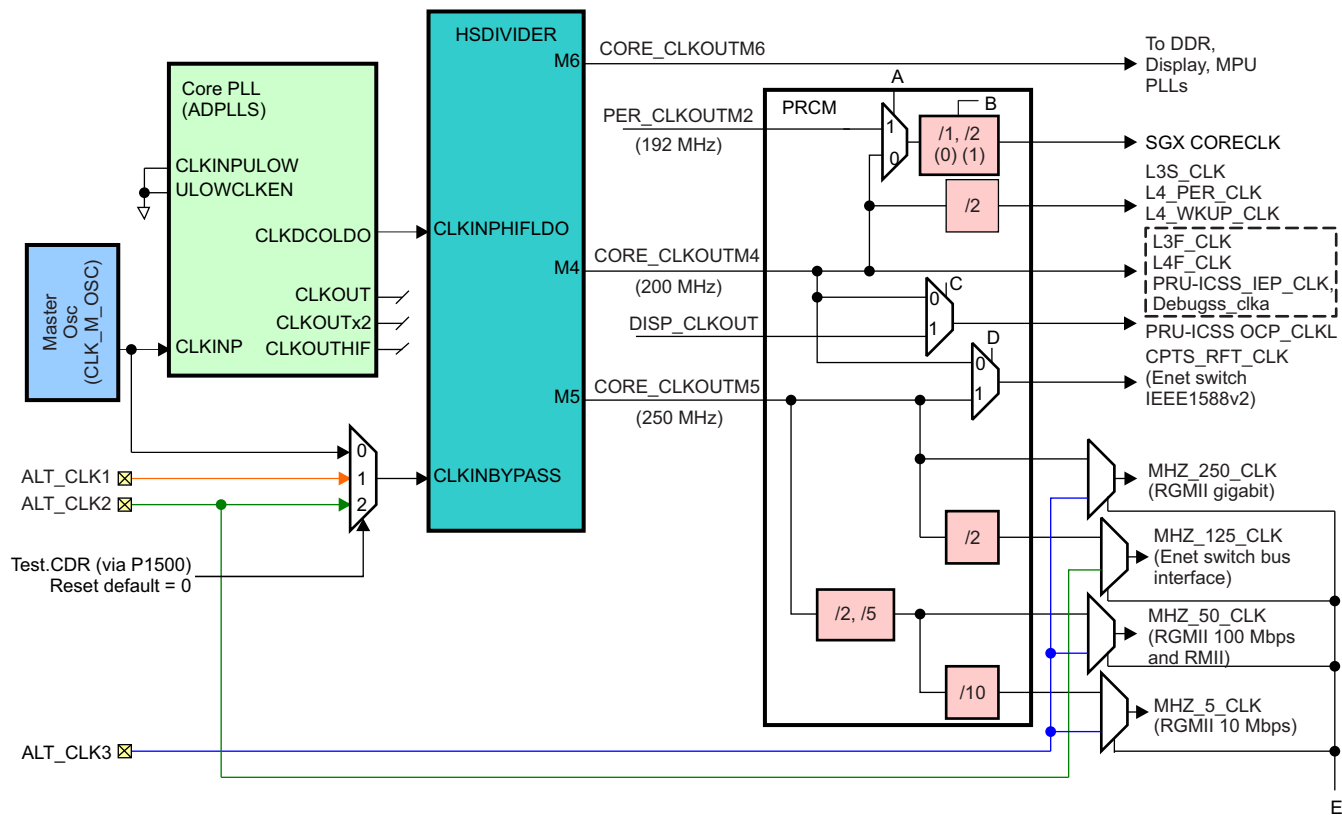
Figure 8-10. Core PLL
