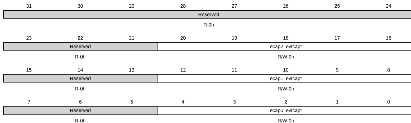
Figure 9-76. ecap_evt_capt Register
