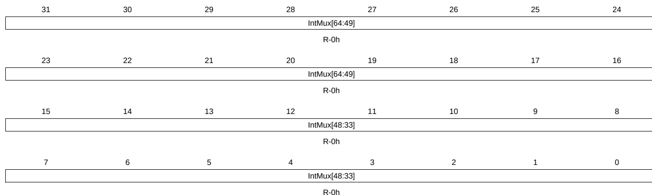
Figure 23-48. INTMUX34 Register
