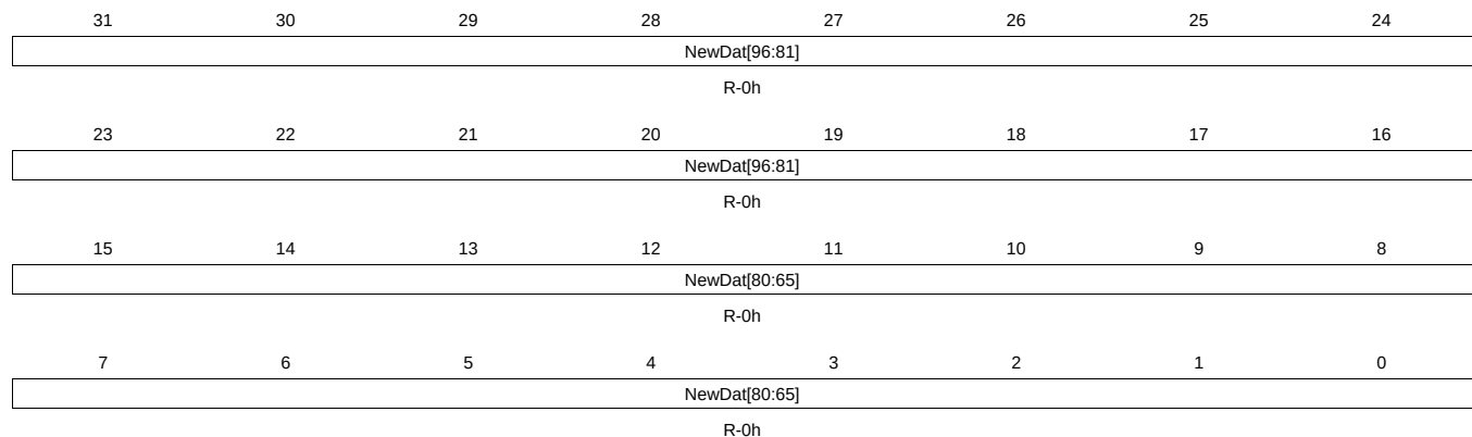
Figure 23-35. NWDAT56 Register
