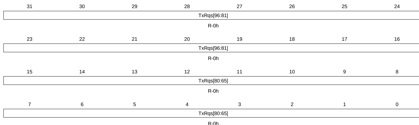
Figure 23-30. TXRQ56 Register
