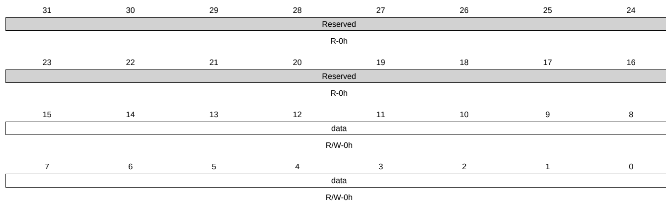
Figure 13-27. LIDD_CS1_DATA Register
