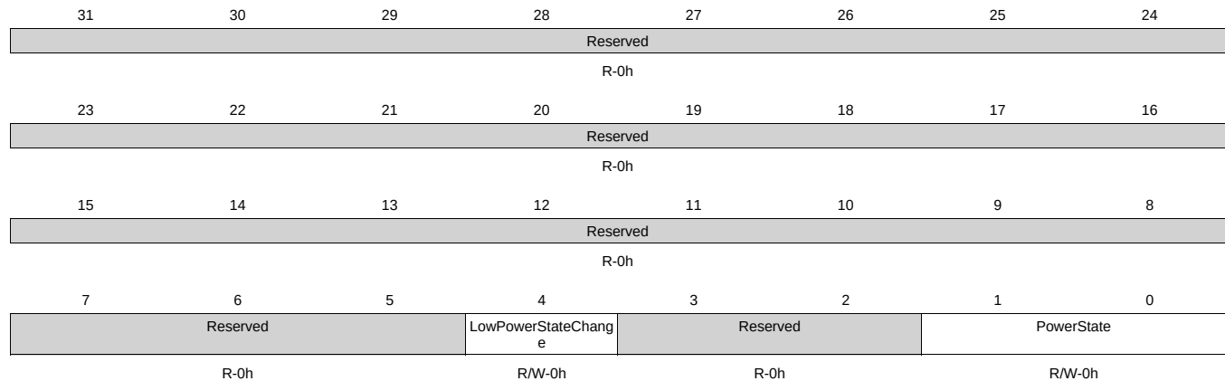
Figure 8-193. PM_CEFUSE_PWRSTCTRL Register
