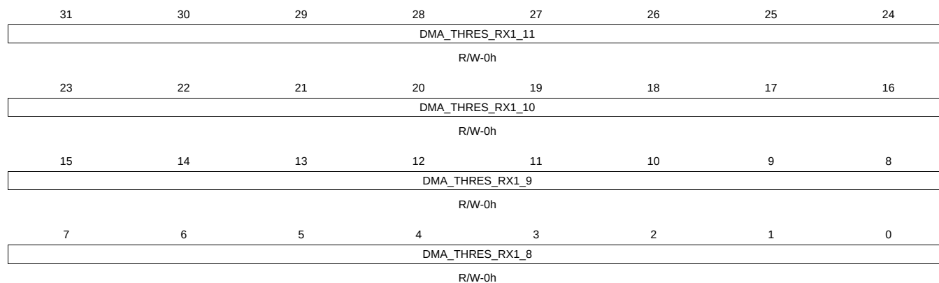
Figure 16-42. IRQDMATHOLDRX12 Register
