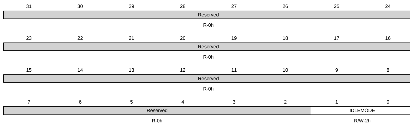
Figure 20-86. RTC_SYSCONFIG Register
