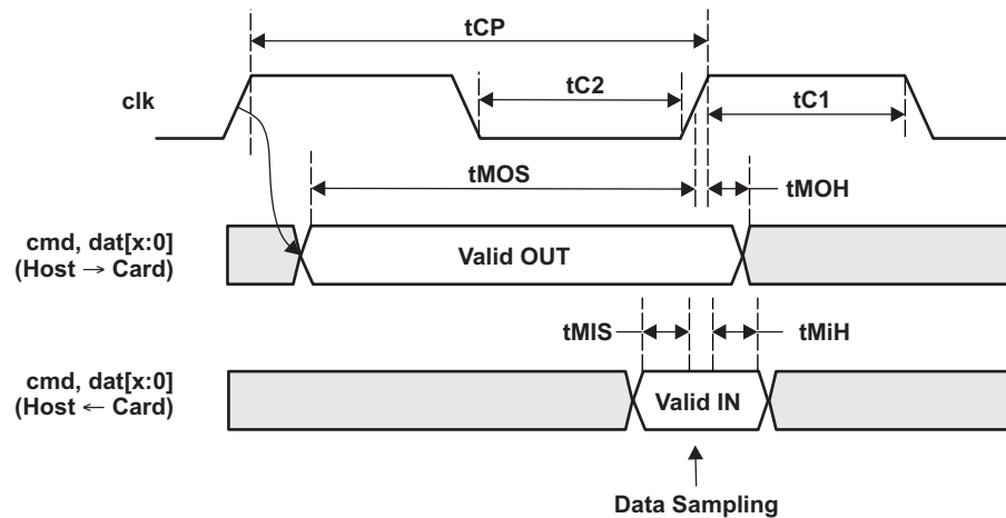
Figure 18-30. Output Driven on Rising Edge
