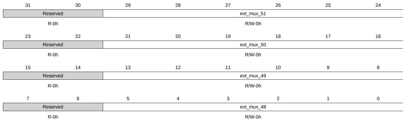
Figure 9-71. tpcc_evt_mux_48_51 Register
