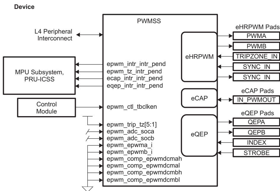
Figure 15-1. PWMSS Integration
