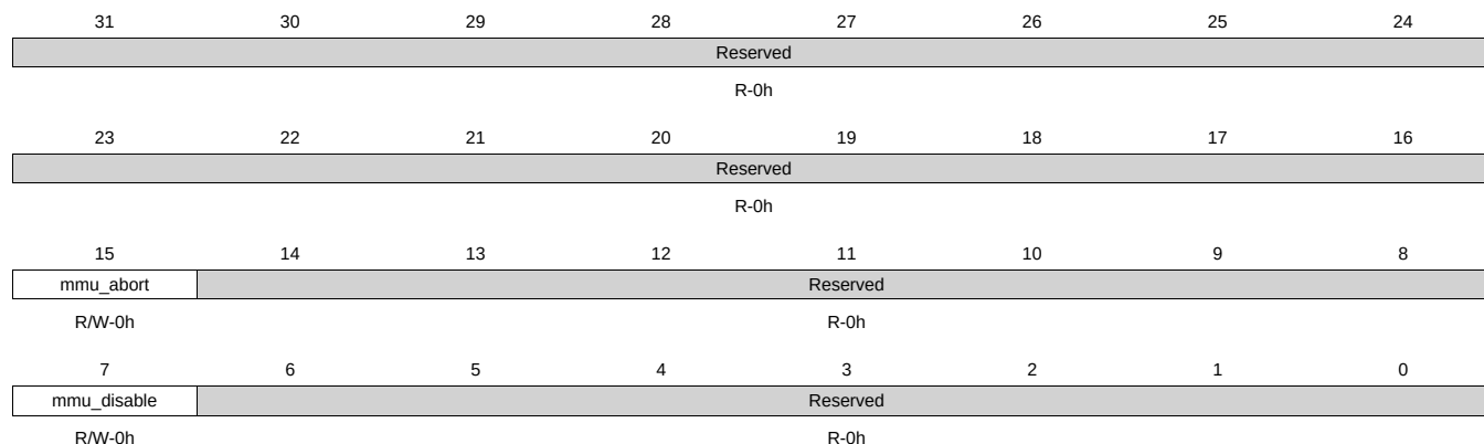
Figure 9-22. mmu_cfg Register
