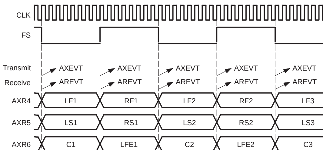
Figure 22-36. DMA Events in an Audio Example—Two Events (Scenario 1)
