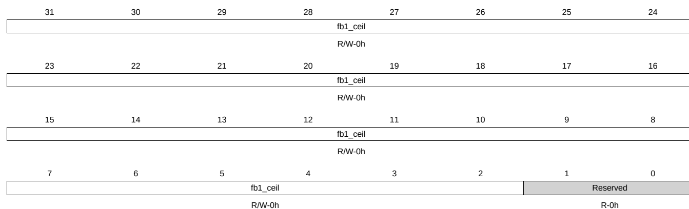
Figure 13-38. LCDDMA_FB1_CEILING Register
