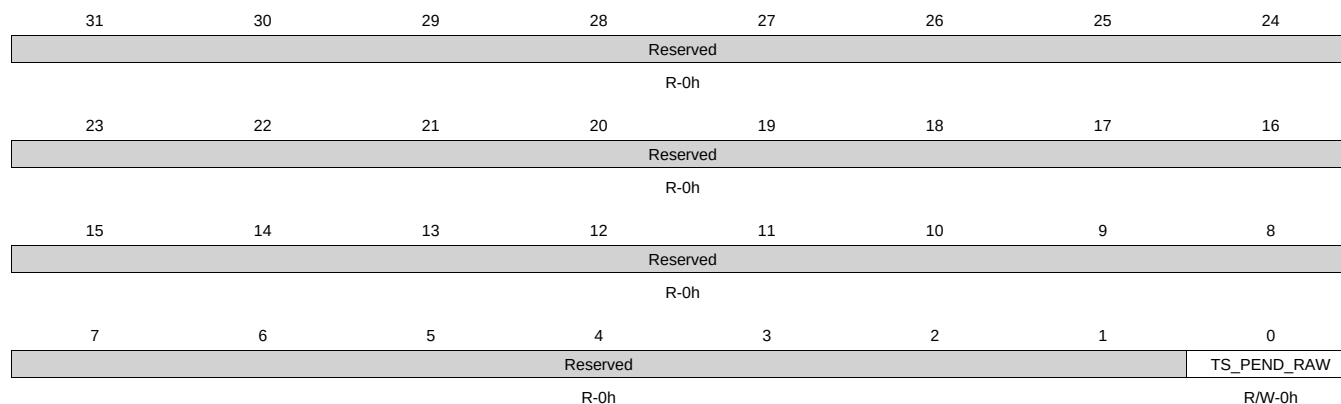
Figure 14-83. CPTS_INTSTAT_RAW Register
