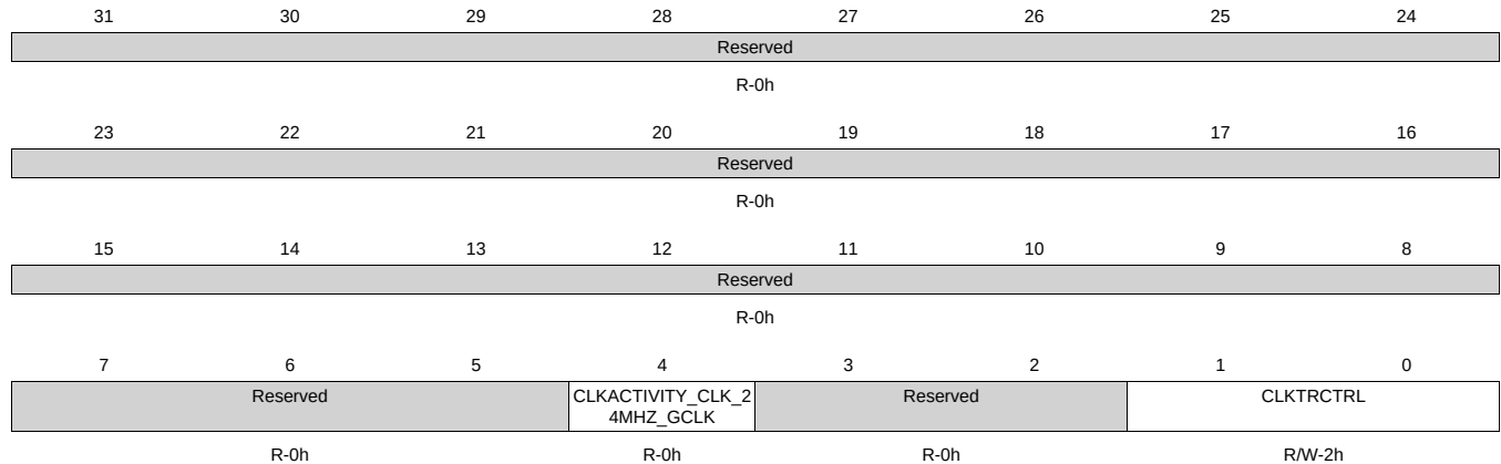
Figure 8-83. CM_PER_CLK_24MHZ_CLKSTCTRL Register
