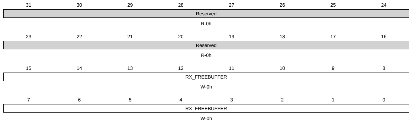
Figure 14-76. RX6_FREEBUFFER Register
