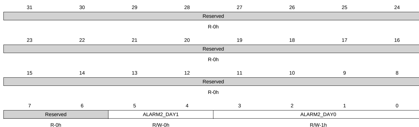
Figure 20-91. ALARM2_DAYS_REG Register
