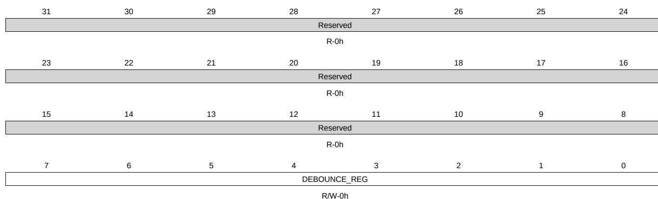
Figure 20-95. RTC_DEBOUNCE Register
