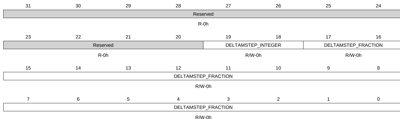
Figure 8-103. CM_SSC_DELTAMSTEP_DPLL_DISP Register
