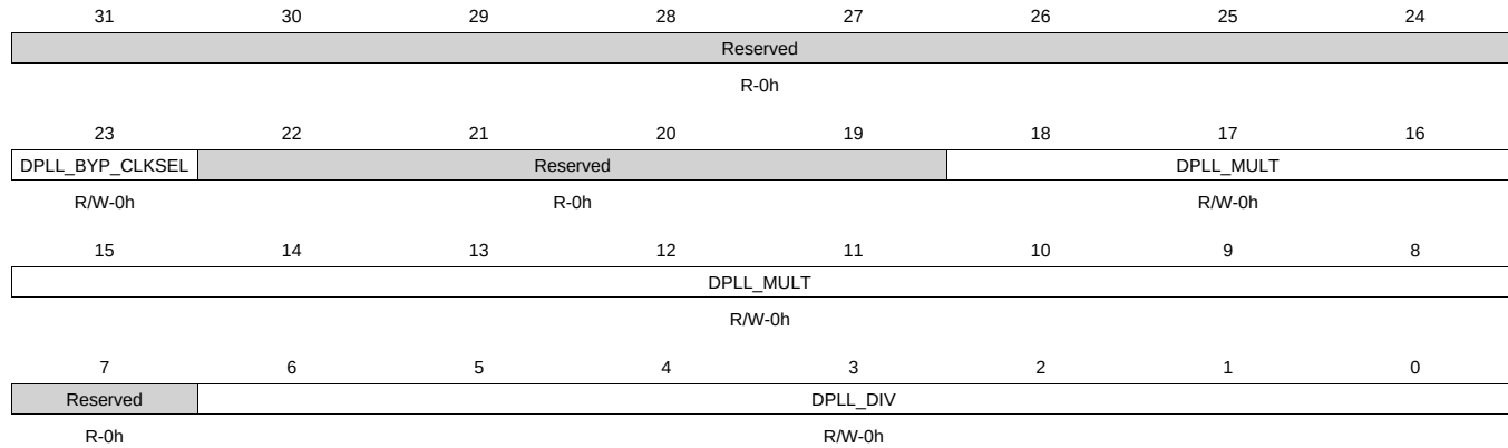
Figure 8-100. CM_CLKSEL_DPLL_DDR Register
