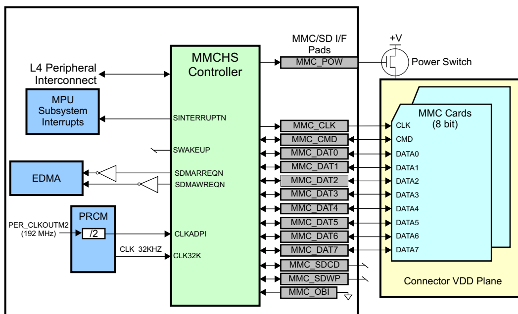
Figure 18-3. MMCHS Module MMC Application
