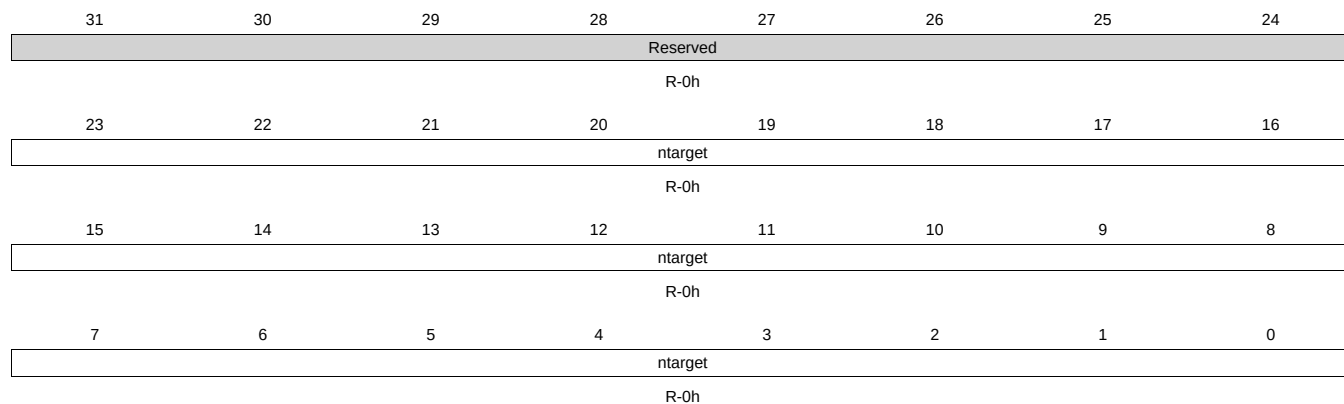
Figure 9-50. vdd_core_opp_100 Register
