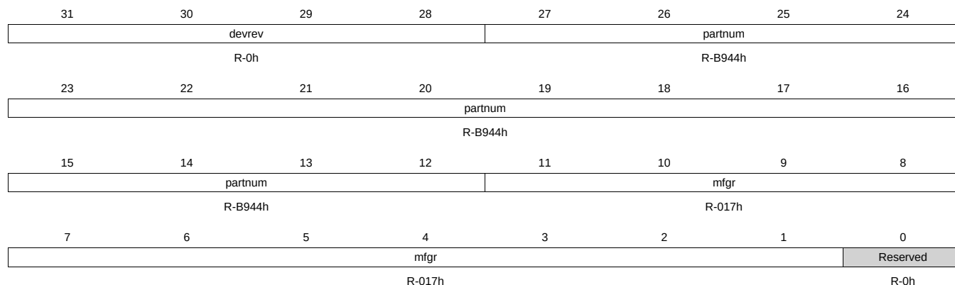
Figure 9-18. device_id Register
