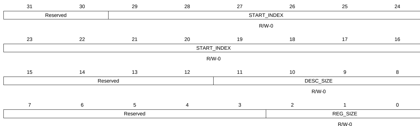
Figure 16-304. QMEMCTRL4 Register
