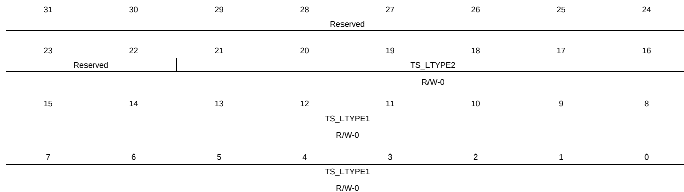
Figure 14-195. TS_LTYPE Register
