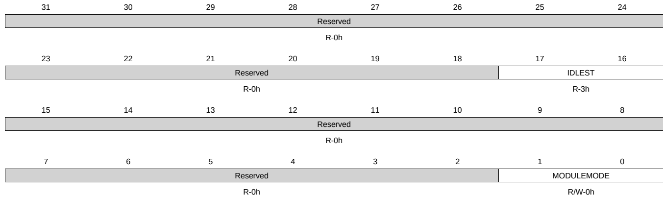
Figure 8-134. CM_WKUP_SMARTREFLEX1_CLKCTRL Register
