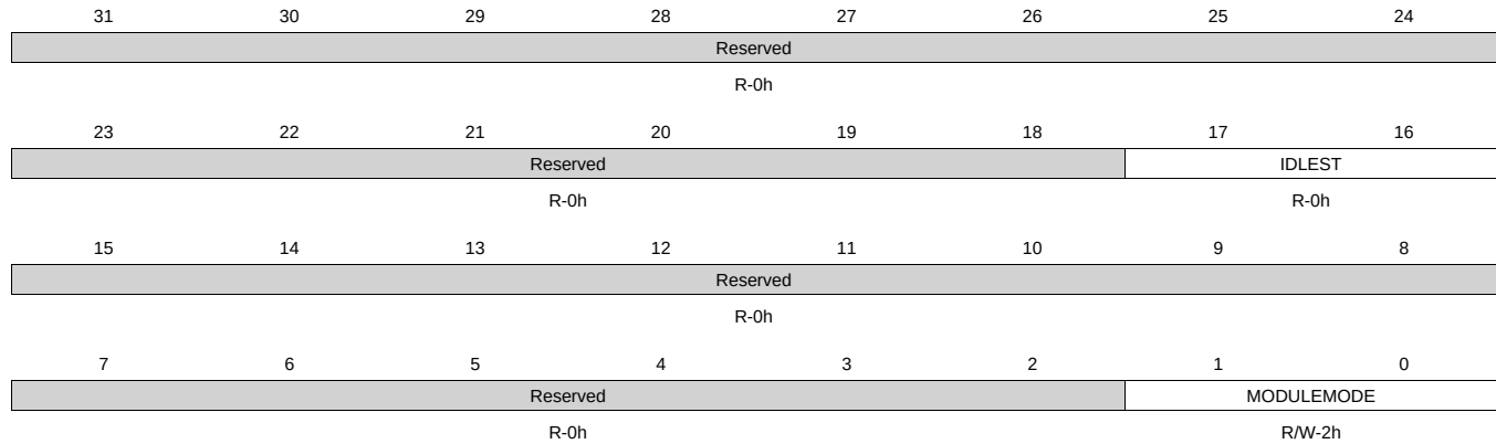
Figure 8-76. CM_PER_L4HS_CLKCTRL Register
