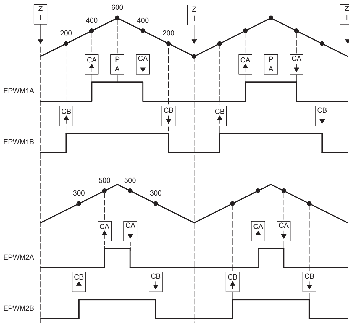
Figure 15-59. Buck Waveforms for Figure 15-58 (Note: F_{PWM2} = F_{PWM1} )
