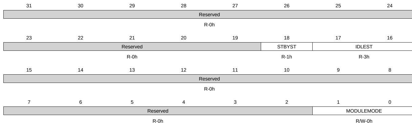
Figure 8-71. CM_PER_TPTC1_CLKCTRL Register
