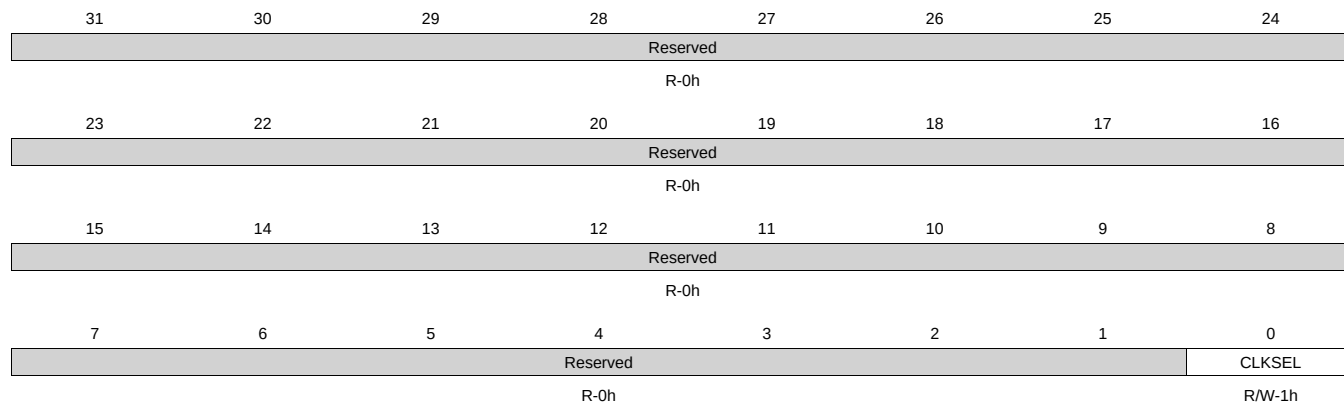
Figure 8-150. CLKSEL_WDT1_CLK Register
