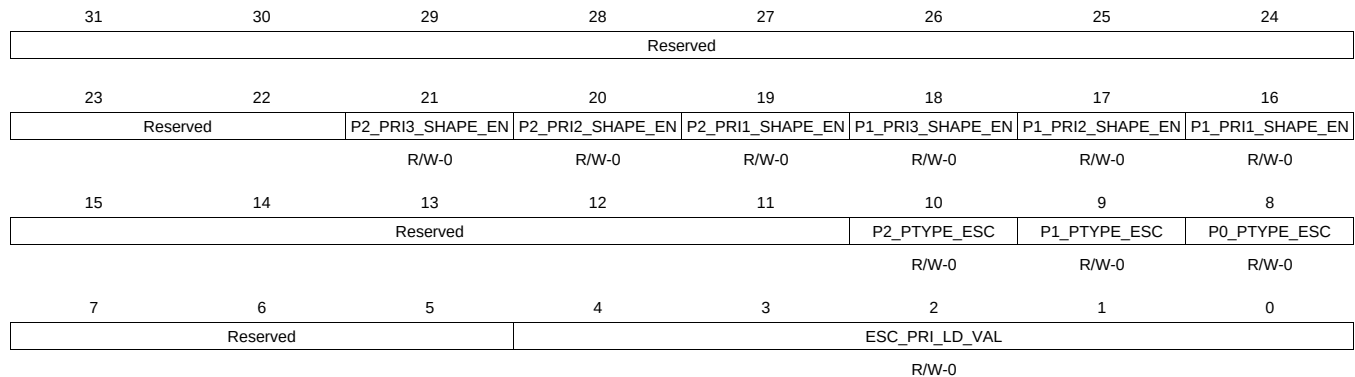
Figure 14-188. PTYPE Register
