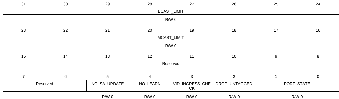
Figure 14-24. PORTCTL1 Register
