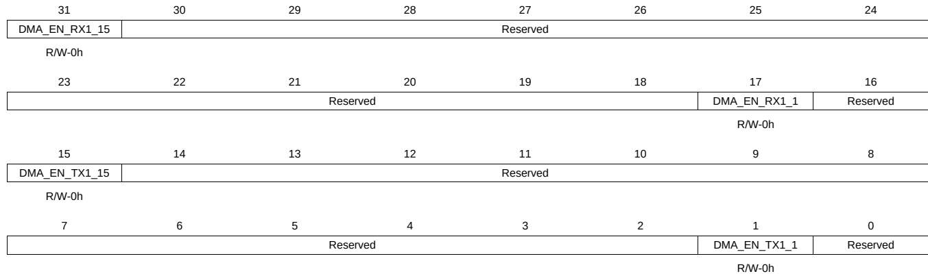
Figure 16-45. IRQDMAENABLE1 Register
