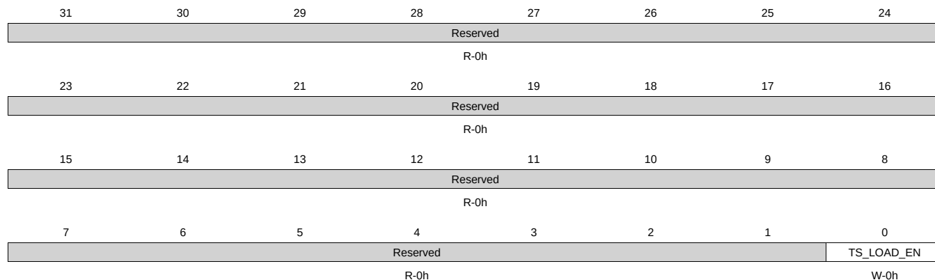
Figure 14-82. CPTS_TS_LOAD_EN Register
