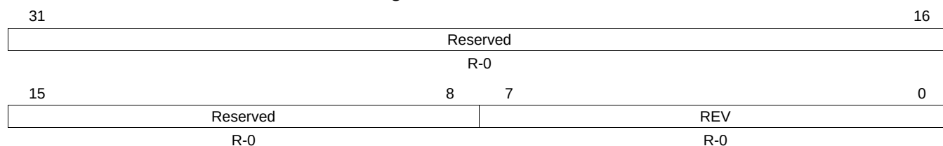
Figure 7-51. GPMC_REVISION
