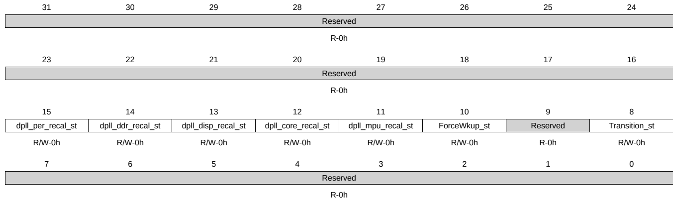
Figure 8-165. PRM_IRQSTATUS_MPU Register
