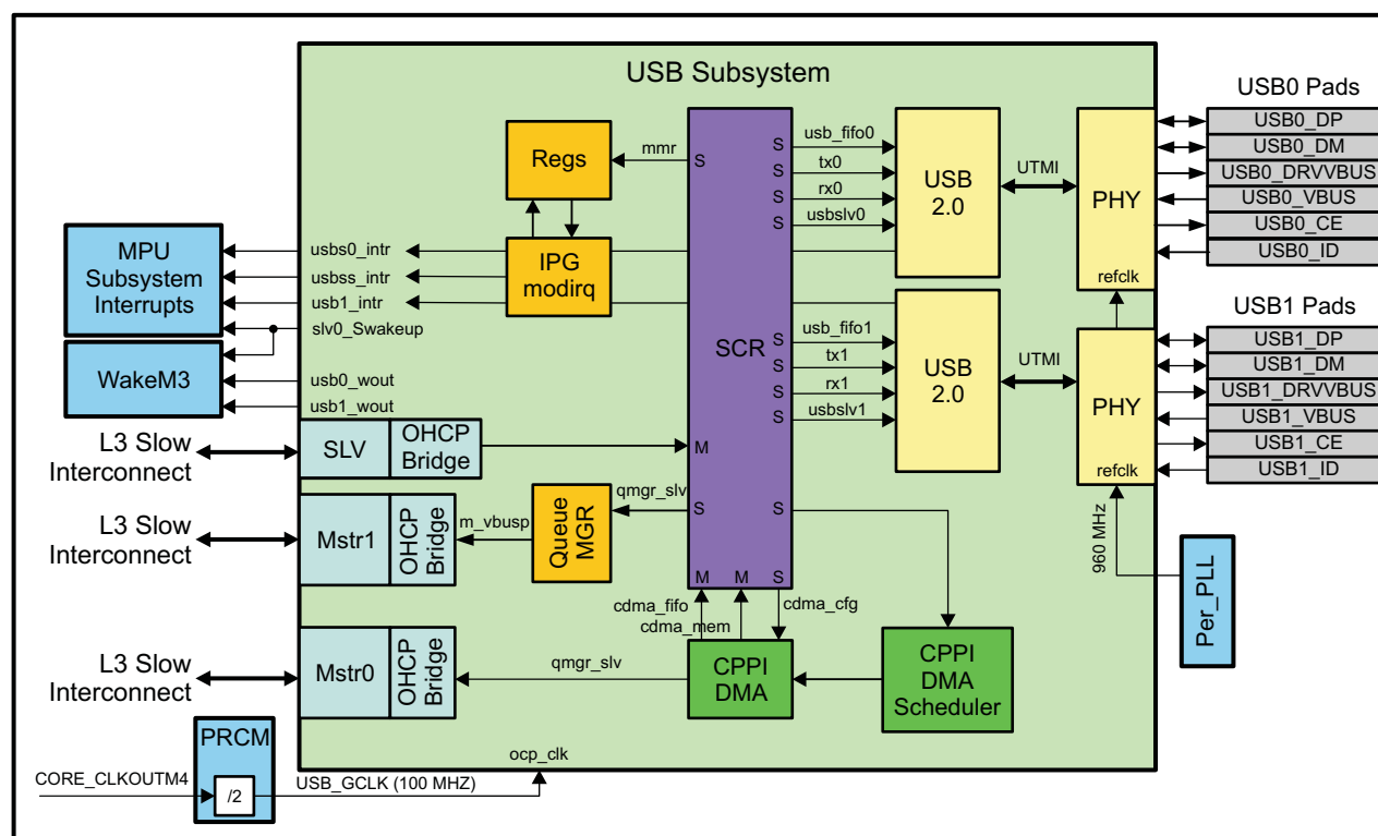
Figure 16-1. USB Integration
