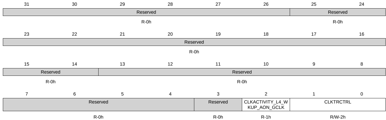
Figure 8-135. CM_L4_WKUP_AON_CLKSTCTRL Register
