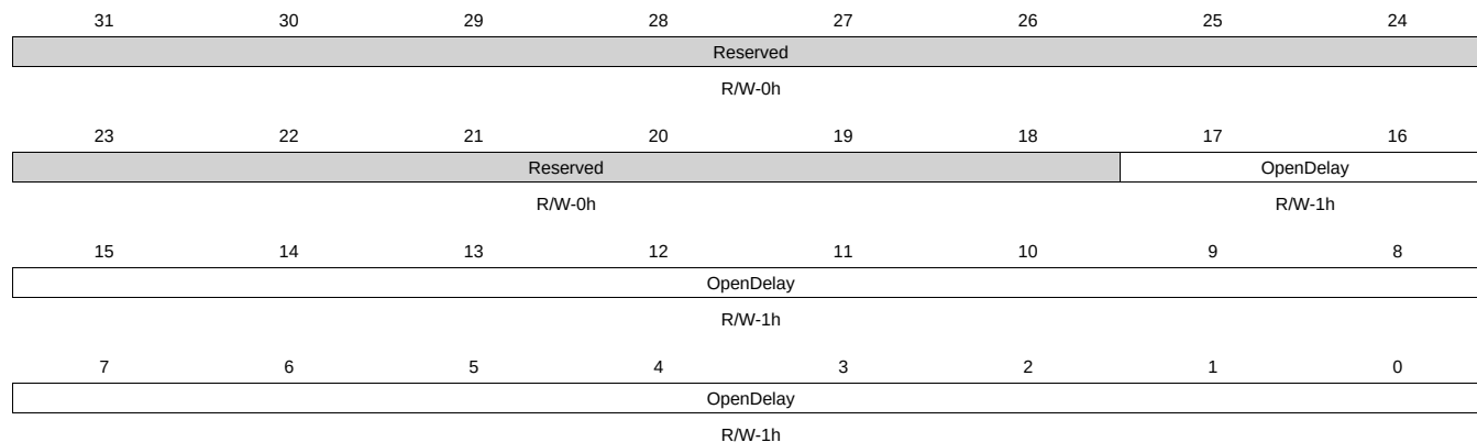
Figure 12-22. TS_CHARGE_DELAY Register
