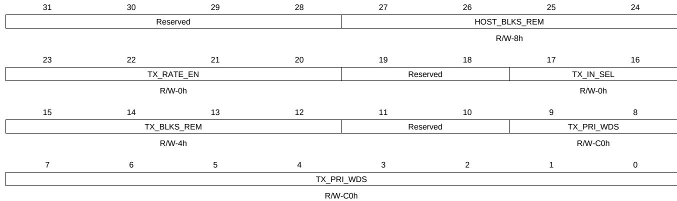
Figure 14-140. P1_TX_IN_CTL Register
