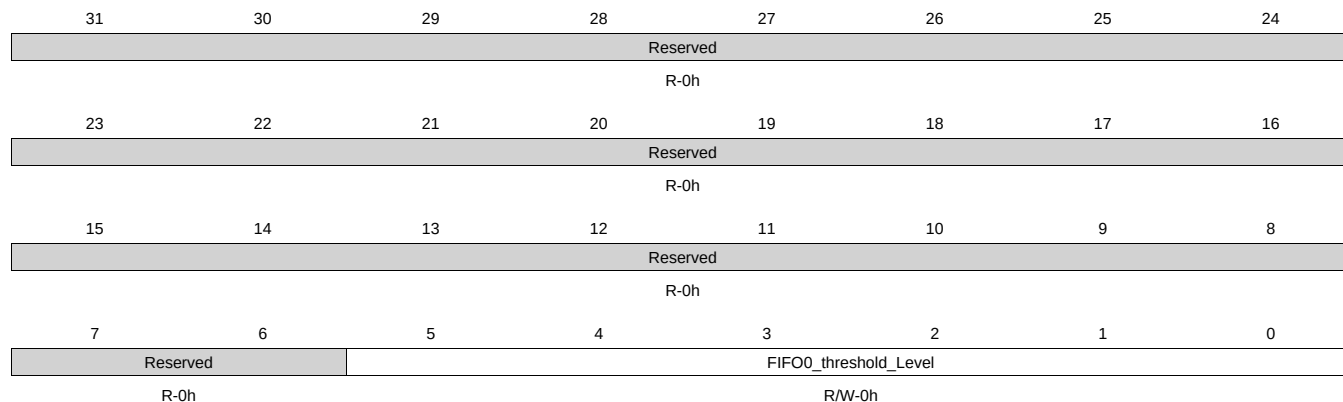
Figure 12-56. FIFO0THRESHOLD Register
