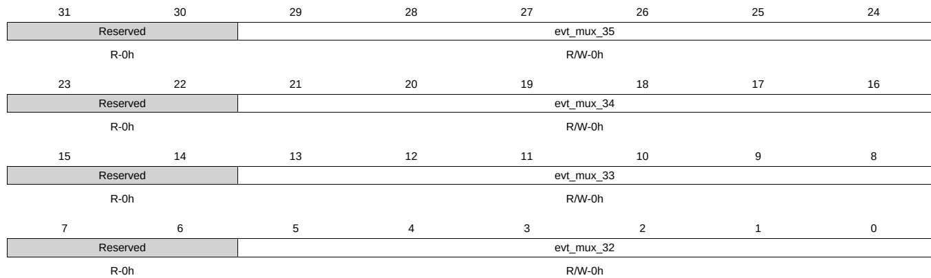
Figure 9-67. tpcc_evt_mux_32_35 Register
