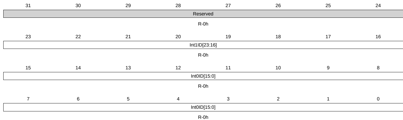
Figure 23-23. INT Register
