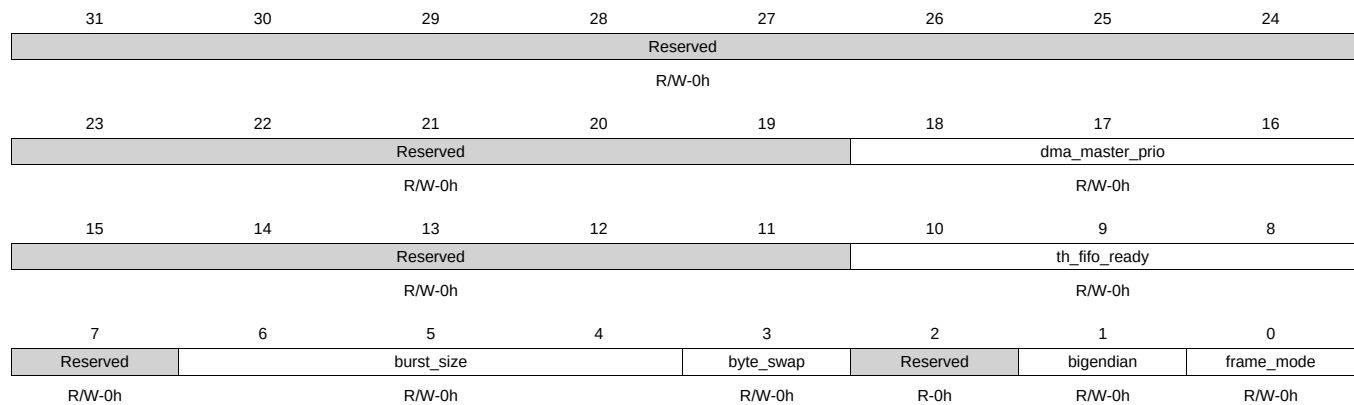
Figure 13-34. LCDDMA_CTRL Register
