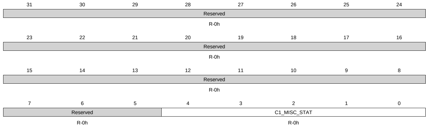
Figure 14-220. C1_MISC_STAT Register
