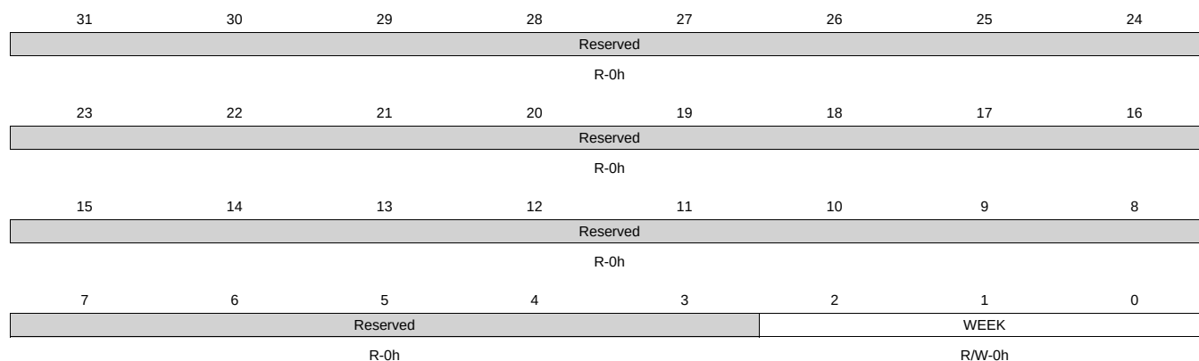
Figure 20-67. WEEKS_REG Register
