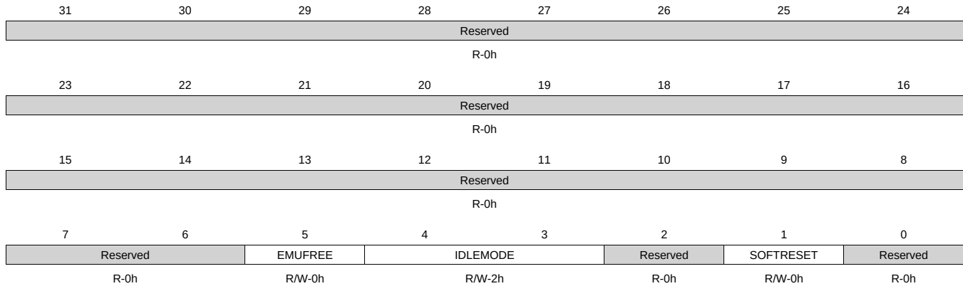
Figure 20-100. WDT_WDSC Register
