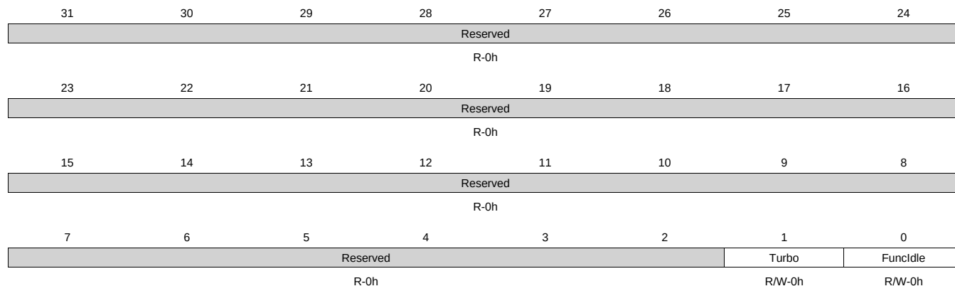
Figure 6-11. INTC_IDLE Register
