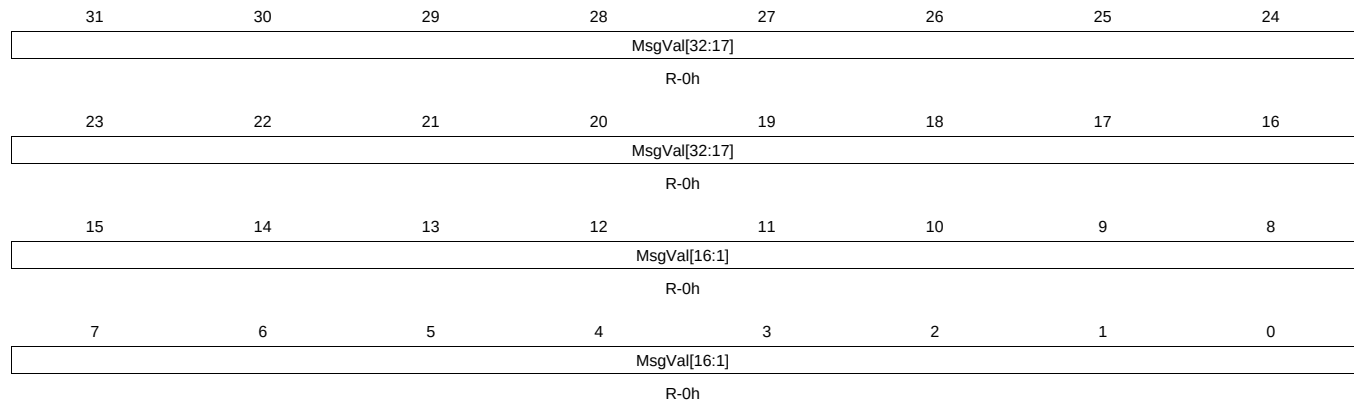
Figure 23-43. MSGVAL12 Register
