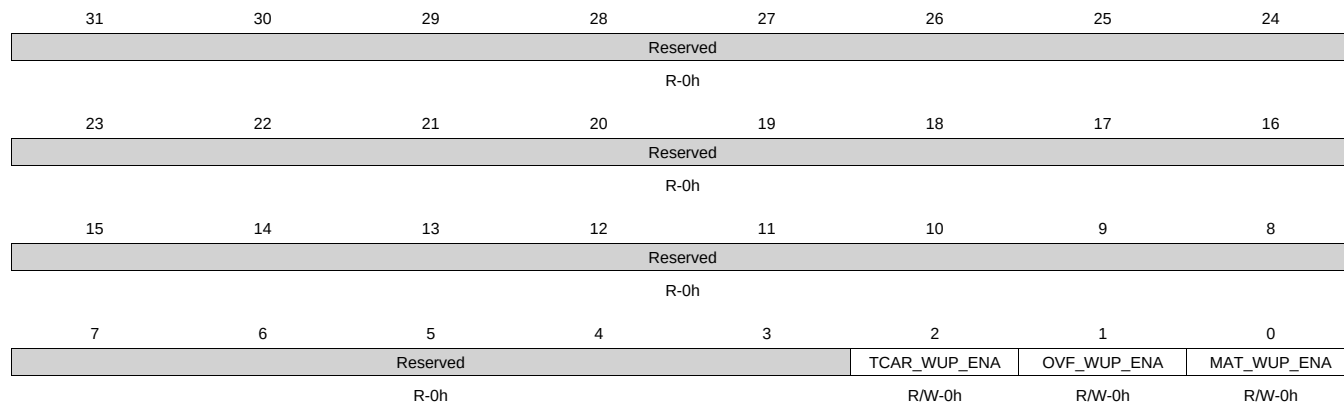
Figure 20-40. TWER Register
