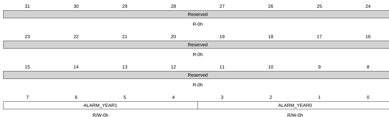
Figure 20-73. ALARM_YEARS_REG Register
