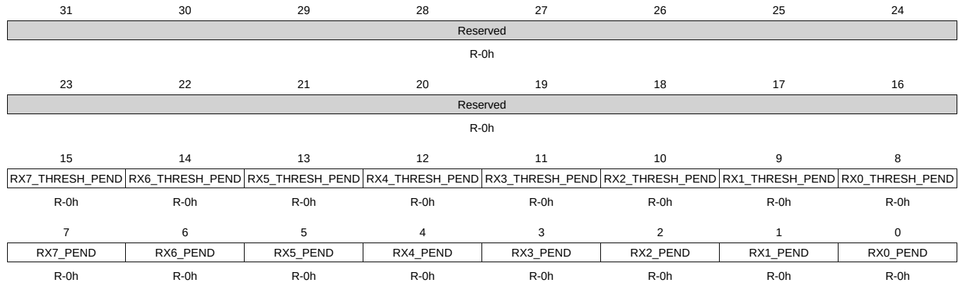
Figure 14-54. RX_INTSTAT_RAW Register
