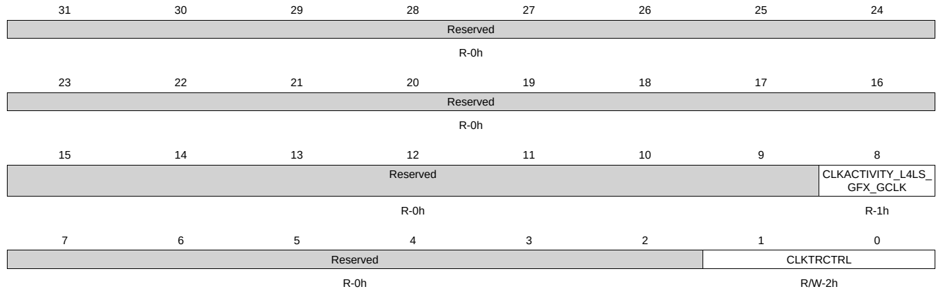
Figure 8-159. CM_GFX_L4LS_GFX_CLKSTCTRL Register
