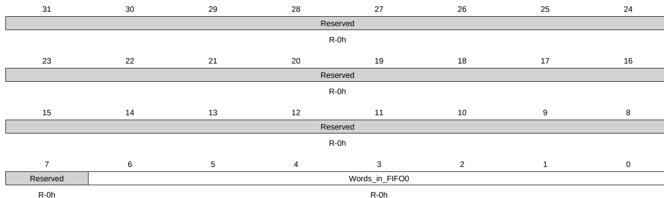
Figure 12-58. FIFO1COUNT Register
