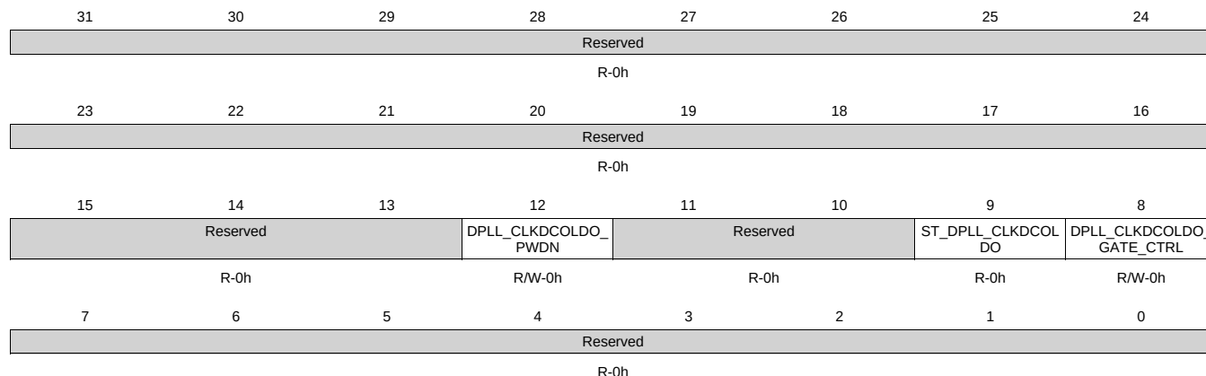
Figure 8-115. CM_CLKDCOLDO_DPLL_PER Register
