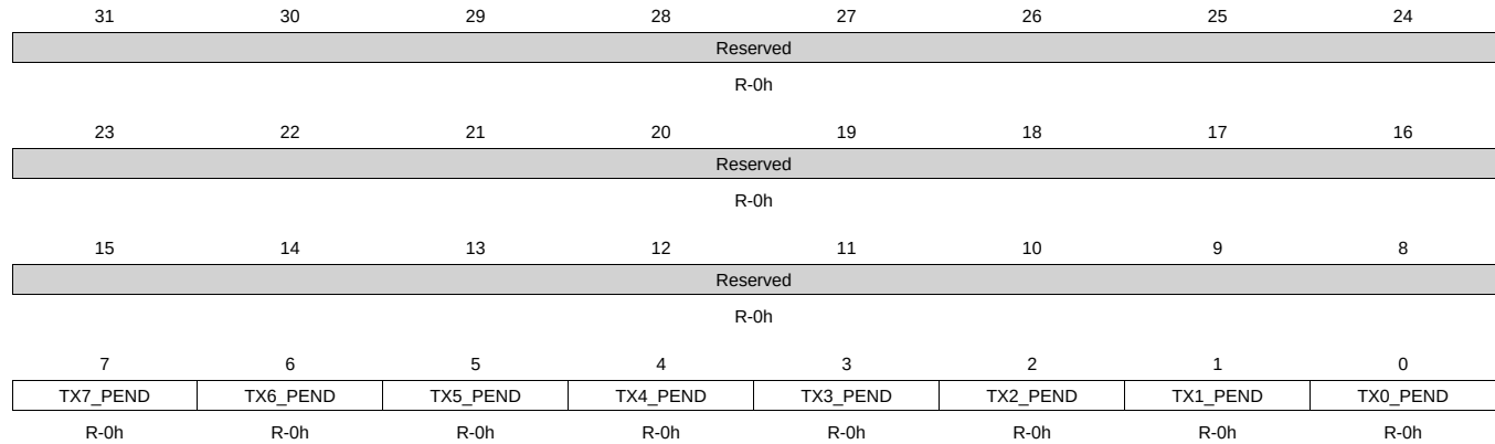
Figure 14-48. TX_INTSTAT_RAW Register
