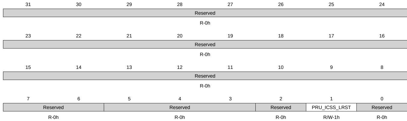
Figure 8-169. RM_PER_RSTCTRL Register
