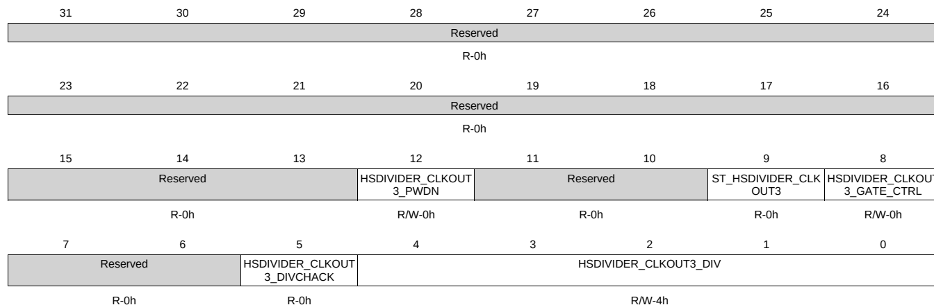
Figure 8-137. CM_DIV_M6_DPLL_CORE Register
