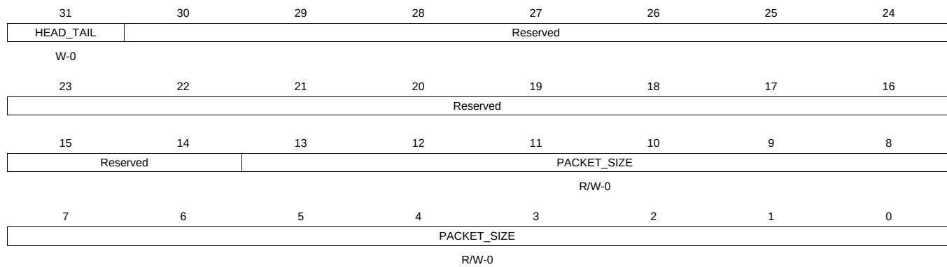
Figure 16-621. QUEUE_77_C Register
