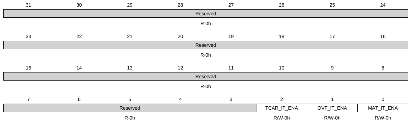
Figure 20-39. TIER Register
