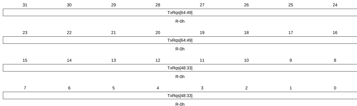
Figure 23-29. TXRQ34 Register
