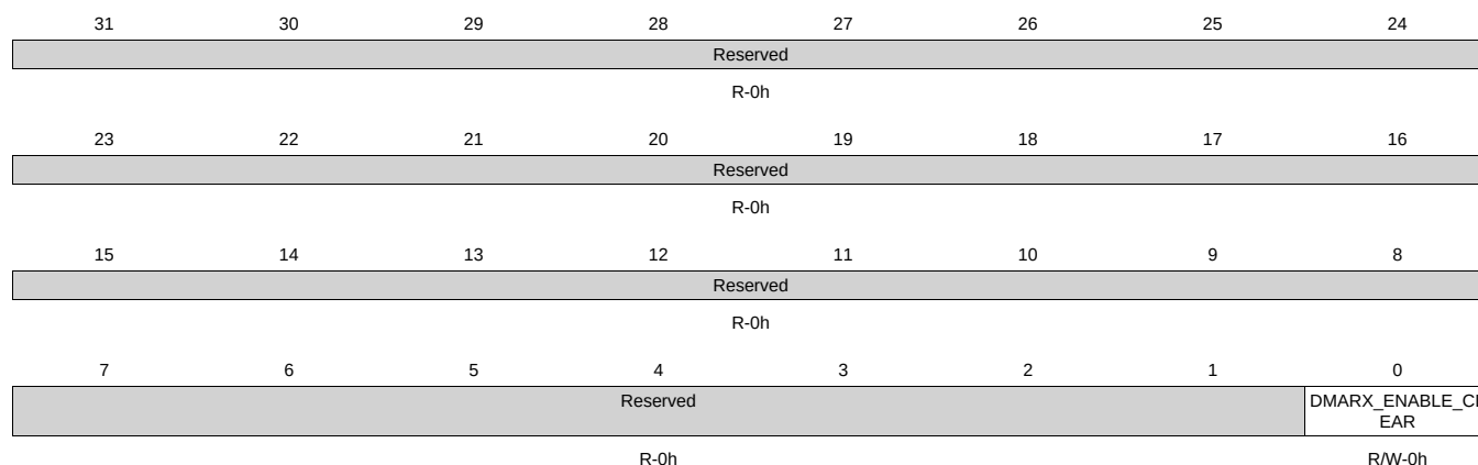
Figure 21-26. I2C_DMARXENABLE_CLR Register
