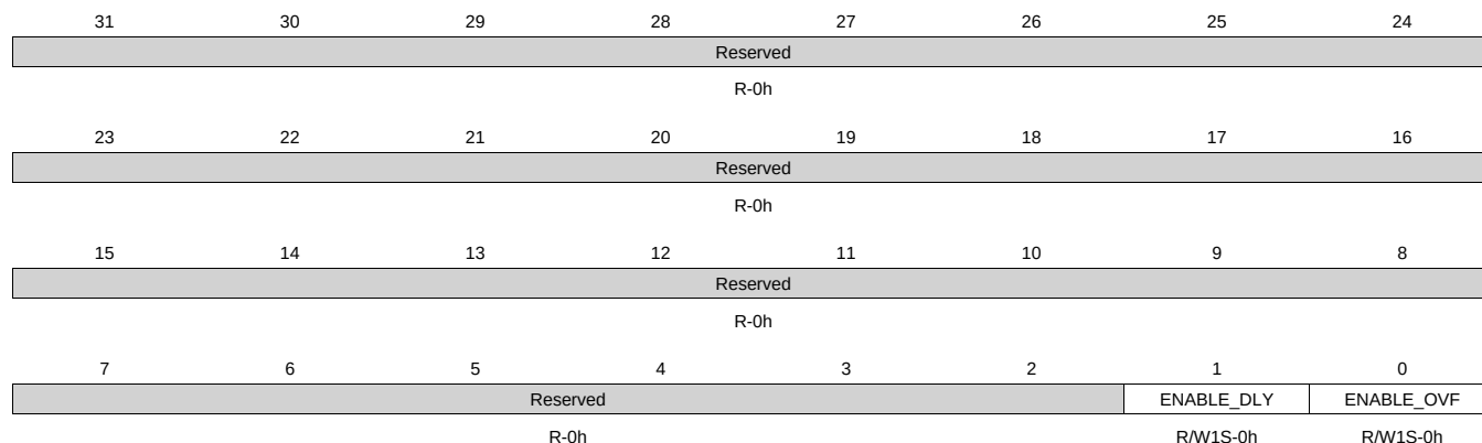
Figure 20-113. WDT_WIRQENSET Register
