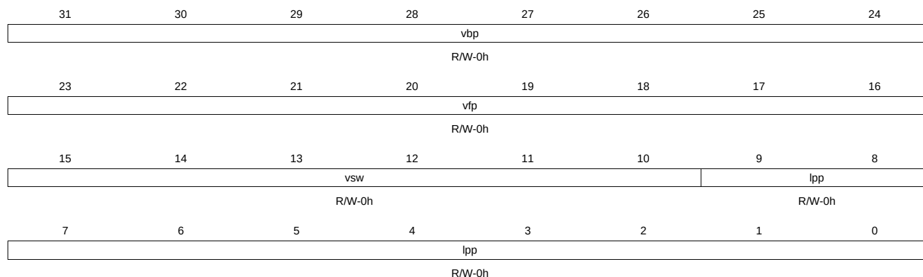
Figure 13-30. RASTER_TIMING_1 Register
