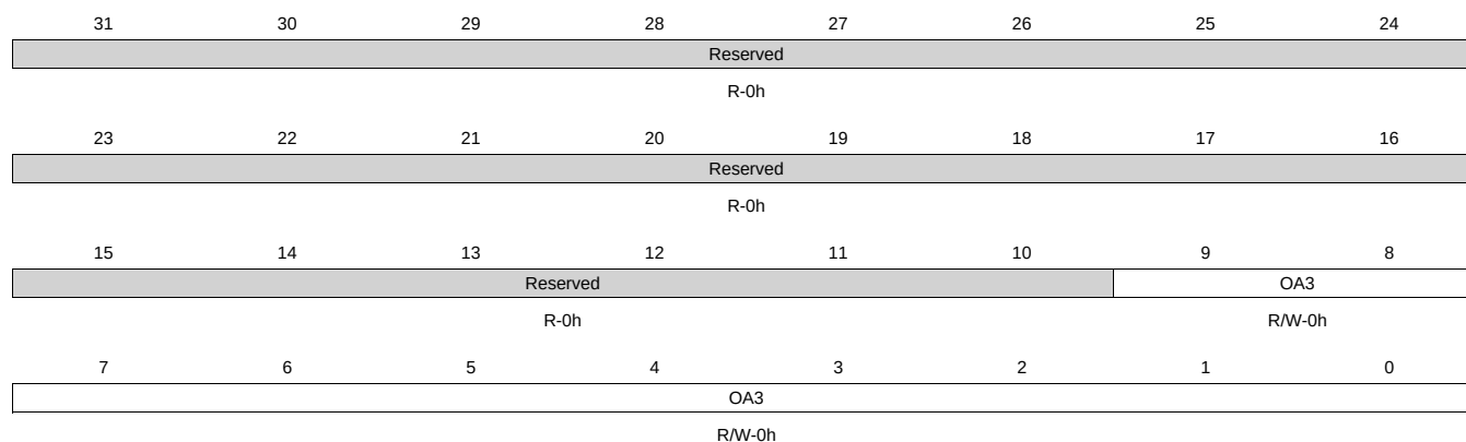
Figure 21-44. I2C_OA3 Register
