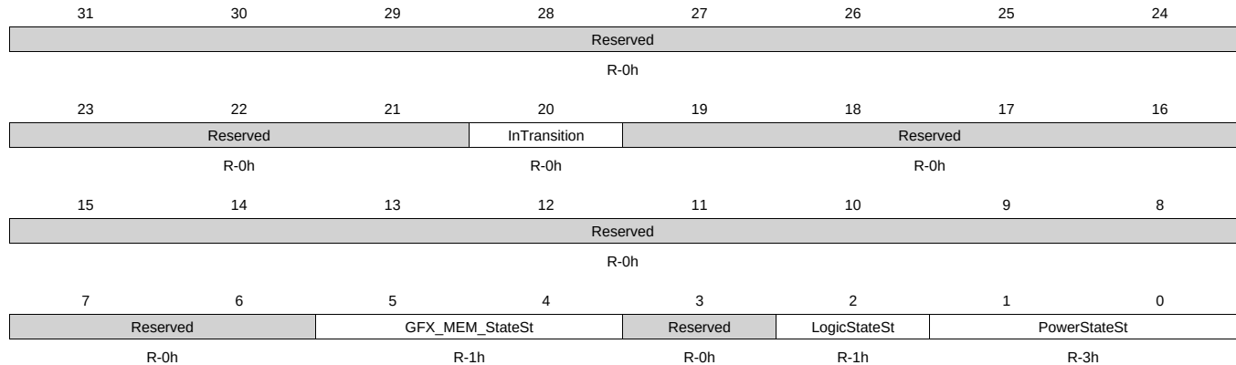
Figure 8-191. PM_GFX_PWRSTST Register
