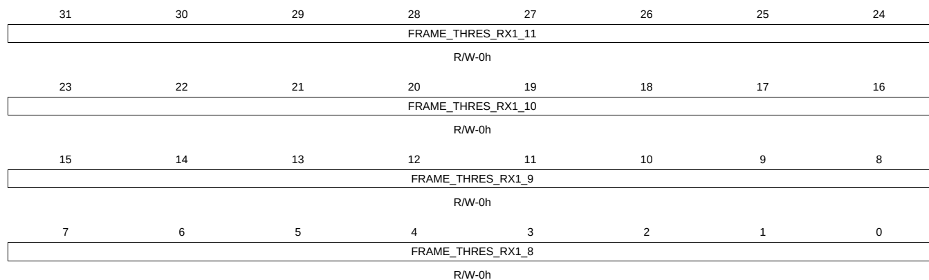
Figure 16-60. IRQFRAMETHOLDRX12 Register
