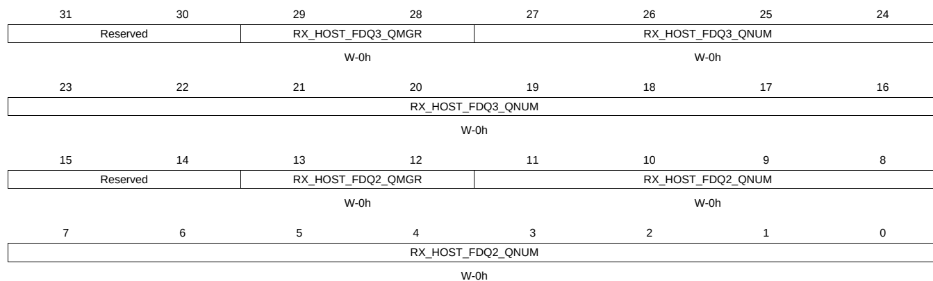
Figure 16-190. RXHPCRB8 Register
