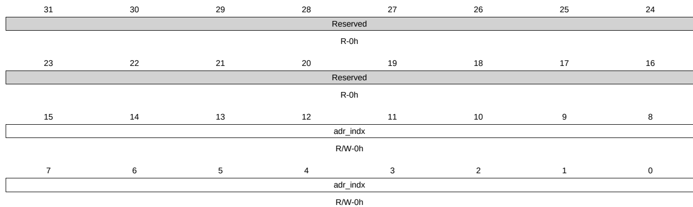
Figure 13-26. LIDD_CS1_ADDR Register
