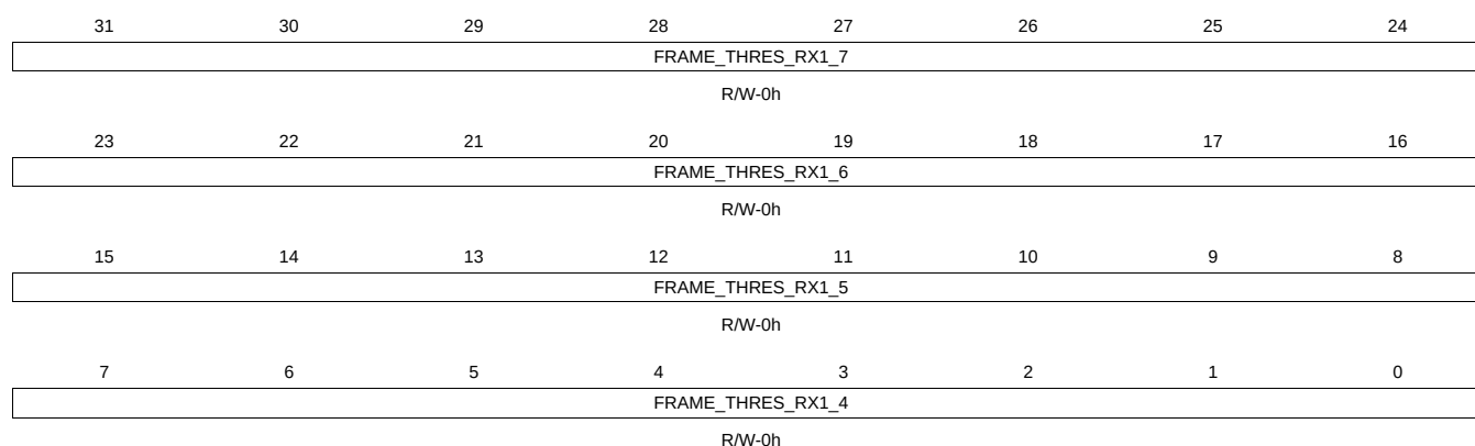
Figure 16-59. IRQFRAMETHOLDRX11 Register
