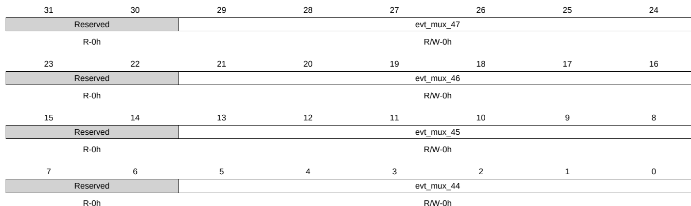
Figure 9-70. tpcc_evt_mux_44_47 Register
