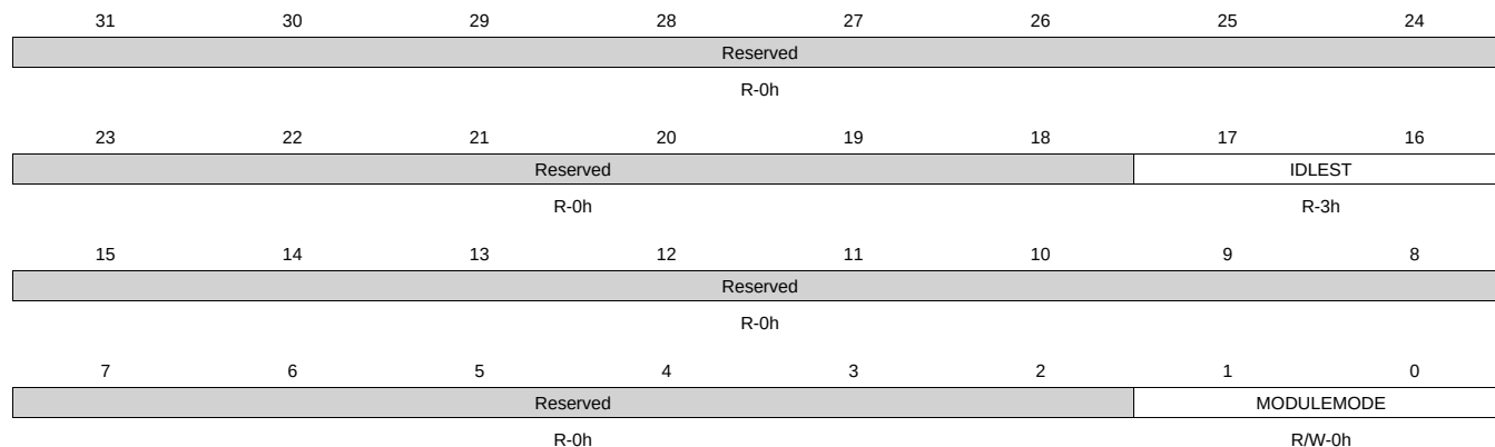
Figure 8-47. CM_PER_UART3_CLKCTRL Register
