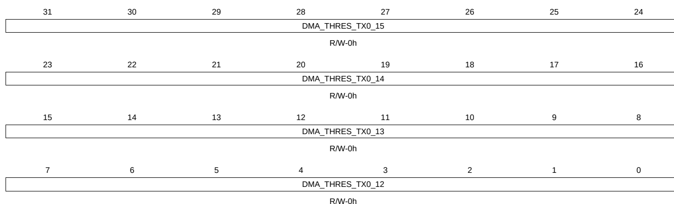
Figure 16-31. IRQDMATHOLDTX03 Register
