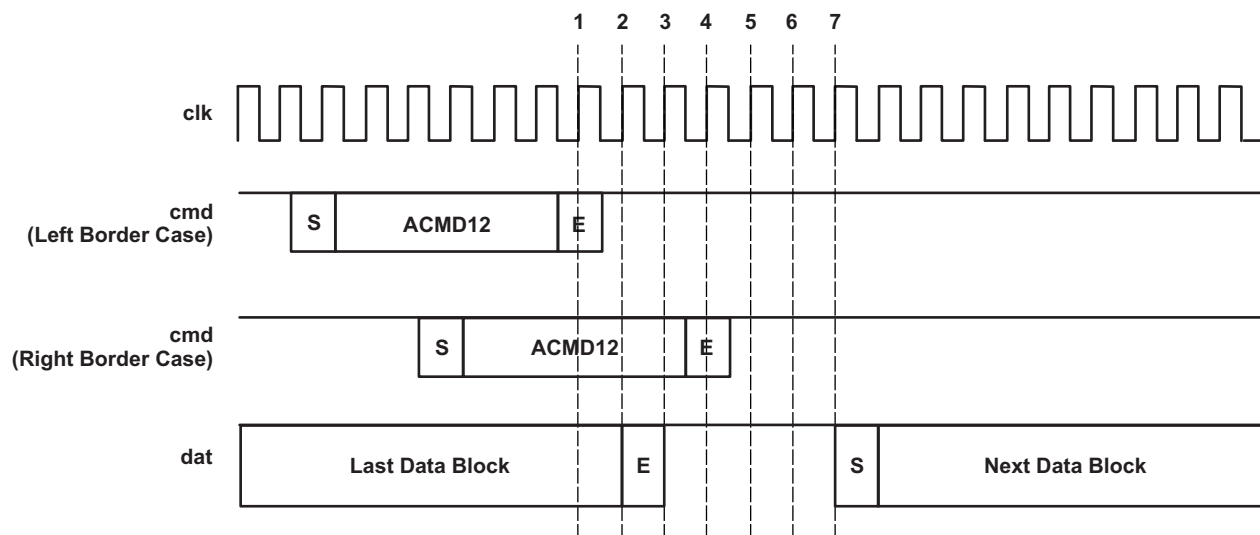
Figure 18-28. Auto Command 12 Timings During Read Transfer
