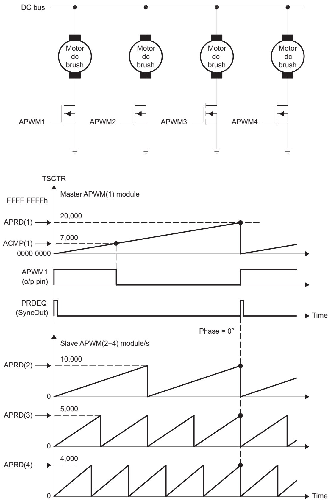
Figure 15-114. Multichannel PWM Example Using 4 eCAP Modules
