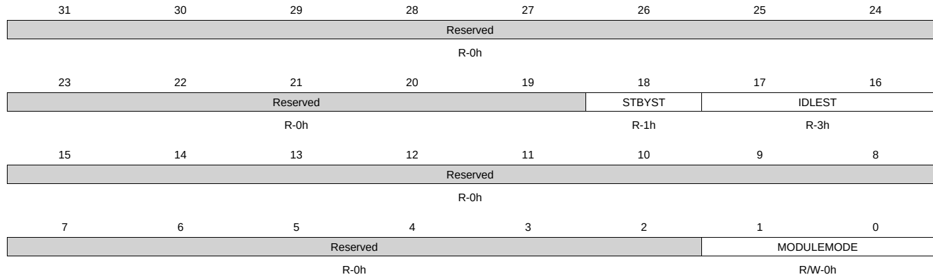
Figure 8-27. CM_PER_CPGMAC0_CLKCTRL Register
