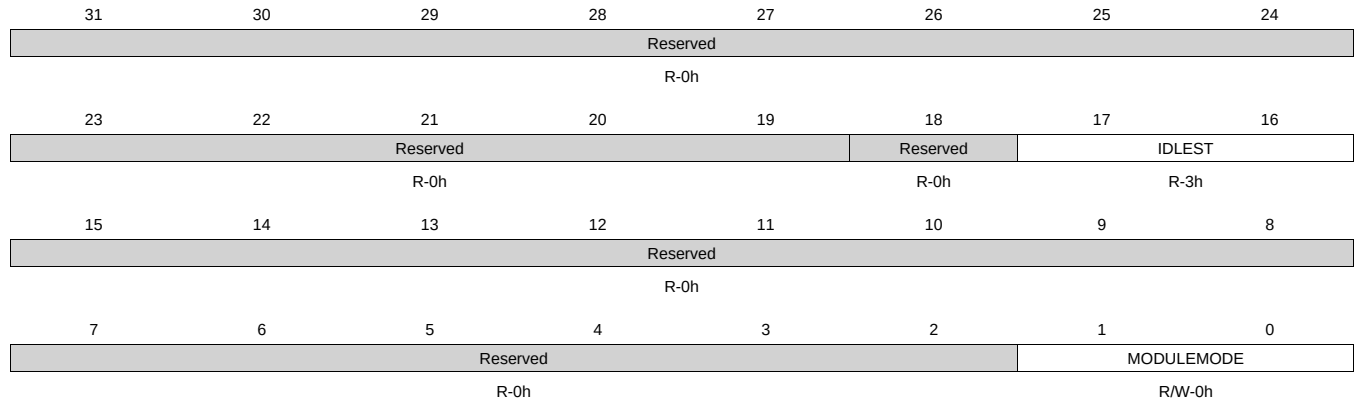
Figure 8-133. CM_WKUP_TIMER1_CLKCTRL Register
