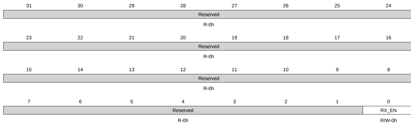
Figure 14-33. RX_CONTROL Register
