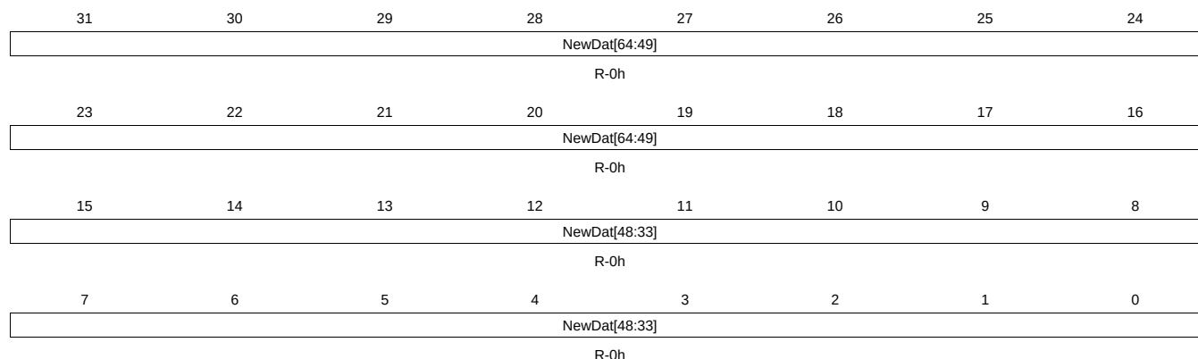
Figure 23-34. NWDAT34 Register
