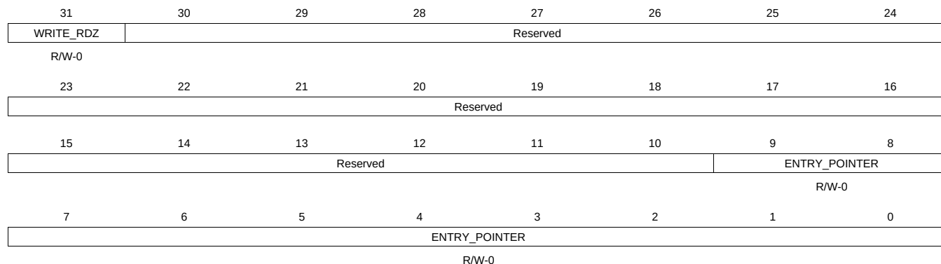
Figure 14-19. TBLCTL Register
