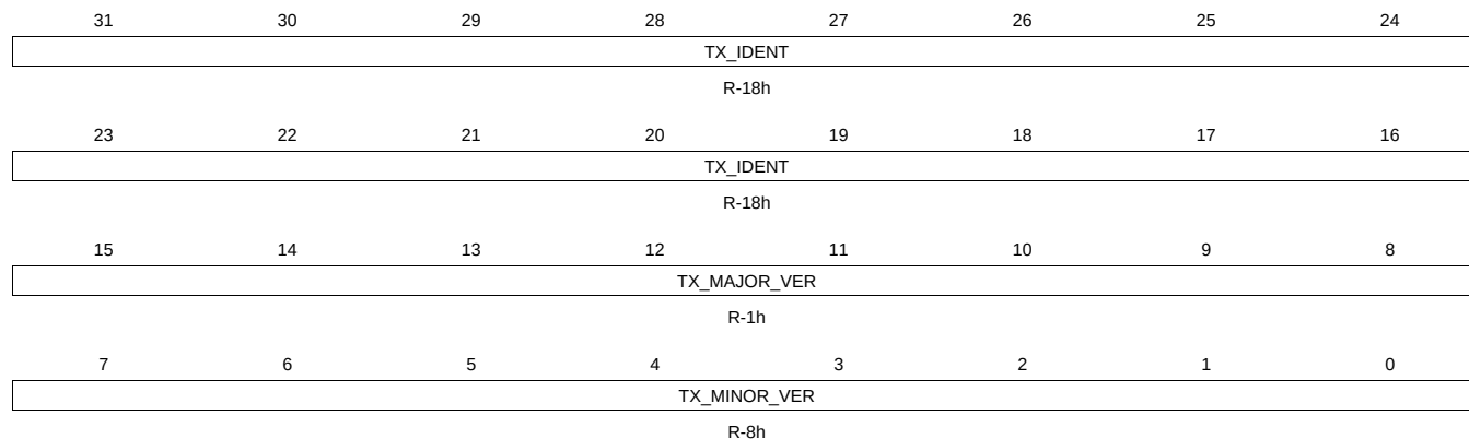
Figure 14-29. TX_IDVER Register
