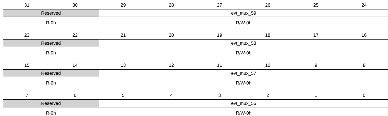
Figure 9-73. tpcc_evt_mux_56_59 Register
