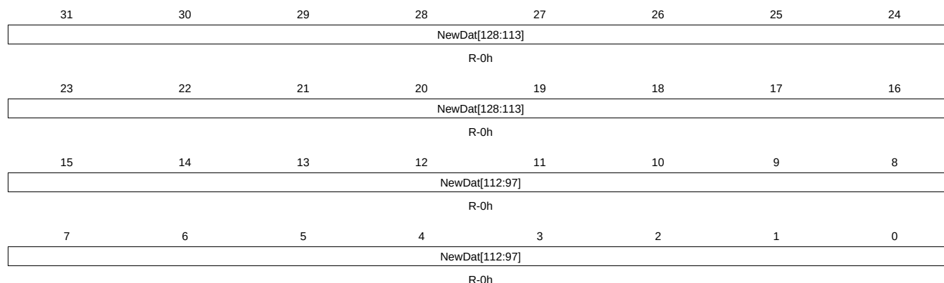
Figure 23-36. NWDAT78 Register
