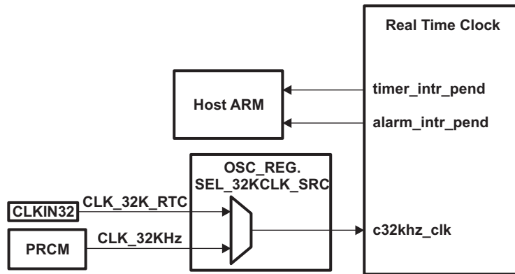
Figure 20-56. RTC Block Diagram
