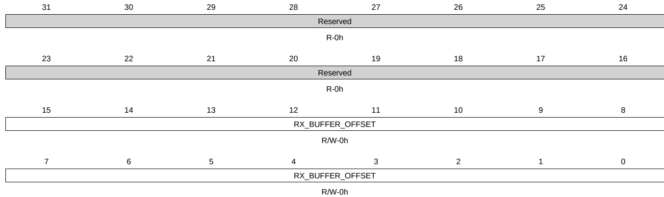
Figure 14-38. RX_BUFFER_OFFSET Register
