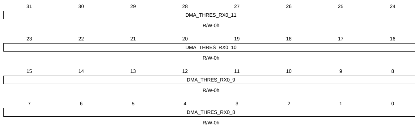
Figure 16-34. IRQDMATHOLDRX02 Register
