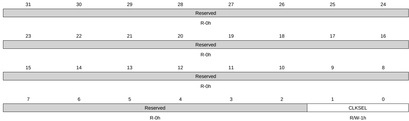
Figure 8-138. CLKSEL_TIMER7_CLK Register
