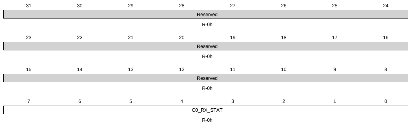
Figure 14-214. C0_RX_STAT Register
