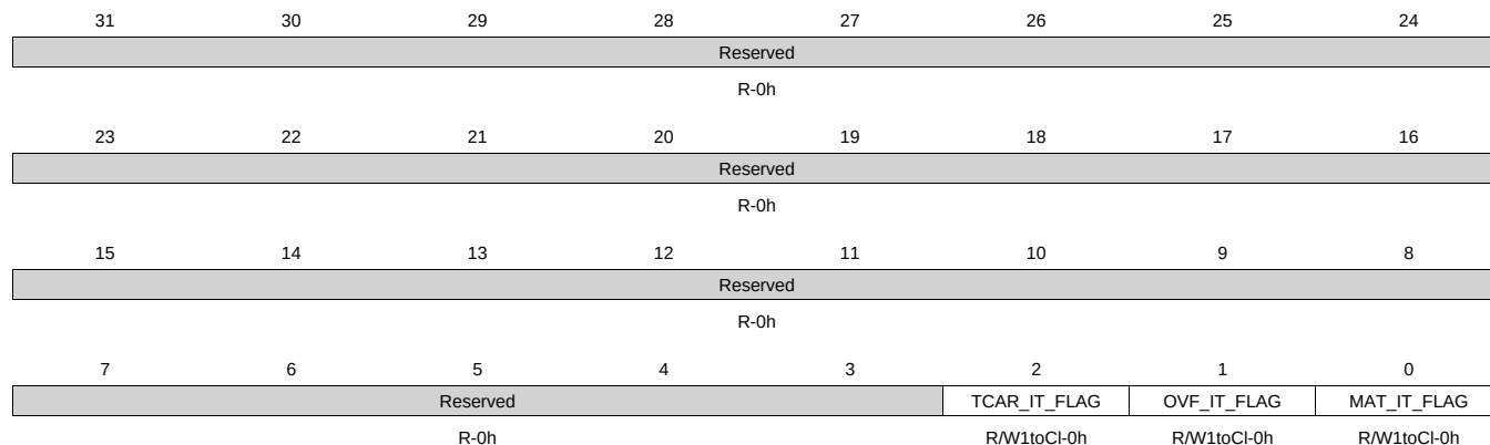
Figure 20-38. TISR Register
