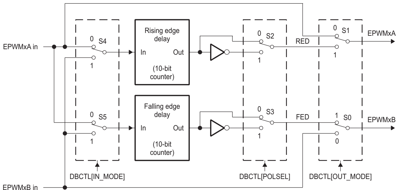
Figure 15-34. Configuration Options for the Dead-Band Generator Submodule
