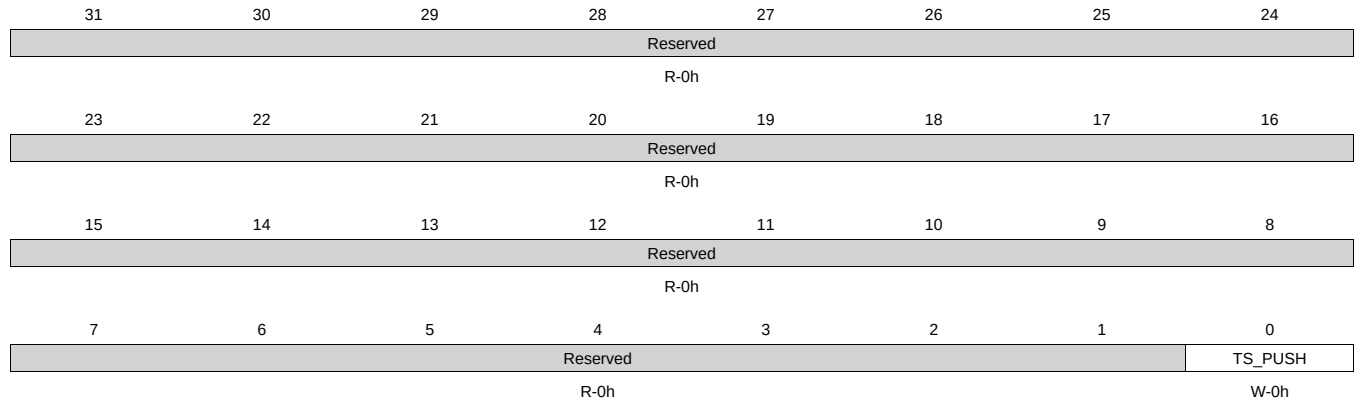
Figure 14-80. CPTS_TS_PUSH Register
