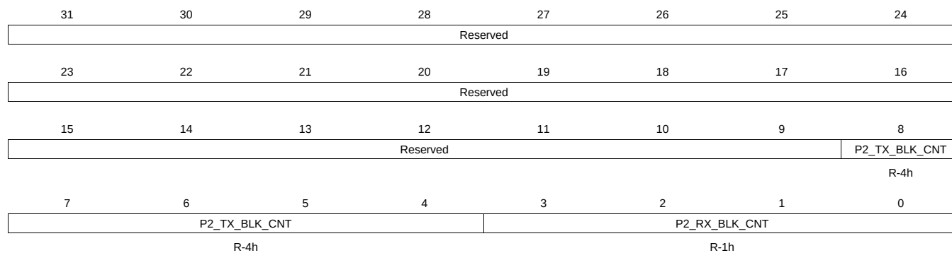
Figure 14-157. P2_BLK_CNT Register
