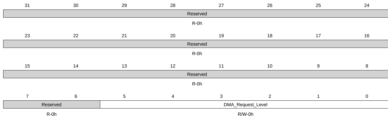
Figure 12-60. DMA1REQ Register
