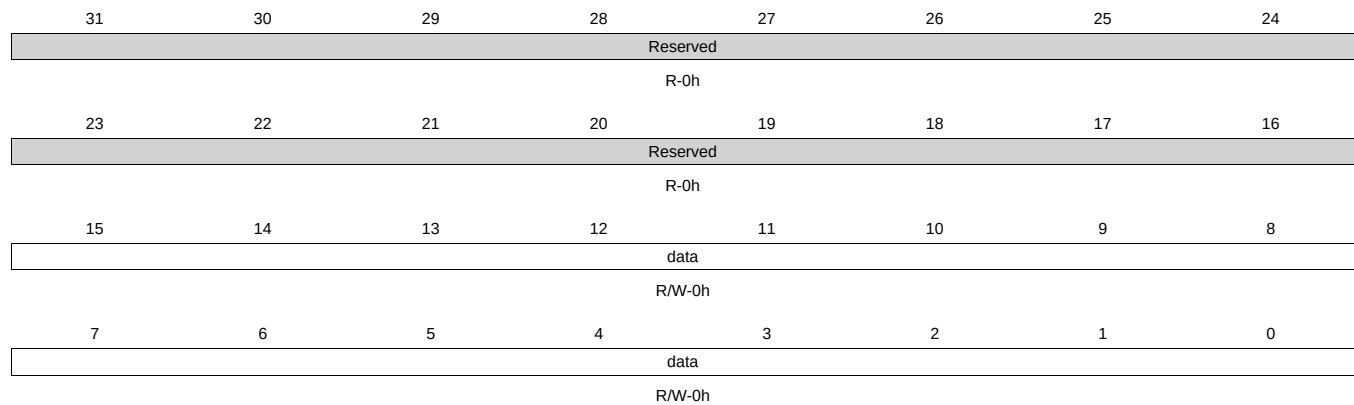
Figure 13-24. LIDD_CS0_DATA Register
