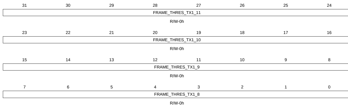
Figure 16-56. IRQFRAMETHOLDTX12 Register
