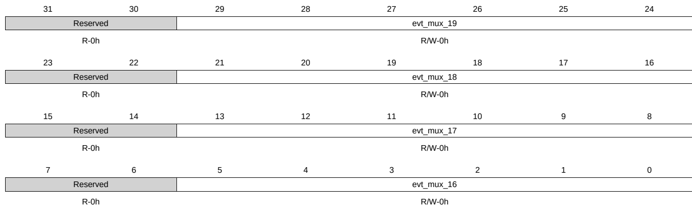
Figure 9-63. tpcc_evt_mux_16_19 Register
