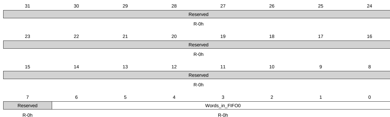
Figure 12-55. FIFO0COUNT Register
