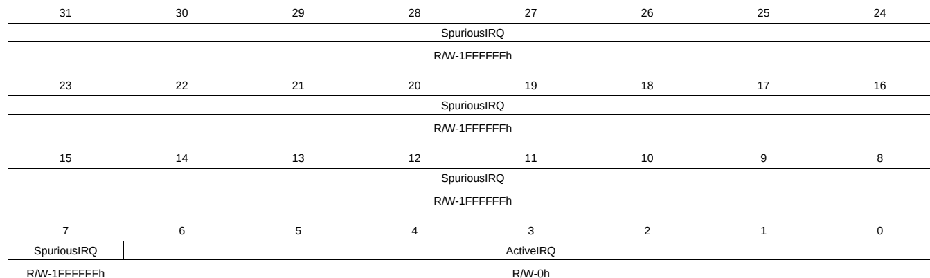
Figure 6-7. INTC_SIR_IRQ Register
