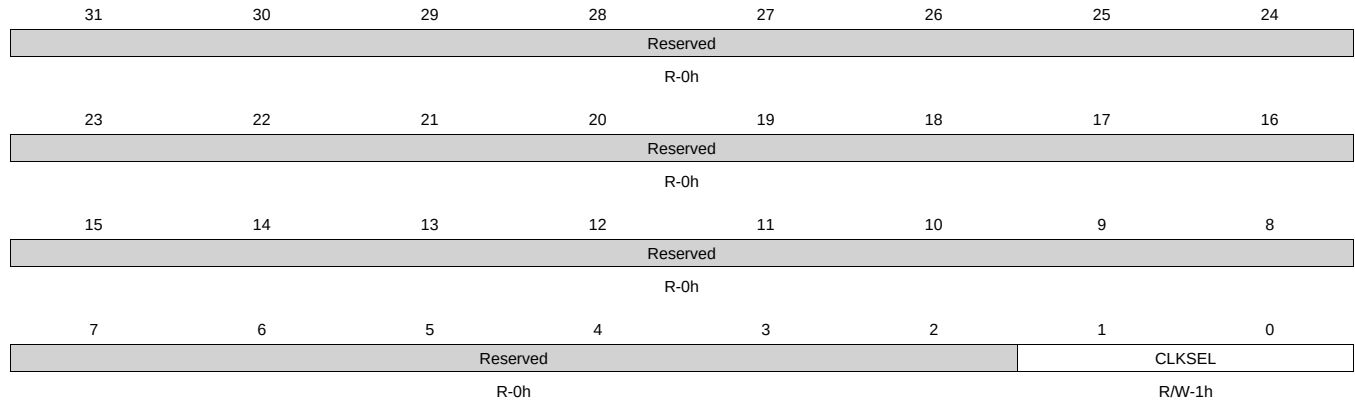
Figure 8-140. CLKSEL_TIMER3_CLK Register
