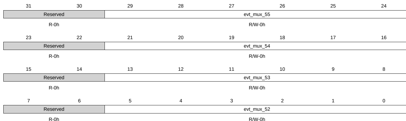
Figure 9-72. tpcc_evt_mux_52_55 Register
