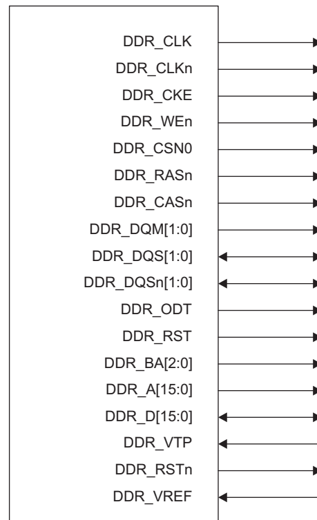
Figure 7-88. DDR2/3/mDDR Memory Controller Signals
