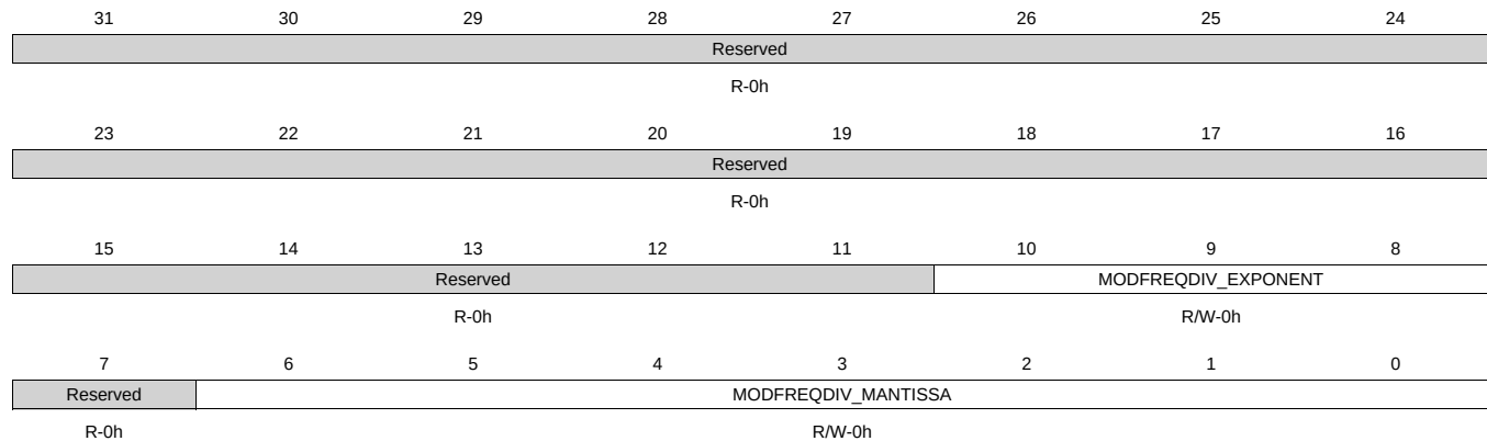
Figure 8-114. CM_SSC_MODFREQDIV_DPLL_PER Register
