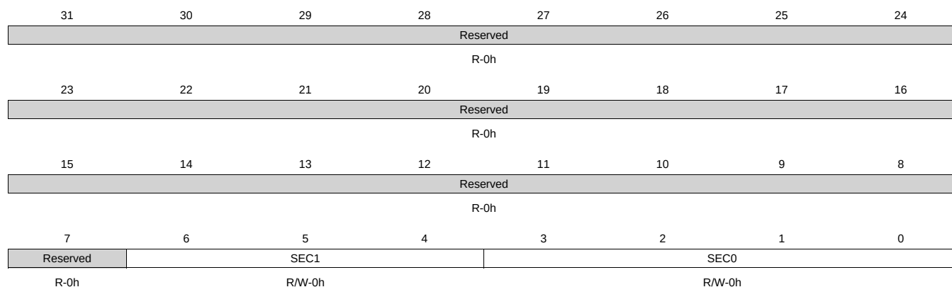
Figure 20-61. SECONDS_REG Register
