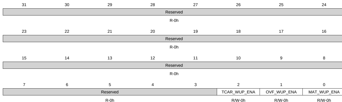
Figure 20-16. IRQWAKEEN Register
