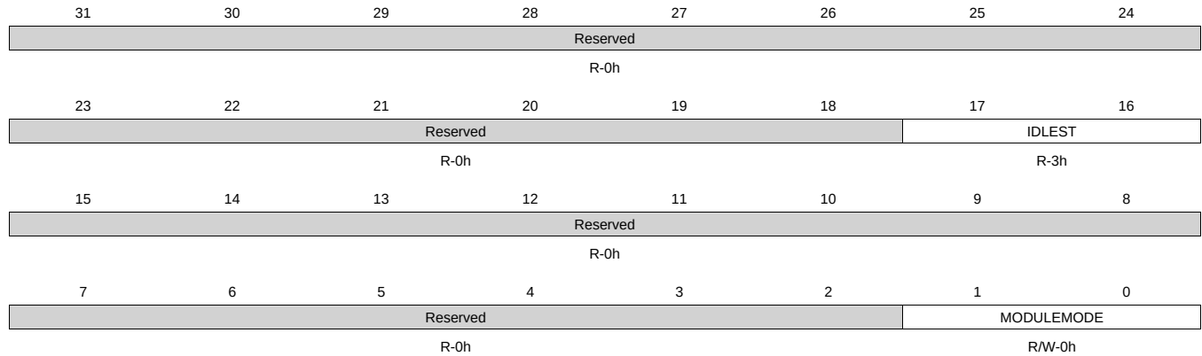
Figure 8-59. CM_PER_EPWMSS1_CLKCTRL Register
