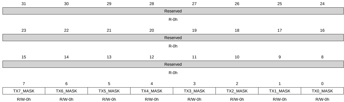
Figure 14-51. TX_INTMASK_CLEAR Register
