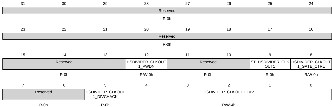
Figure 8-116. CM_DIV_M4_DPLL_CORE Register
