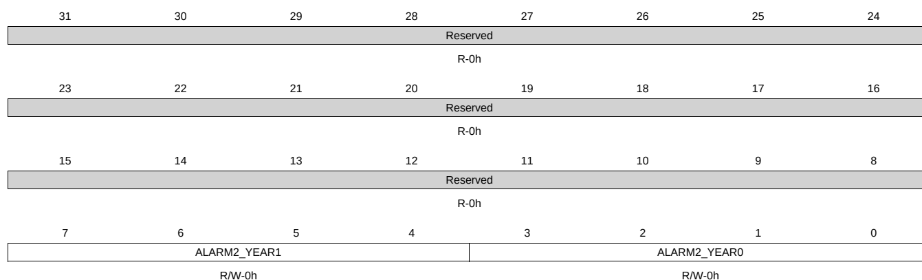
Figure 20-93. ALARM2_YEARS_REG Register
