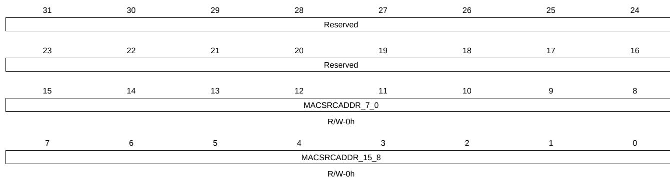
Figure 14-144. P1_SA_LO Register
