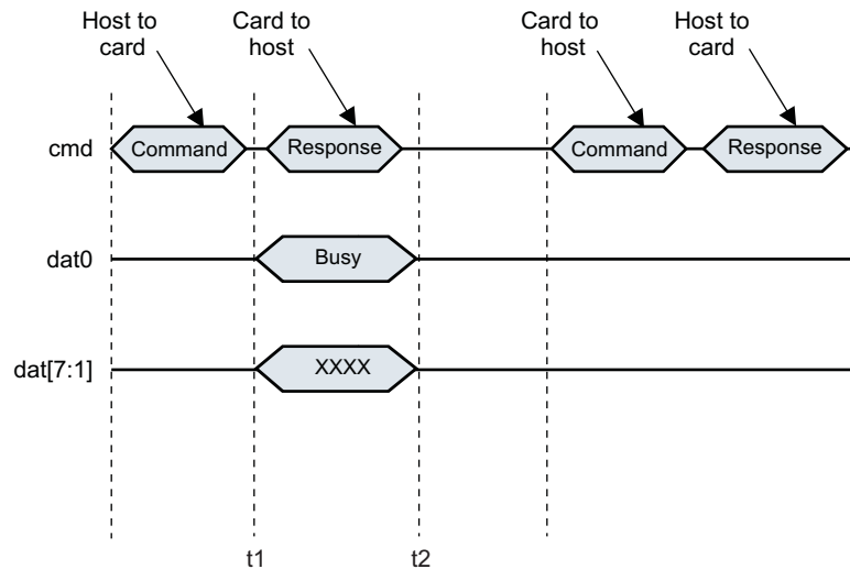
Figure 18-21. Busy Timeout for R1b, R5b Responses
