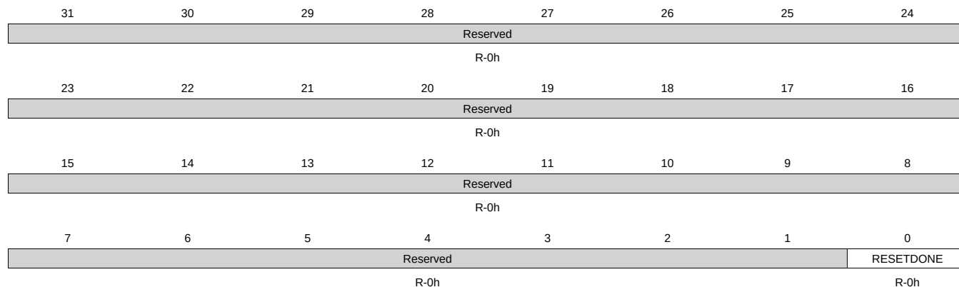
Figure 18-38. SD_SYSSTATUS Register
