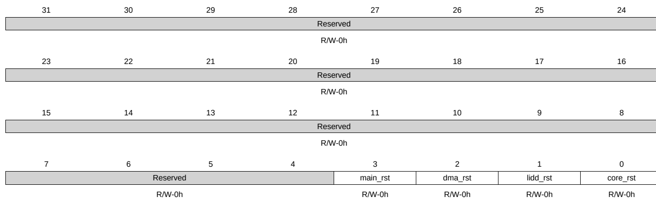
Figure 13-45. CLKC_RESET Register
