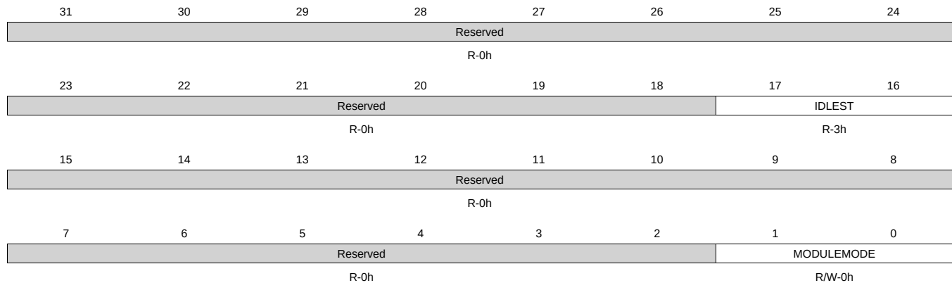
Figure 8-40. CM_PER_SPI0_CLKCTRL Register
