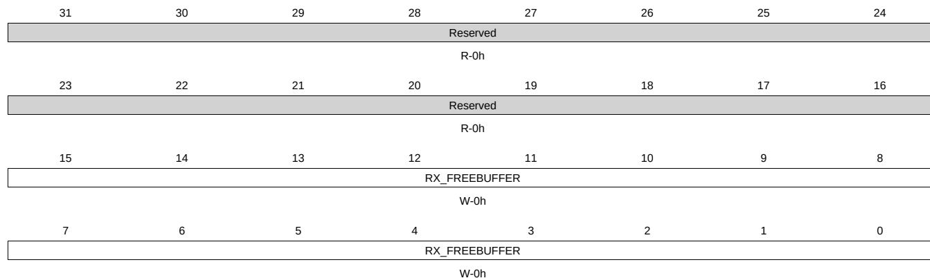
Figure 14-73. RX3_FREEBUFFER Register
