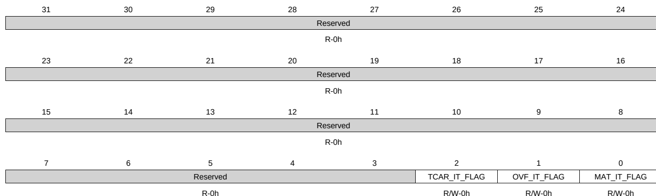
Figure 20-12. IRQSTATUS_RAW Register
