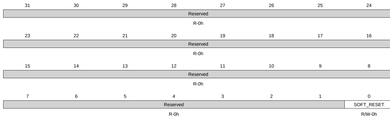
Figure 14-35. CPDMA_SOFT_RESET Register
