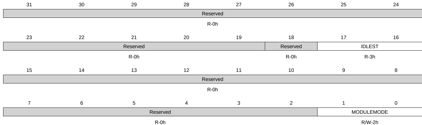
Figure 8-136. CM_WKUP_WDT1_CLKCTRL Register
