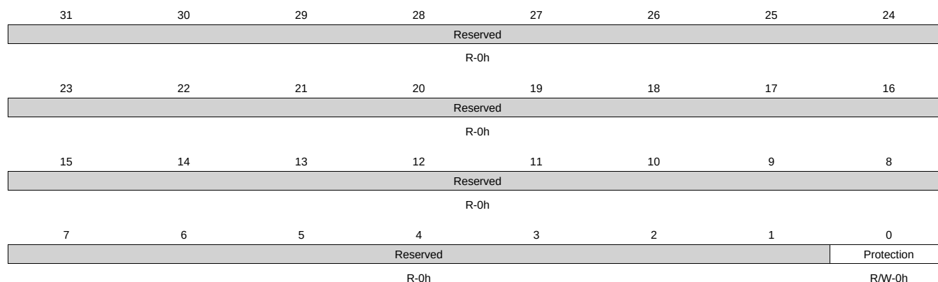
Figure 6-10. INTC_PROTECTION Register
