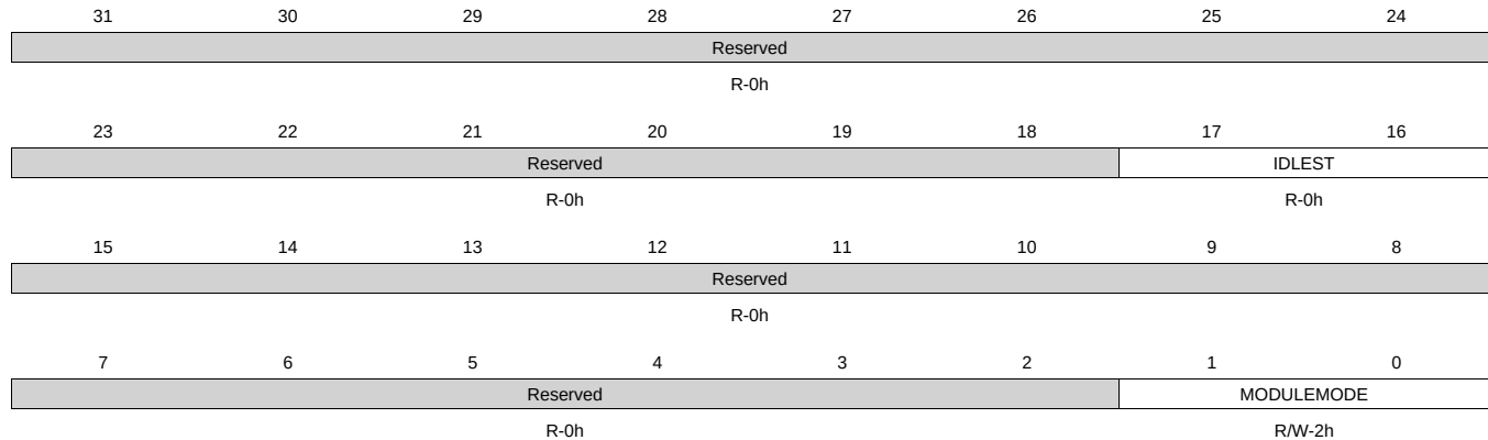
Figure 8-64. CM_PER_L3_CLKCTRL Register
