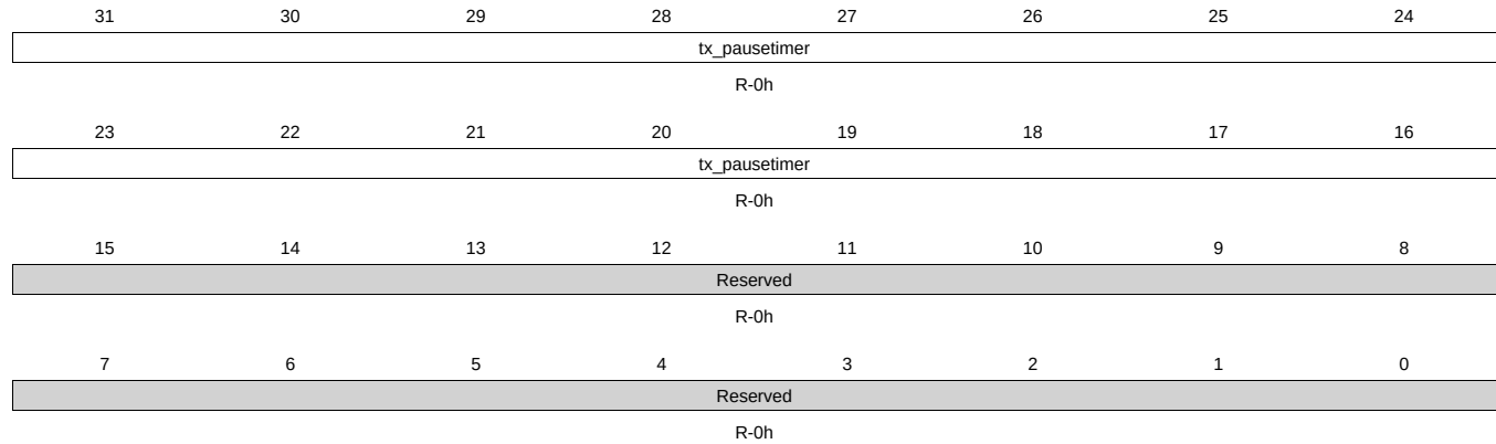
Figure 14-180. TX_PAUSE Register
