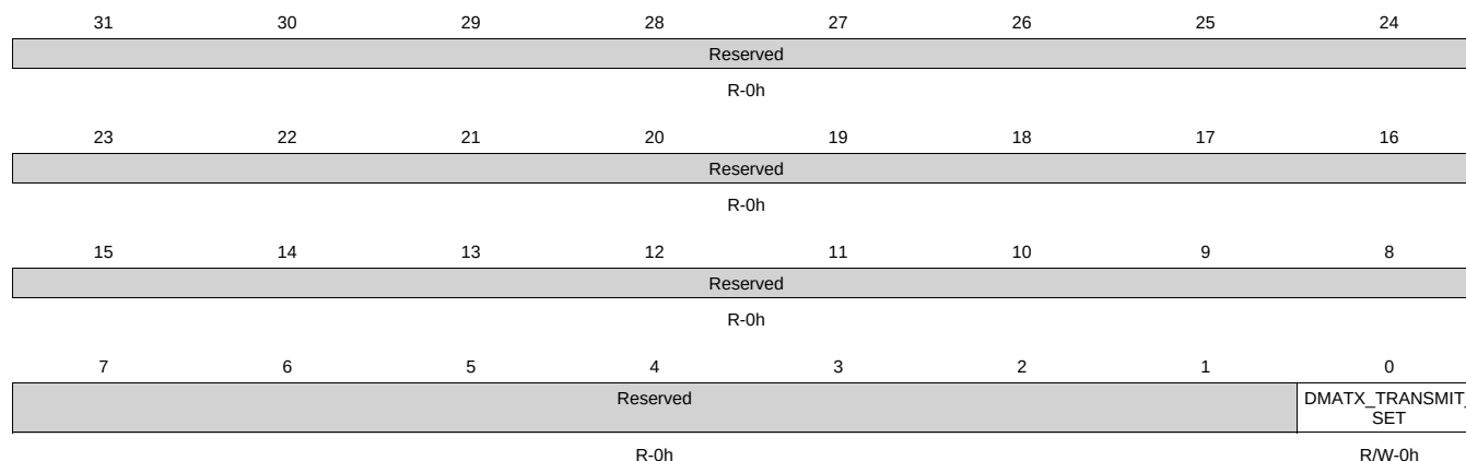
Figure 21-25. I2C_DMATXENABLE_SET Register
