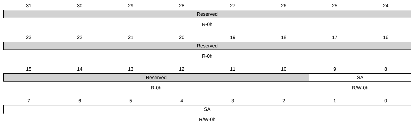
Figure 21-36. I2C_SA Register
