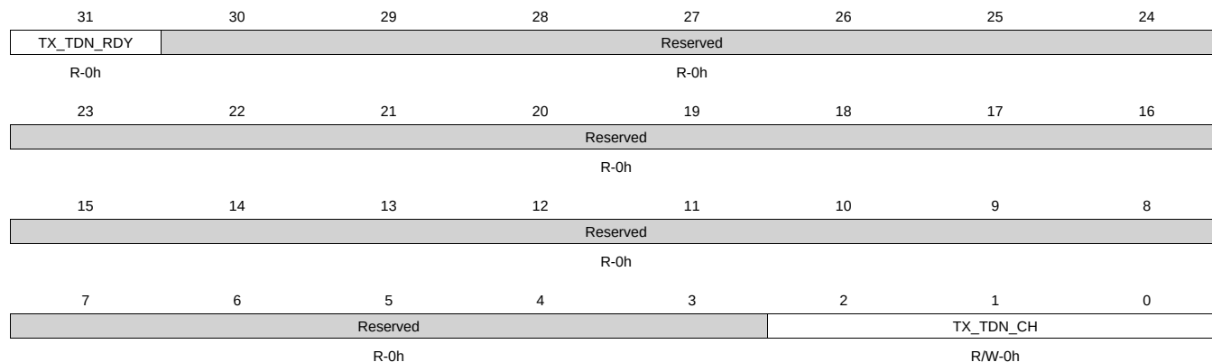
Figure 14-31. TX_TEARDOWN Register
