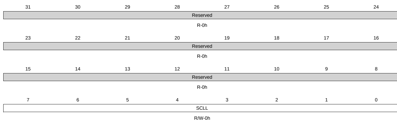
Figure 21-38. I2C_SCLL Register
