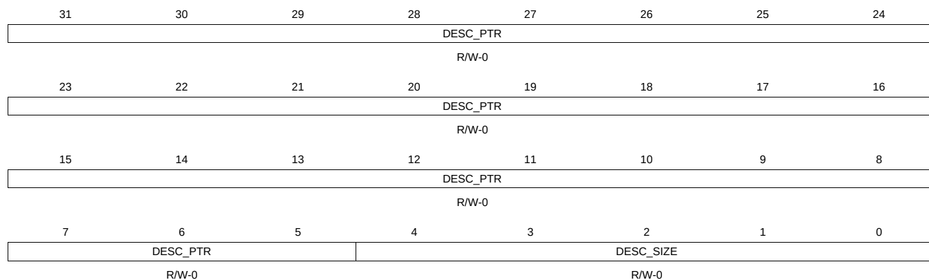
Figure 16-666. QUEUE_88_D Register
