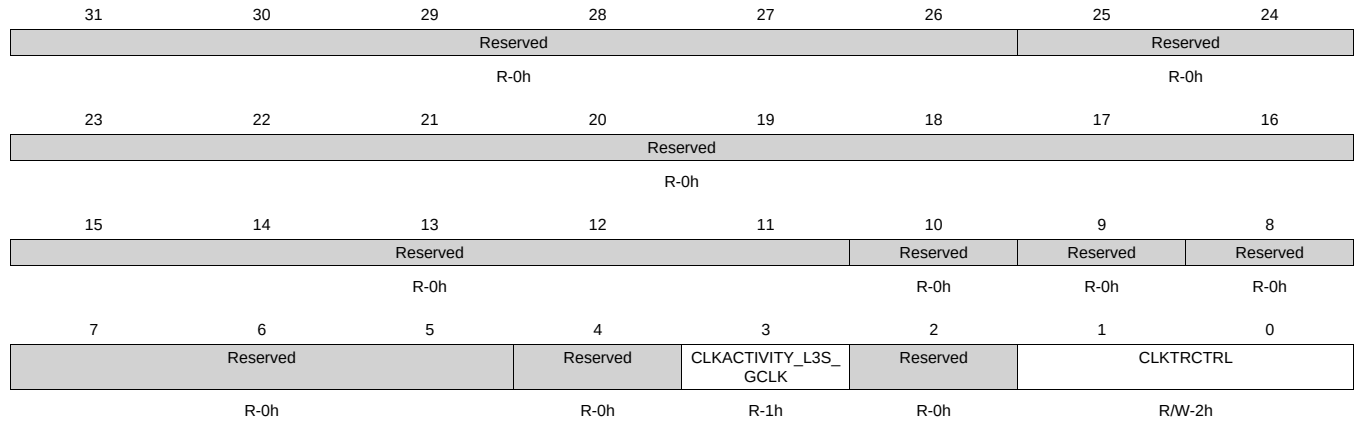
Figure 8-24. CM_PER_L3S_CLKSTCTRL Register
