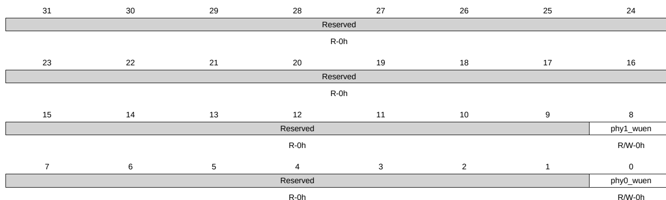
Figure 9-33. usb_wkup_ctrl Register
