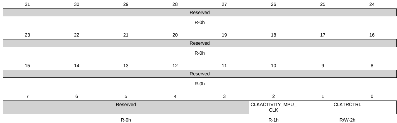
Figure 8-152. CM_MPU_CLKSTCTRL Register
