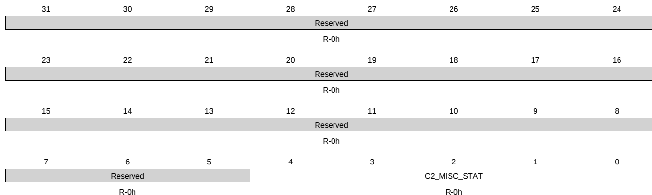
Figure 14-224. C2_MISC_STAT Register
