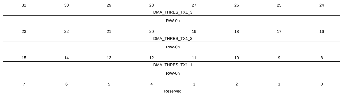
Figure 16-36. IRQDMATHOLDTX10 Register
