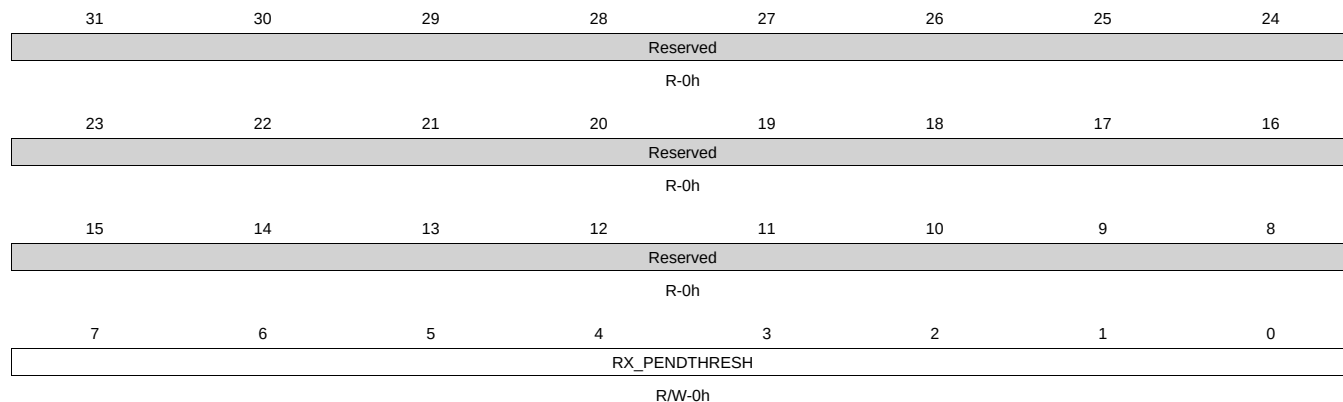
Figure 14-67. RX5_PENDTHRESH Register
