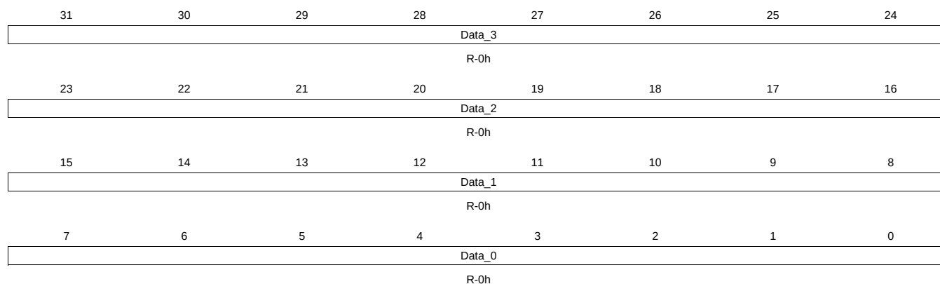
Figure 23-67. IF3DATA Register
