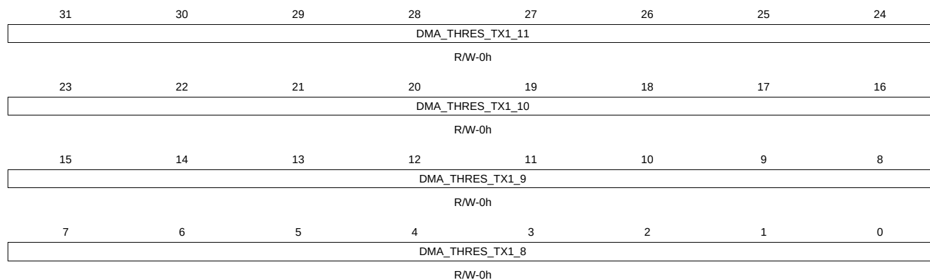
Figure 16-38. IRQDMATHOLDTX12 Register
