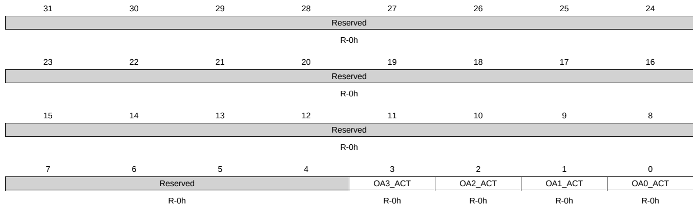
Figure 21-45. I2C_ACTOA Register
