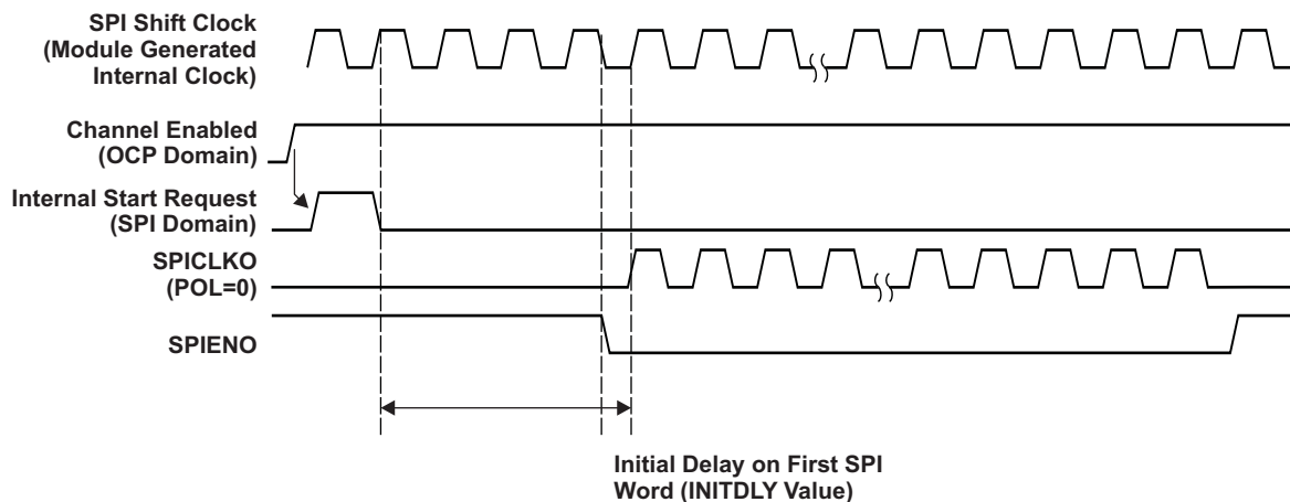
Figure 24-21. Master Single Channel Initial Delay
