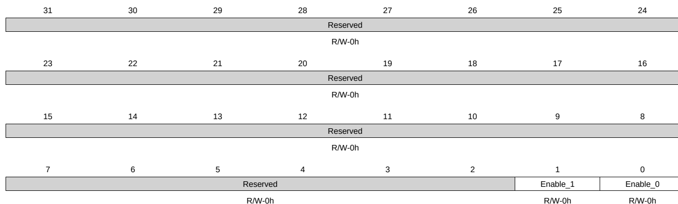
Figure 12-13. DMAENABLE_CLR Register
