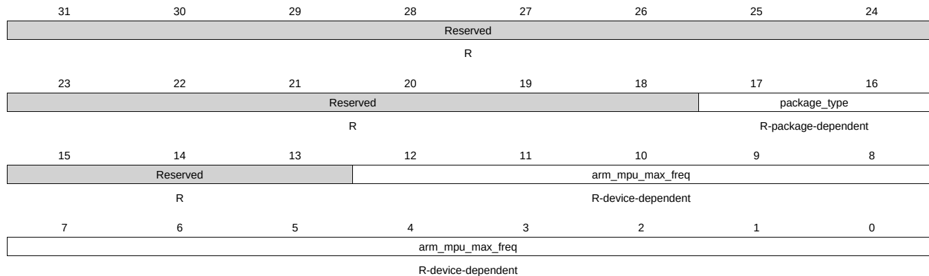
Figure 9-53. efuse_sma Register
