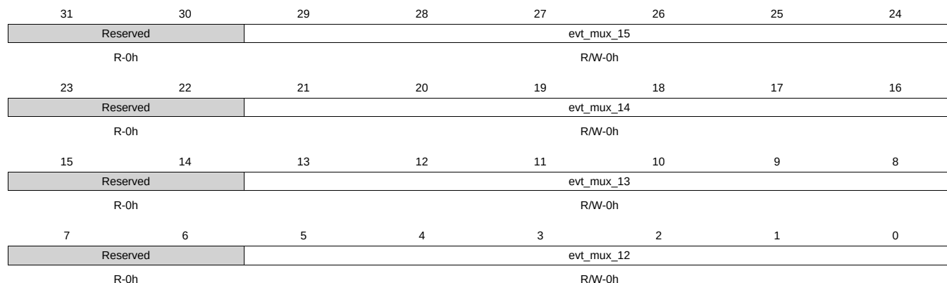
Figure 9-62. tpcc_evt_mux_12_15 Register
