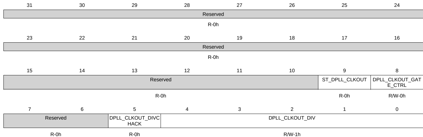
Figure 8-124. CM_DIV_M2_DPLL_DDR Register
