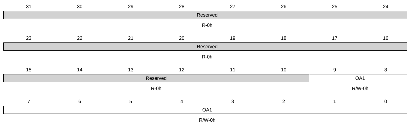
Figure 21-42. I2C_OA1 Register
