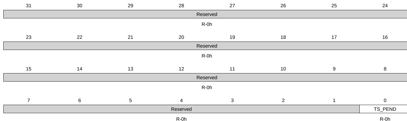
Figure 14-84. CPTS_INTSTAT_MASKED Register
