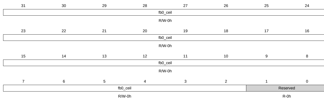
Figure 13-36. LCDDMA_FB0_CEILING Register
