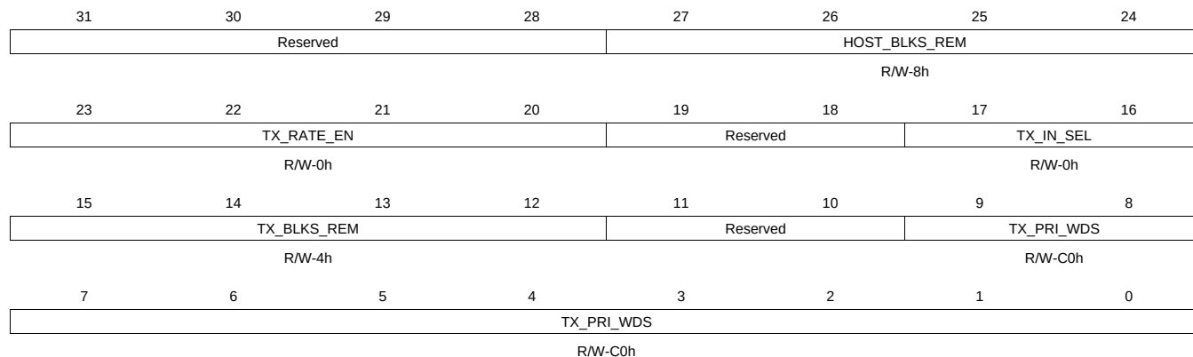
Figure 14-158. P2_TX_IN_CTL Register
