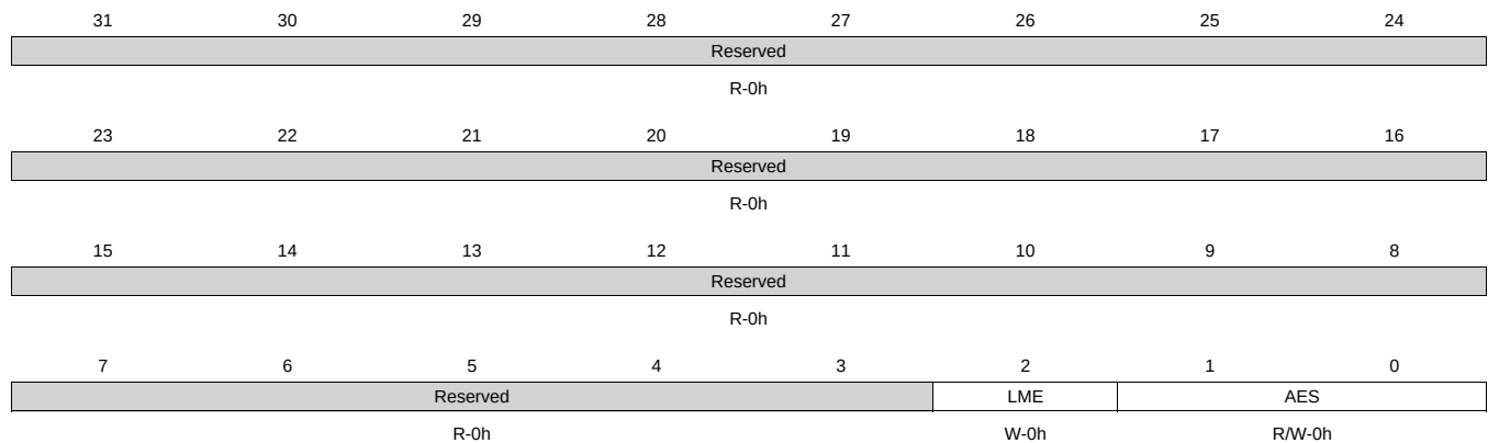
Figure 18-62. SD_ADMAES Register
