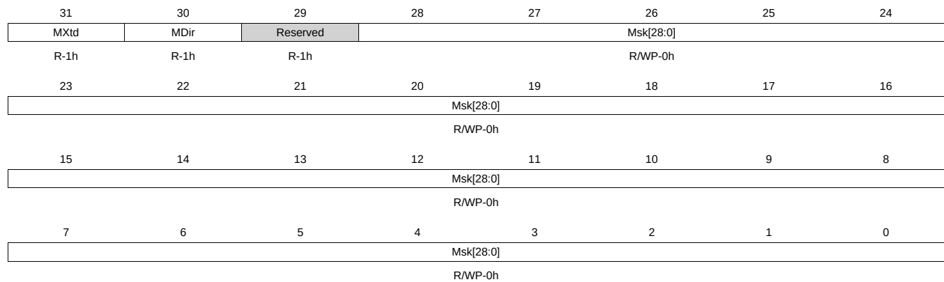
Figure 23-64. IF3MSK Register
