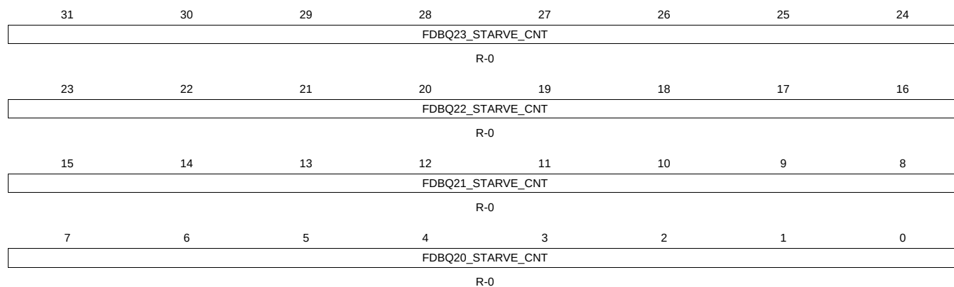
Figure 16-284. FDBSC5 Register
