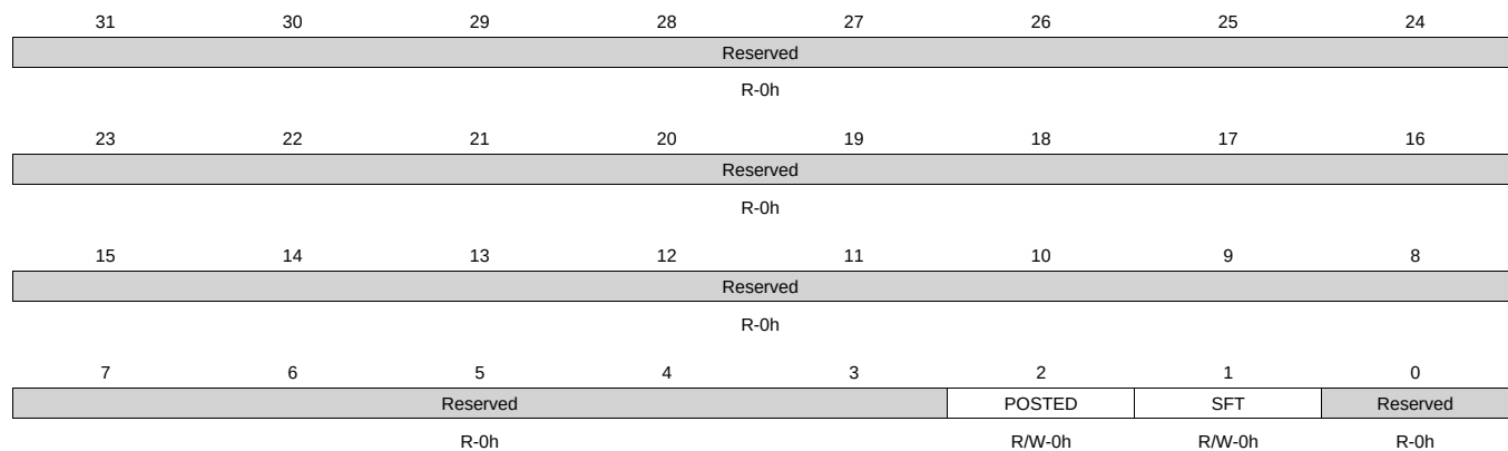
Figure 20-24. TSICR Register
