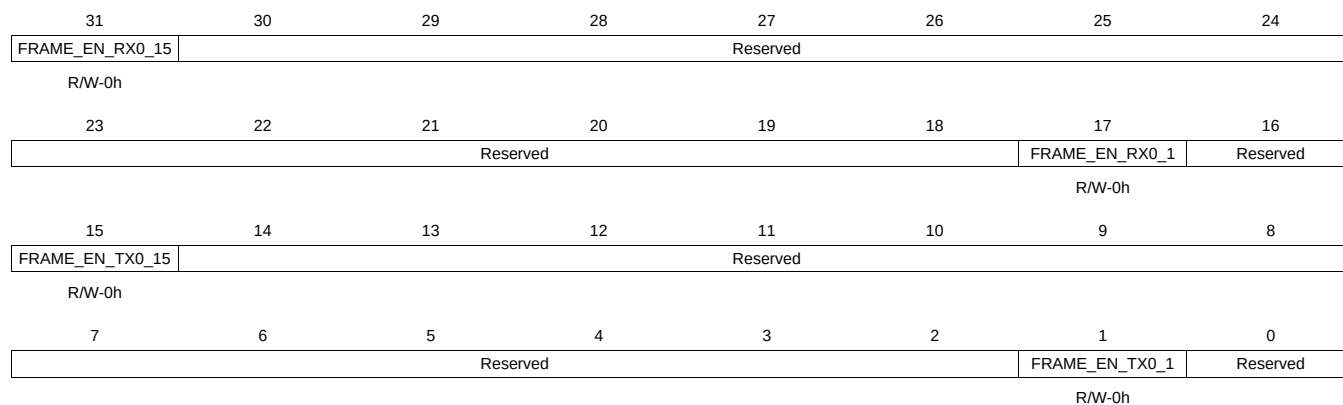
Figure 16-62. IRQFRAMEENABLE0 Register
