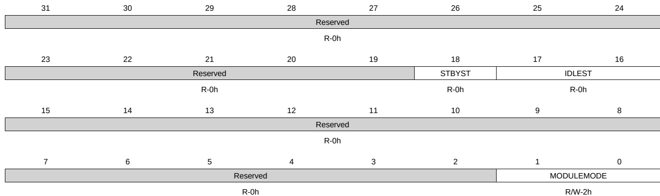
Figure 8-153. CM_MPU_MPU_CLKCTRL Register
