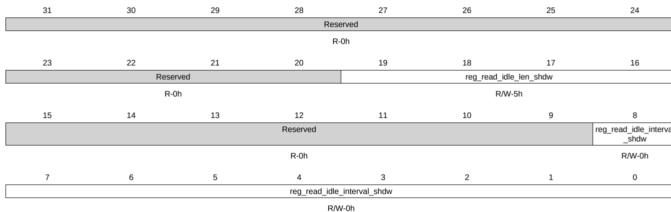
Figure 7-114. READ_IDLE_CTRL_SHDW Register
