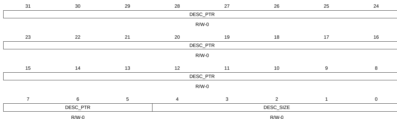
Figure 16-838. QUEUE_131_D Register
