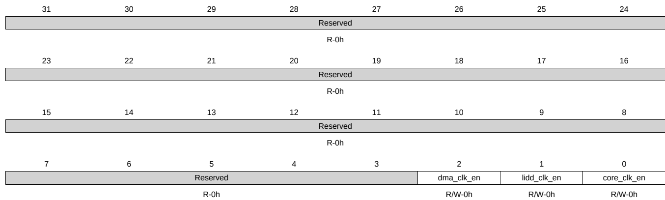
Figure 13-44. CLKC_ENABLE Register
