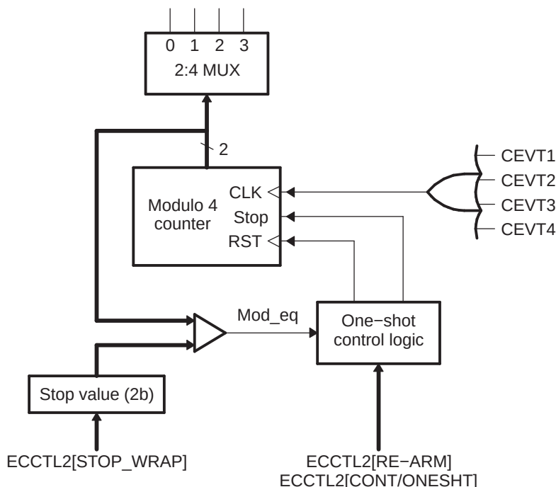
Figure 15-105. Continuous/One-shot Block Diagram
