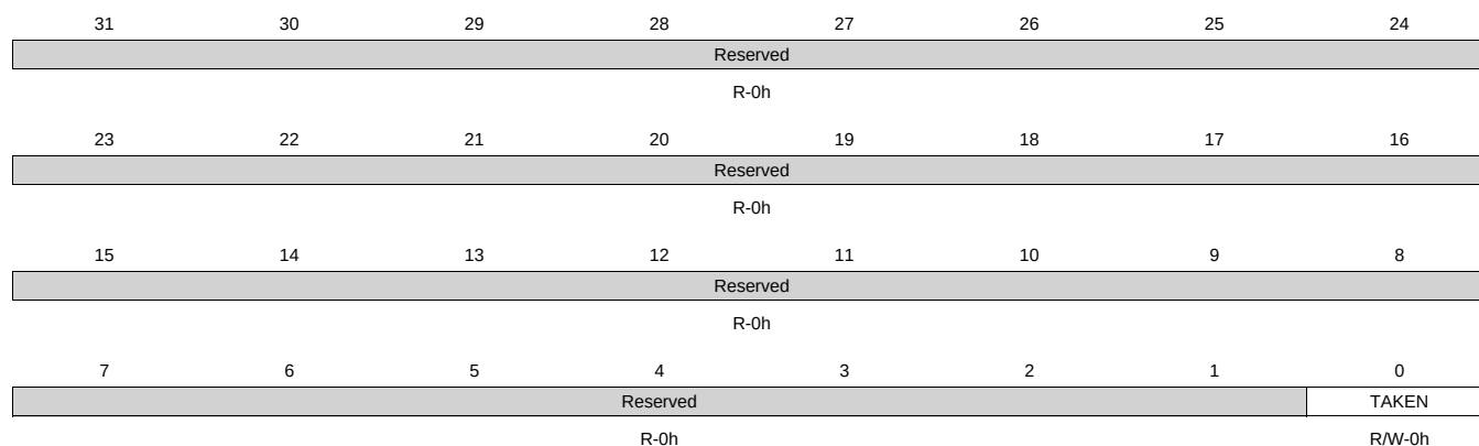
Figure 17-60. LOCK_REG_12 Register
