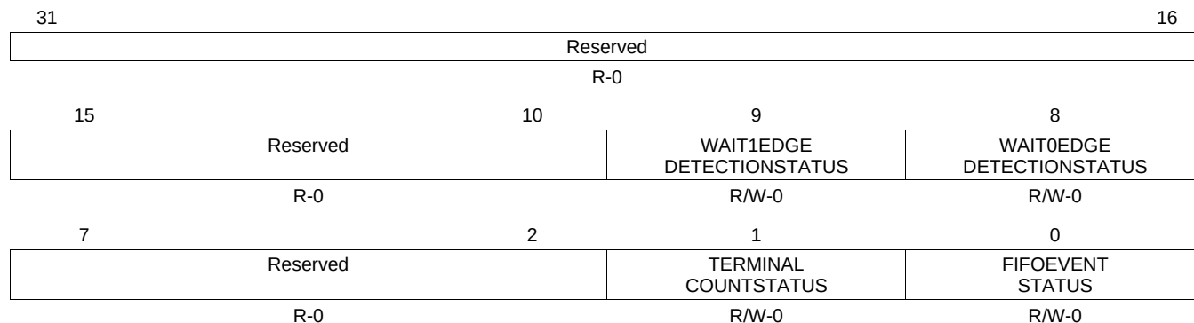
Figure 7-54. GPMC_IRQSTATUS
