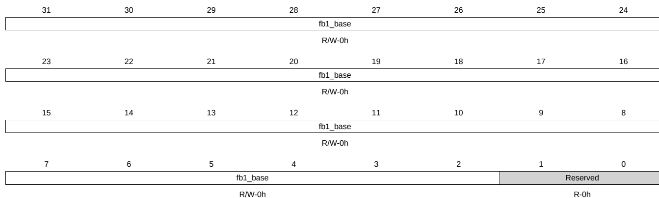
Figure 13-37. LCDDMA_FB1_BASE Register
