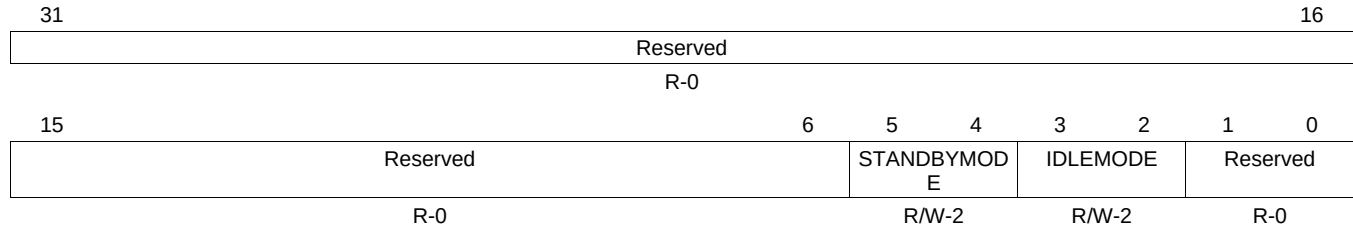
Figure 11-107. EDMA3TC System Configuration Register (SYSCONFIG)
