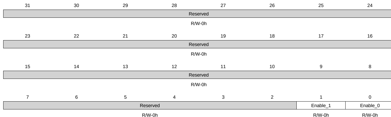
Figure 12-12. DMAENABLE_SET Register
