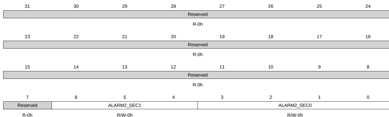
Figure 20-88. ALARM2_SECONDS_REG Register
