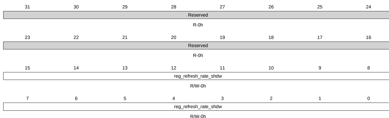
Figure 7-96. SDRAM_REF_CTRL_SHDW Register
