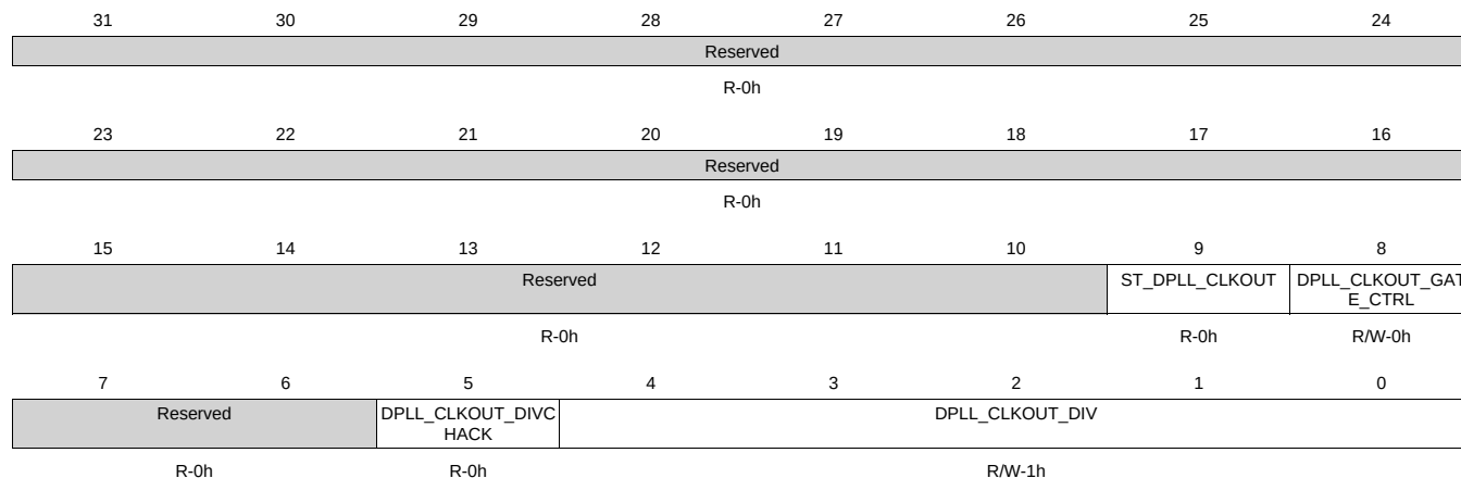
Figure 8-125. CM_DIV_M2_DPLL_DISP Register
