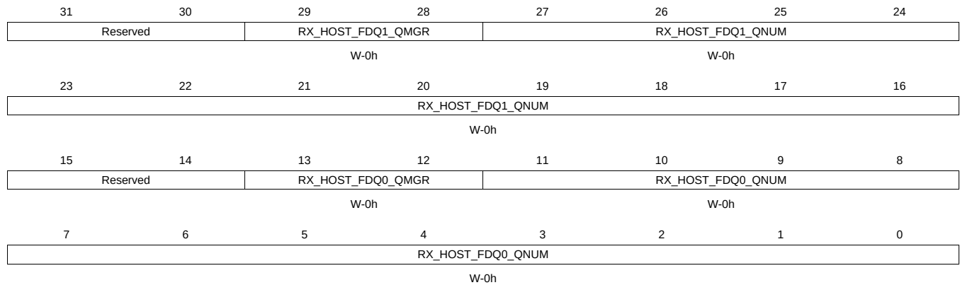
Figure 16-157. RXHPCRA0 Register
