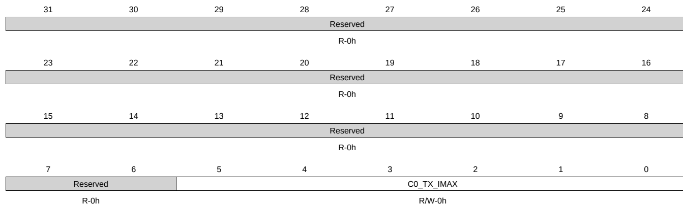
Figure 14-226. C0_TX_IMAX Register
