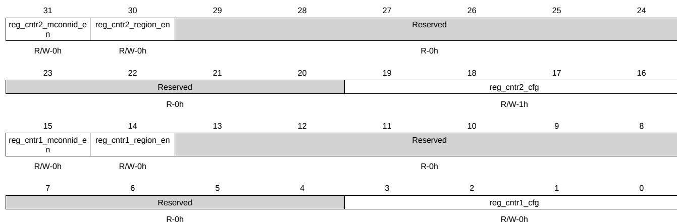
Figure 7-110. PERF_CNT_CFG Register
