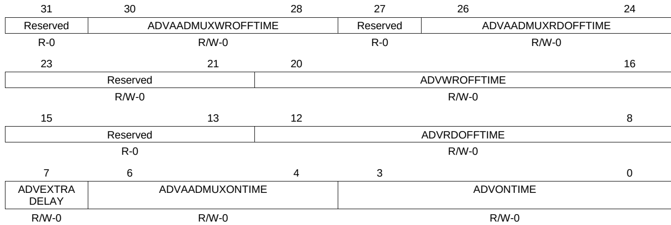
Figure 7-63. GPMC_CONFIG3_i
