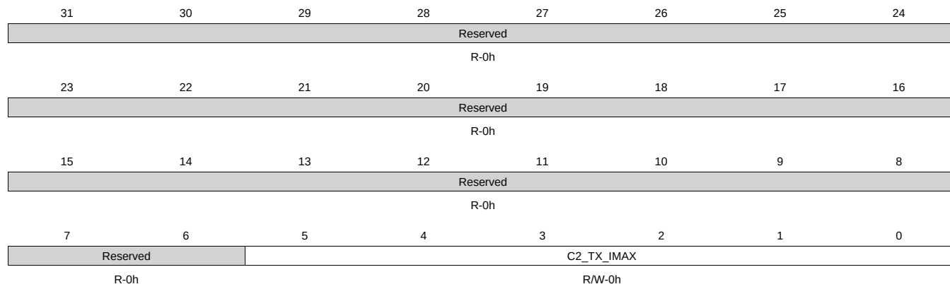
Figure 14-230. C2_TX_IMAX Register
