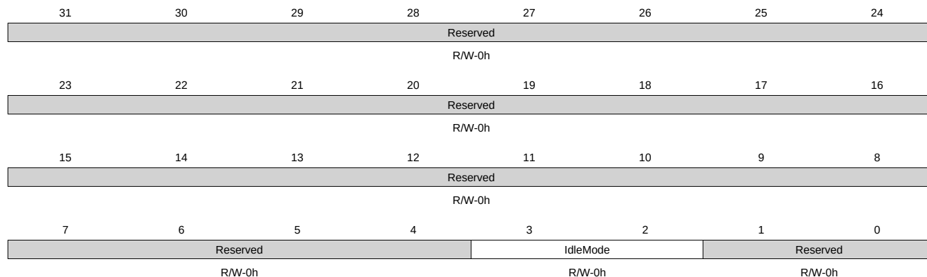
Figure 12-6. SYSCONFIG Register
