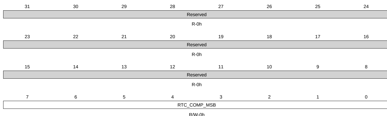
Figure 20-78. RTC_COMP_MSB_REG Register
