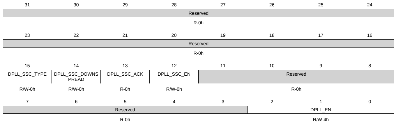
Figure 8-119. CM_CLKMODE_DPLL_PER Register
