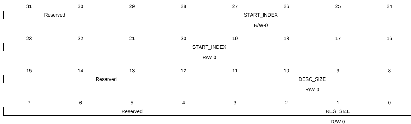
Figure 16-302. QMEMCTRL3 Register
