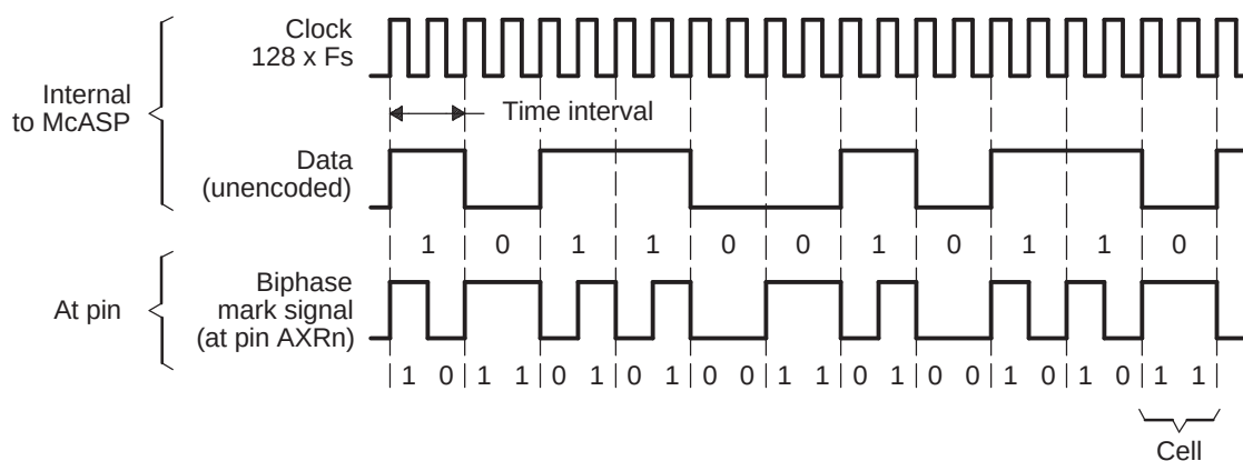
Figure 22-11. Biphasemark Code (BMC)
