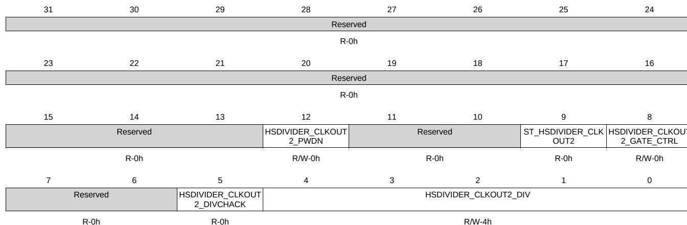
Figure 8-117. CM_DIV_M5_DPLL_CORE Register
