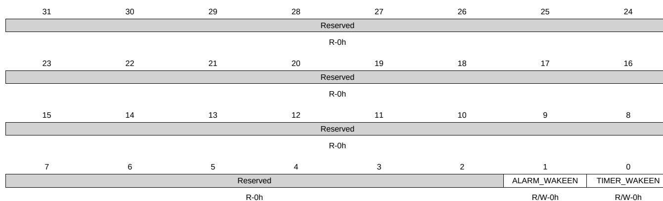
Figure 20-87. RTC_IRQWAKEEN Register
