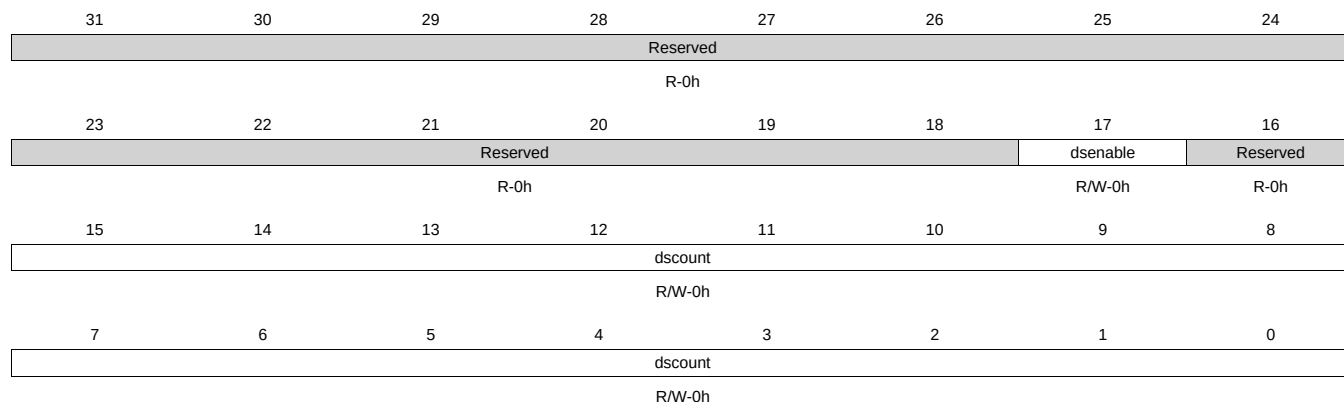
Figure 9-16. deepsleep_ctrl Register
