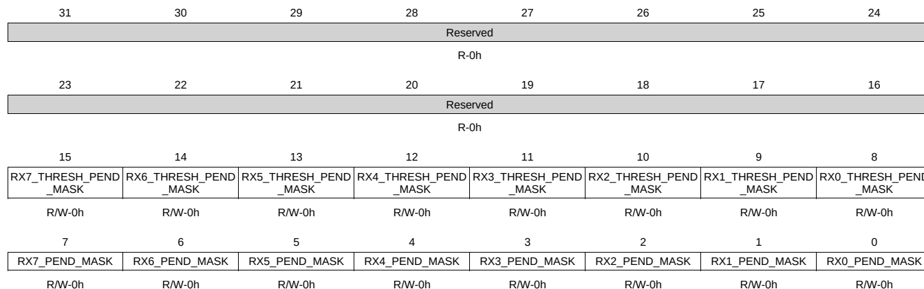
Figure 14-57. RX_INTMASK_CLEAR Register
