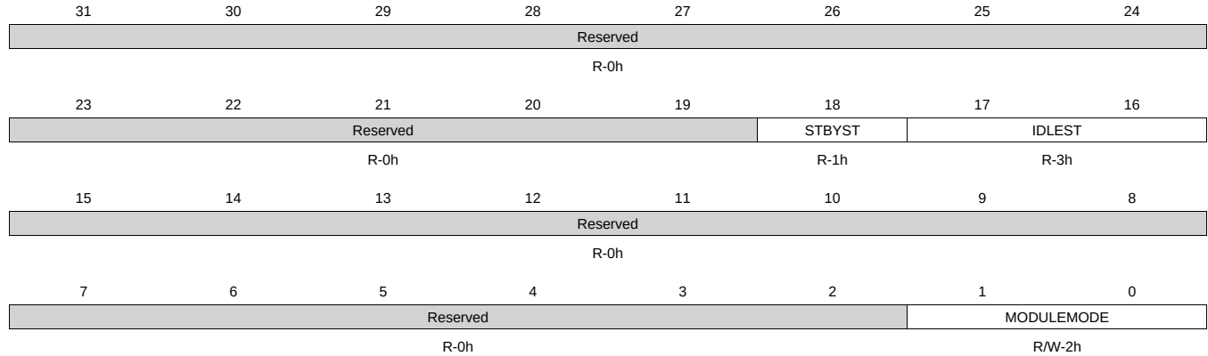
Figure 8-65. CM_PER_IEEE5000_CLKCTRL Register
