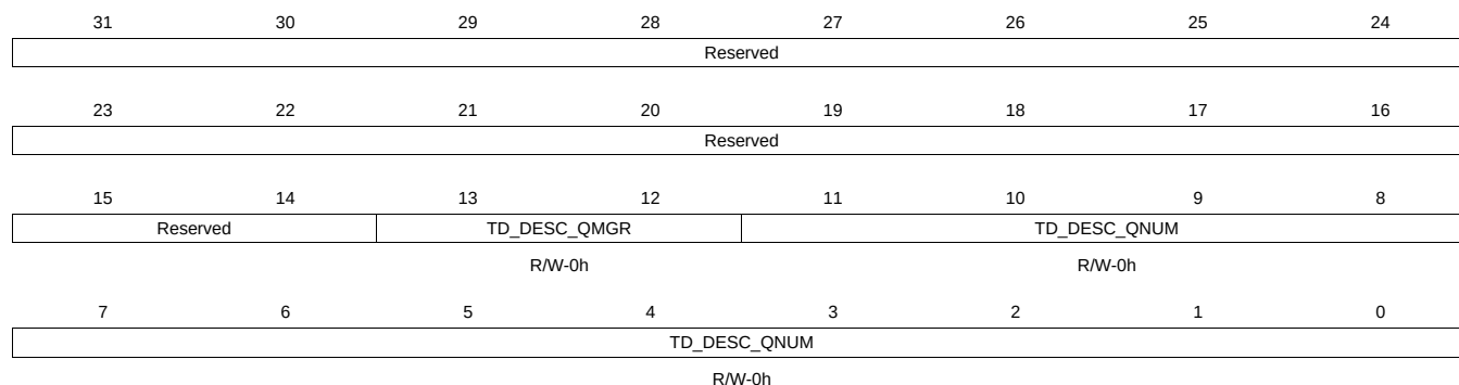
Figure 16-153. TDFDQ Register
