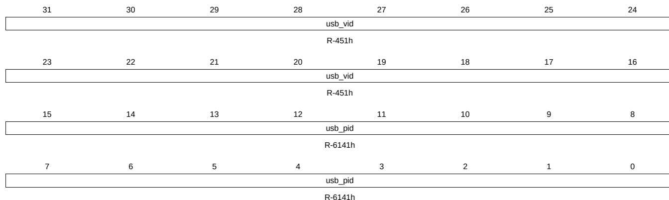
Figure 9-52. usb_vid_pid Register
