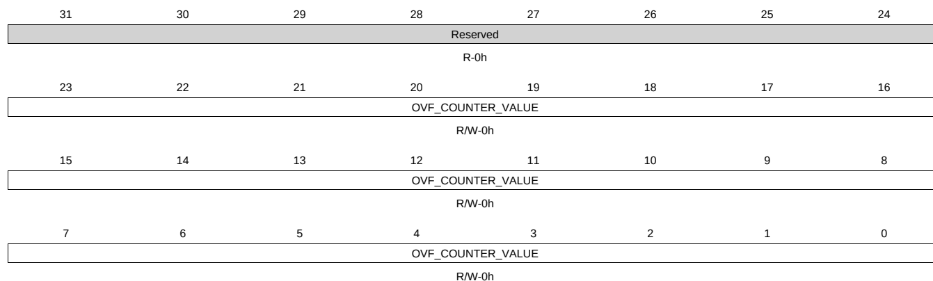
Figure 20-53. TOCR Register
