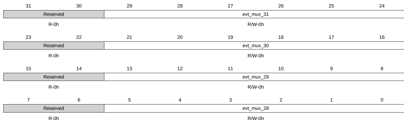
Figure 9-66. tpcc_evt_mux_28_31 Register
