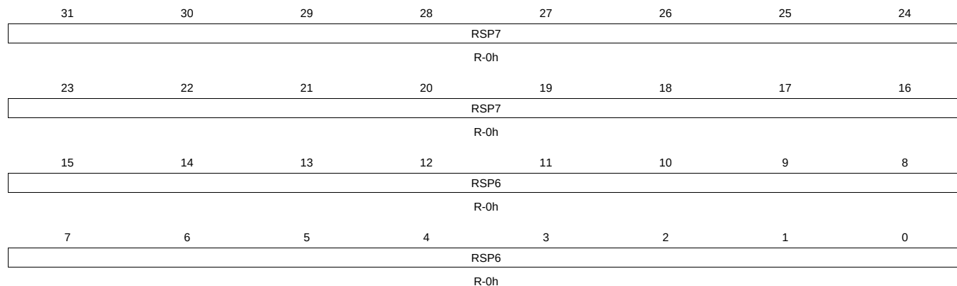
Figure 18-50. SD_RSP76 Register
