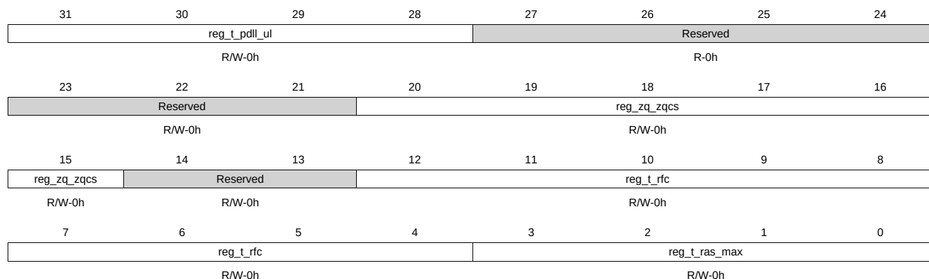
Figure 7-101. SDRAM_TIM_3 Register
