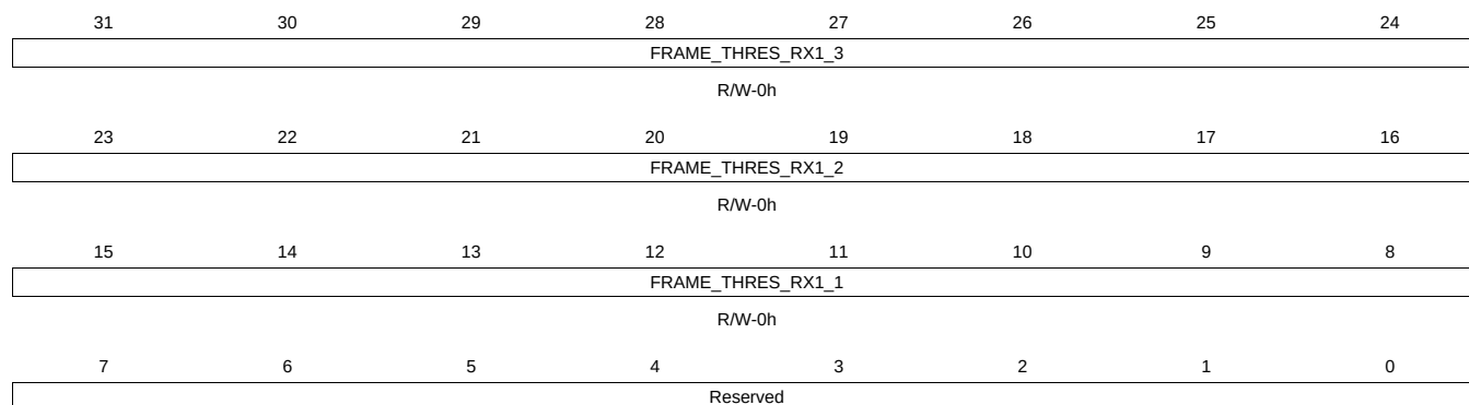
Figure 16-58. IRQFRAMETHOLDRX10 Register
