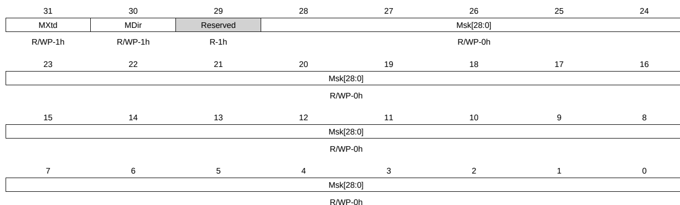
Figure 23-52. IF1MSK Register
