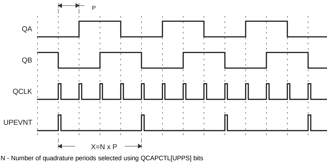
Figure 15-144. Unit Position Event for Low Speed Measurement (QCAPCTL[UPPS] = 0010)
