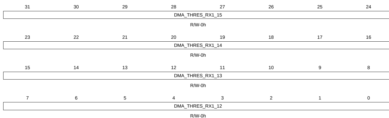
Figure 16-43. IRQDMATHOLDRX13 Register
