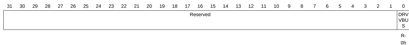
Figure 16-101. USB1STAT Register
