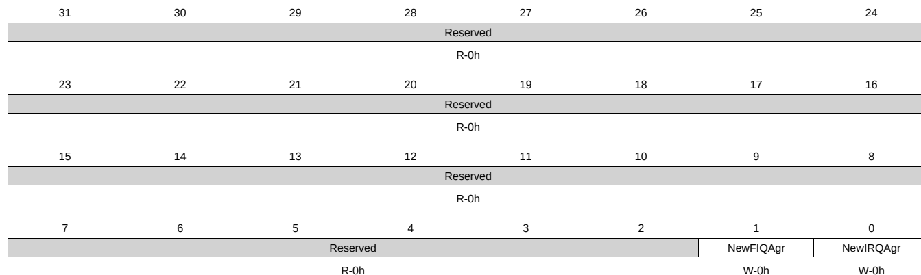
Figure 6-9. INTC_CONTROL Register
