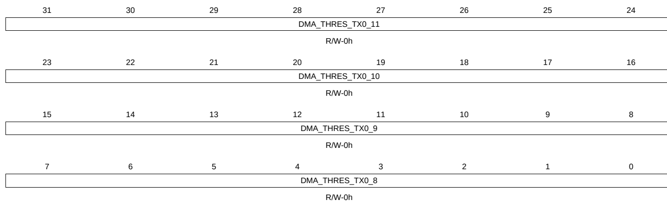
Figure 16-30. IRQDMATHOLDTX02 Register
