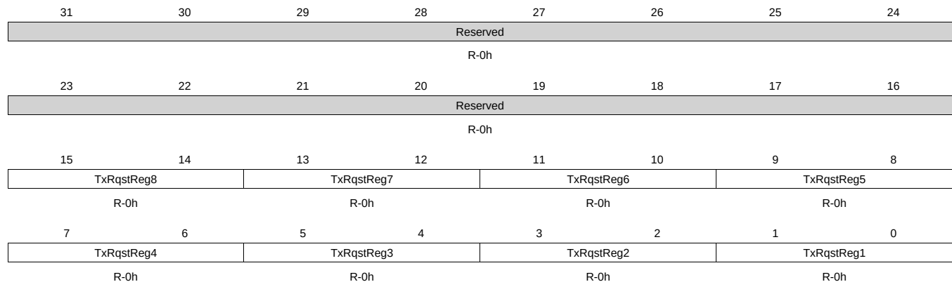
Figure 23-27. TXRQ_X Register
