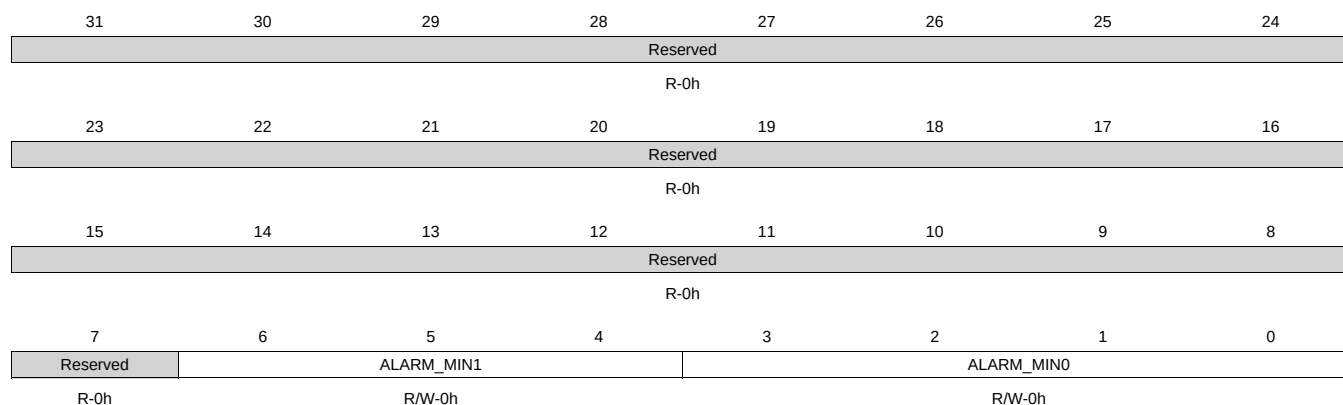
Figure 20-69. ALARM_MINUTES_REG Register
