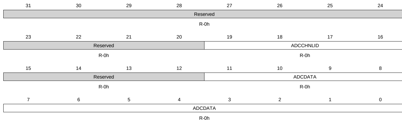
Figure 12-62. FIFO1DATA Register
