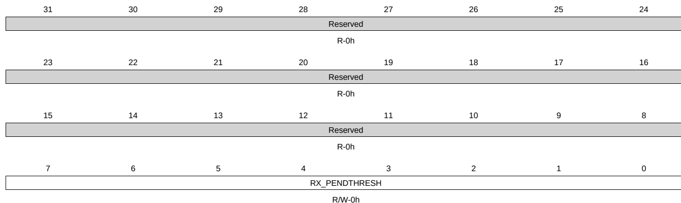
Figure 14-65. RX3_PENDTHRESH Register
