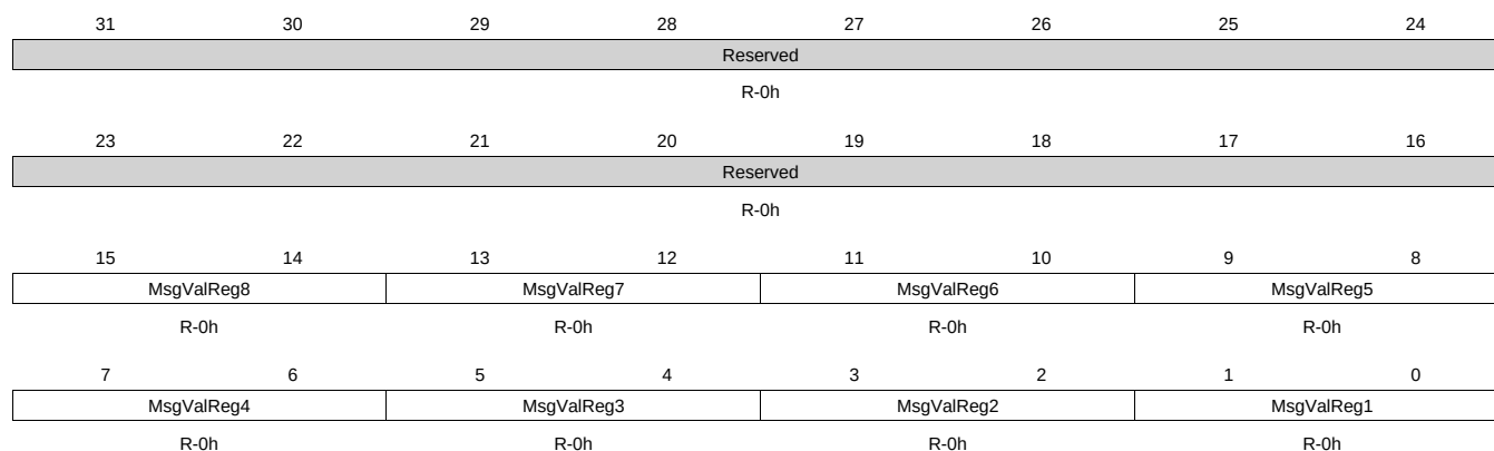
Figure 23-42. MSGVAL_X Register
