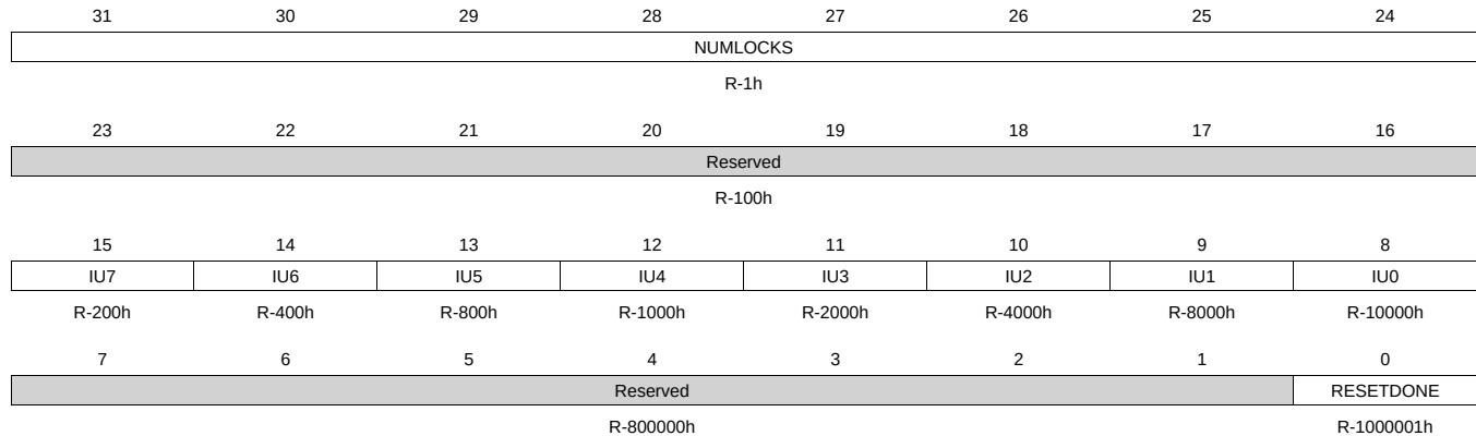
Figure 17-47. SYSTATUS Register
