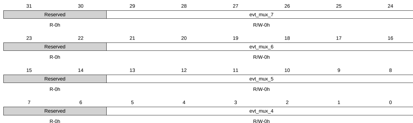
Figure 9-60. tpcc_evt_mux_4_7 Register
