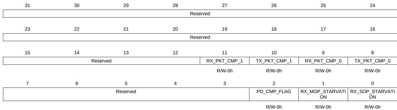
Figure 16-27. IRQCLEARR Register
