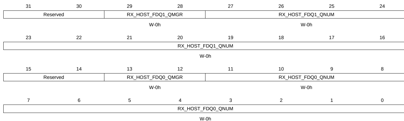
Figure 16-241. RXHPCRA21 Register
