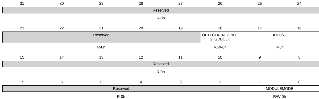
Figure 8-54. CM_PER_GPIO2_CLKCTRL Register
