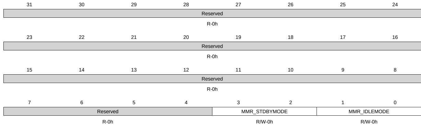
Figure 14-199. CONTROL Register
