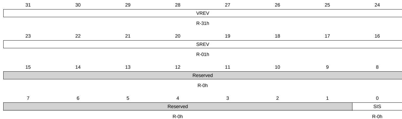
Figure 18-65. SD_REV Register
