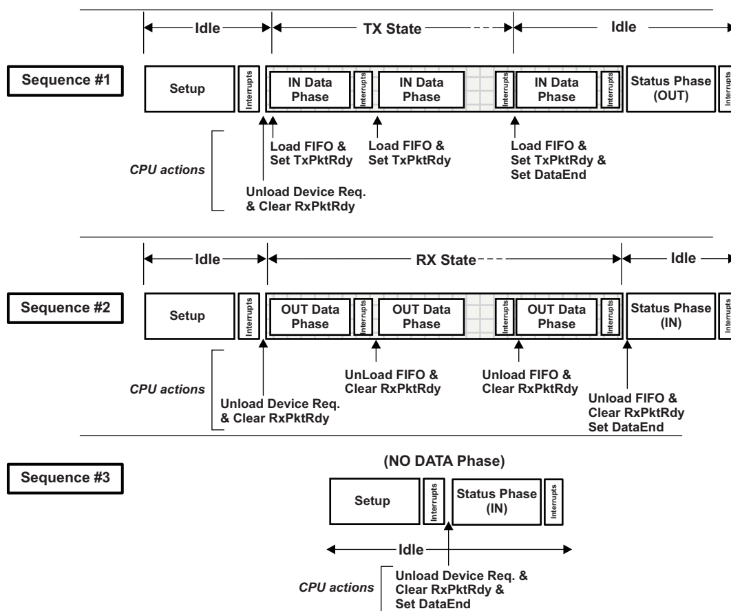
Figure 16-4. Sequence of Transfer
