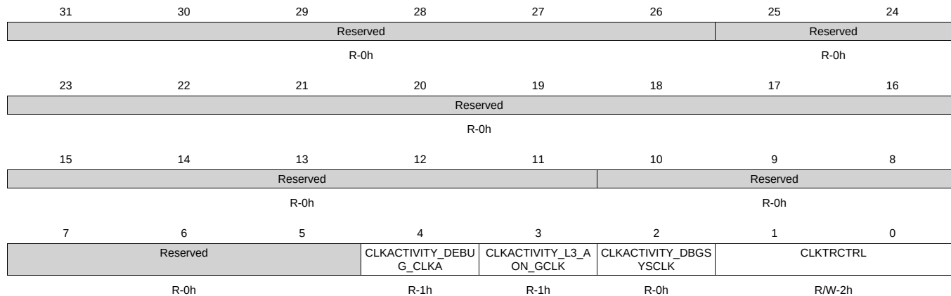
Figure 8-90. CM_L3_AON_CLKSTCTRL Register
