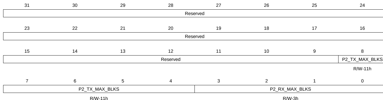
Figure 14-156. P2_MAX_BLKs Register
