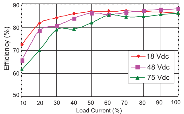
PDQ15-Q48-D15-D Efficiency Curve (Efficiency vs. Line Voltage and Load Current)
