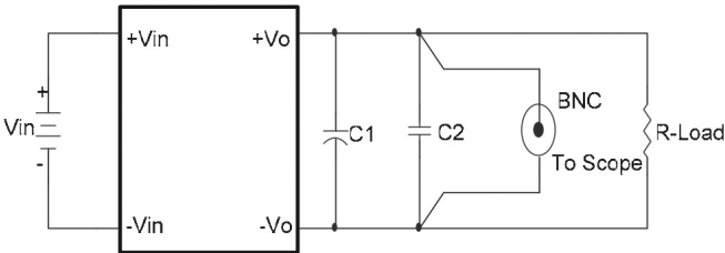
Figure 2 Measuring Output Ripple And Noise
