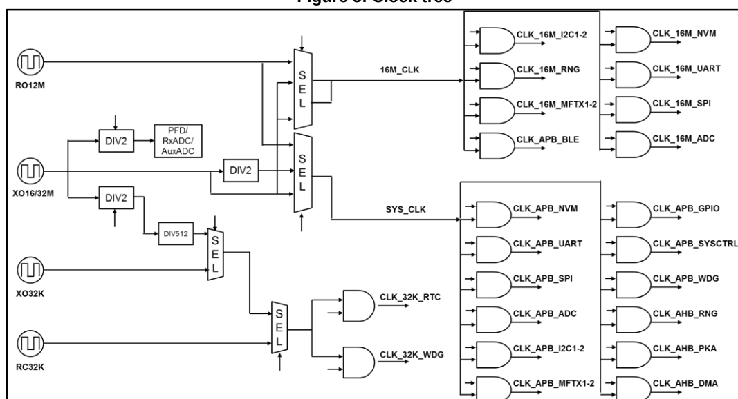
Figure 5: Clock tree
