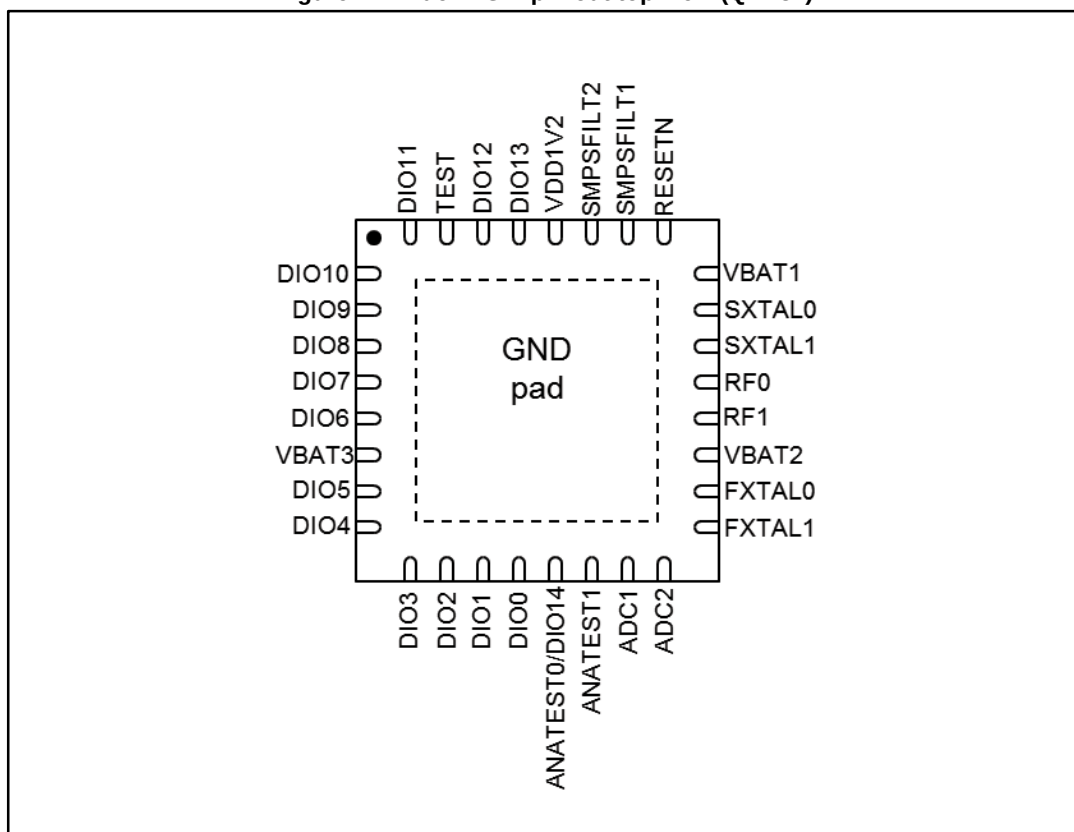
Figure 17: BlueNRG-1 pin out top view (QFN32)
