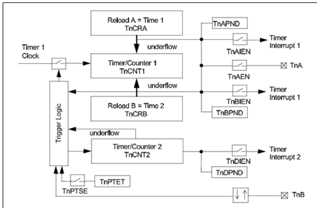
Figure 13: MFT mode 1a block diagram
