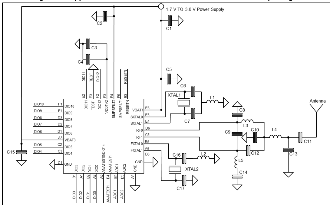
Figure 23: Application circuit: non active DC-DC converter WCSP34 package
