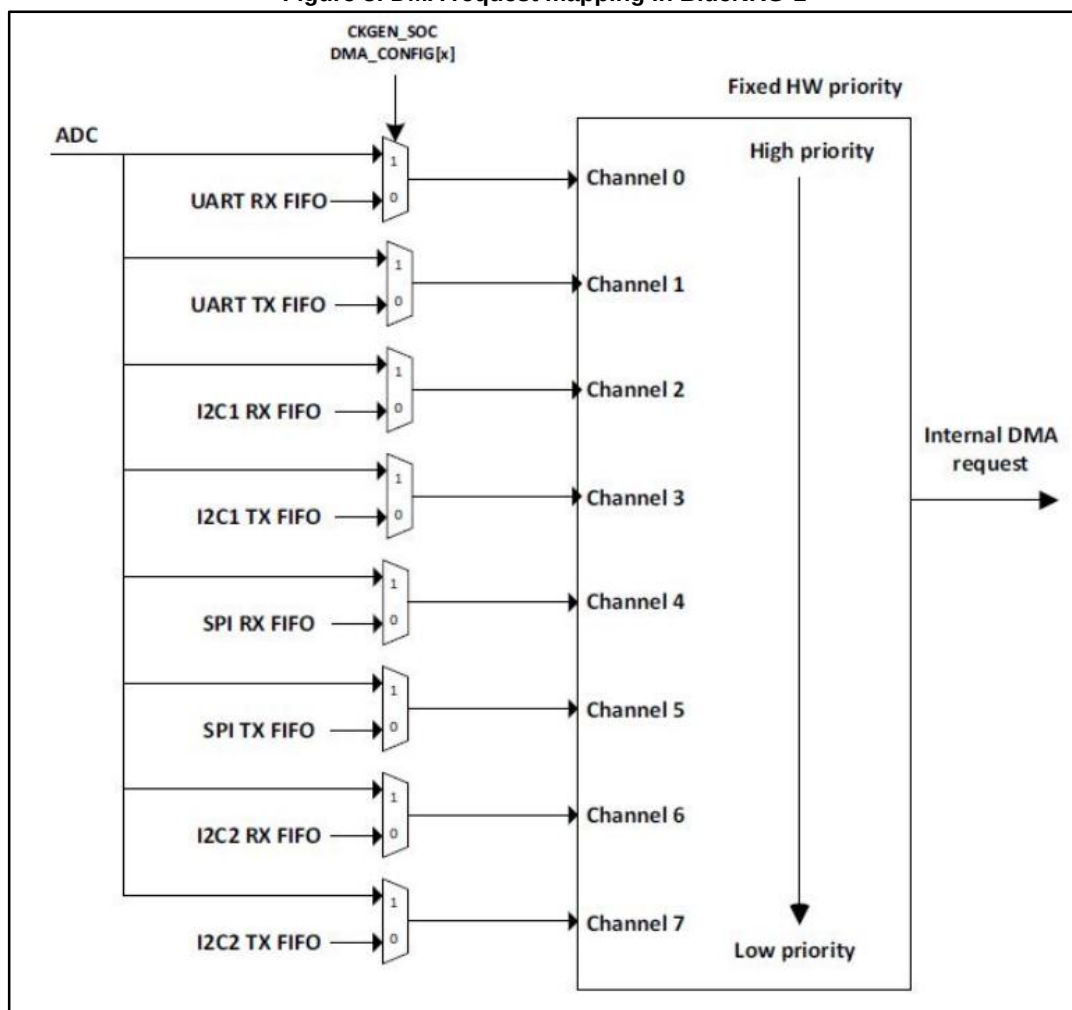
Figure 8: DMA request mapping in BlueNRG-1
