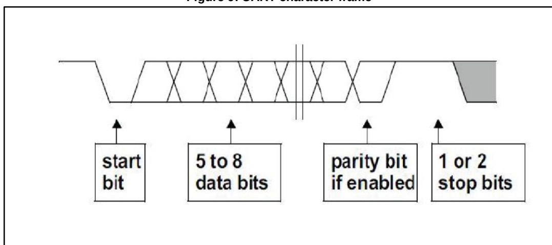
Figure 9: UART character frame
