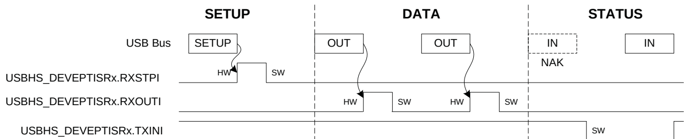
Figure 36-9. Control Write
