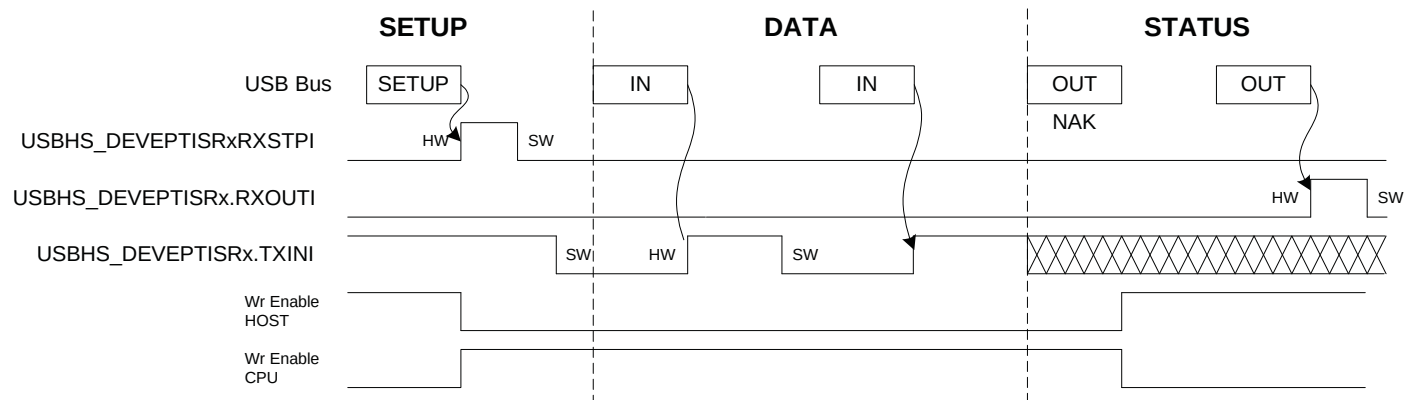
Figure 36-10. Control Read
