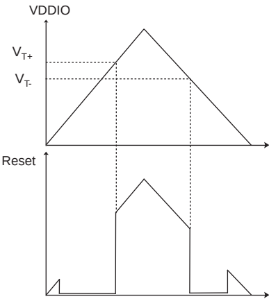
Figure 54-4. VDDIO Power-On Reset Characteristics
