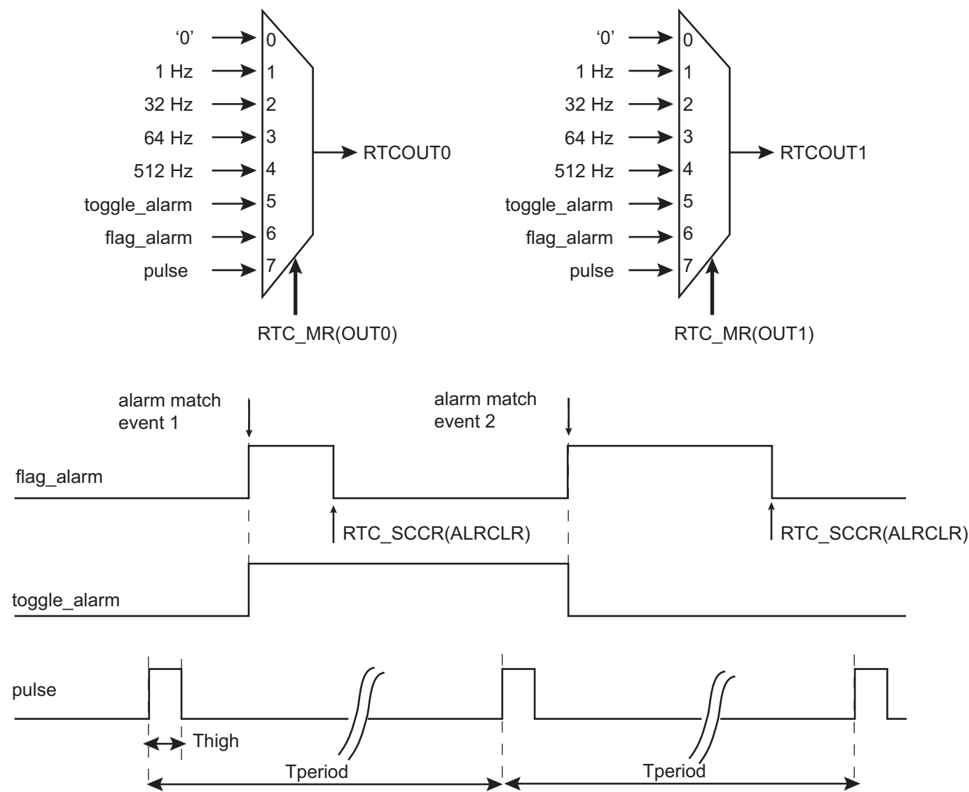
Figure 25-5. Waveform Generation
