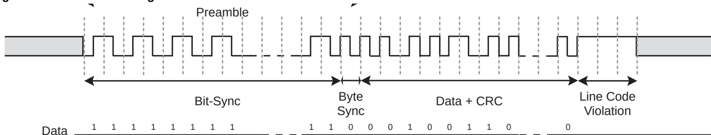
Figure 43-55. LON Framing
