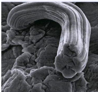
(a) Filament whisker with striations
