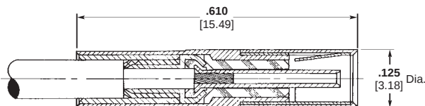
Straight Plug 1 Part Number 142-1000-0001 Instruction Sheet Number 408-08512 Former MICRODOT I.S. Number RF-ASMB-15
