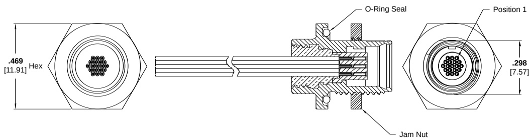
19 Position Drawing Number 1589061
