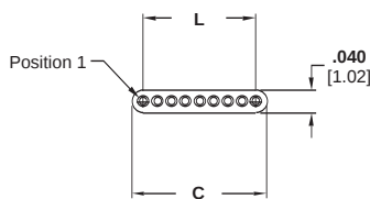
Plug Assembly Drawing Number 1589448
