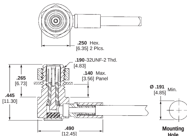
Right-Angle Bulkhead Mount Plug 1 Part Number 142-1021-0001 Instruction Sheet Number 408-08519 Former MICRODOT I.S. Number RF-ASMB-76
