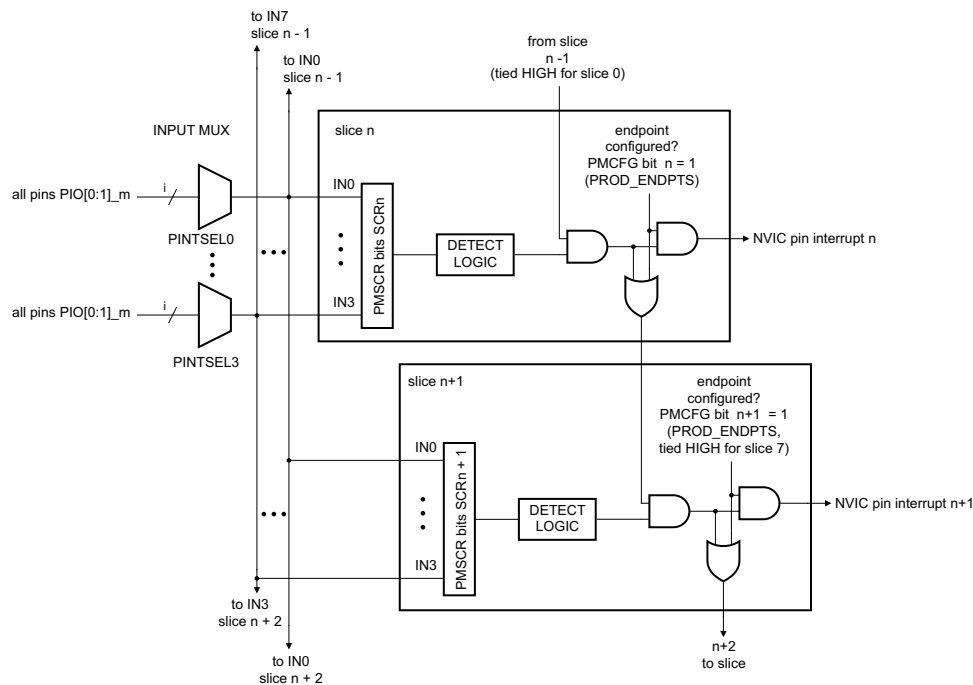
Fig 18. Pattern match engine connections
