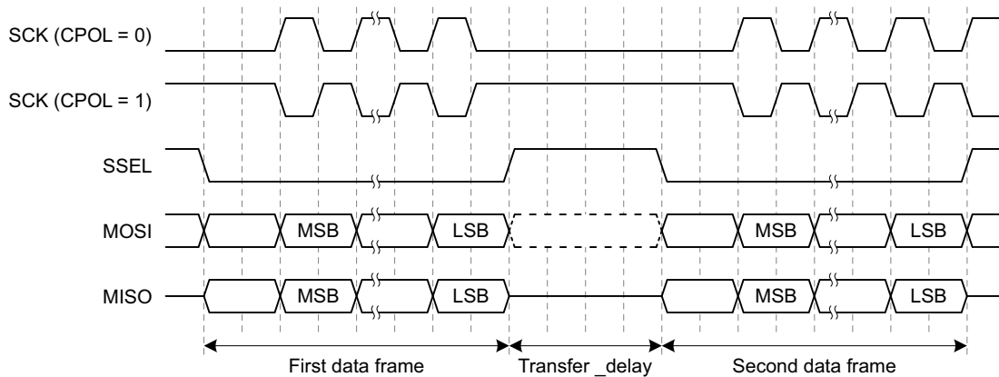
Fig 62. Transfer_delay
