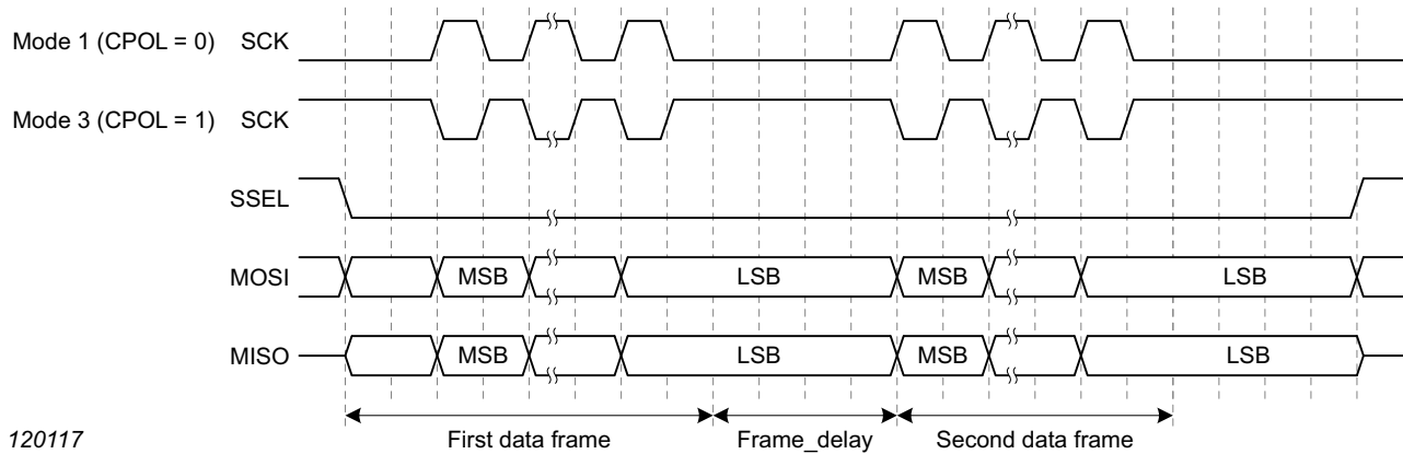
Fig 61. Frame_delay
