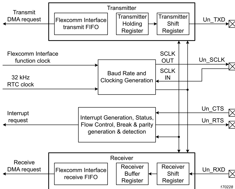
Fig 56. USART block diagram
