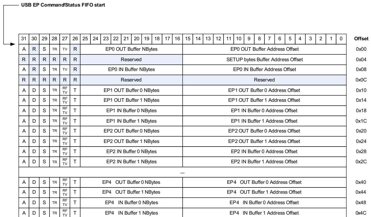
Fig 52. Endpoint command/status list (see also Table 360 )
