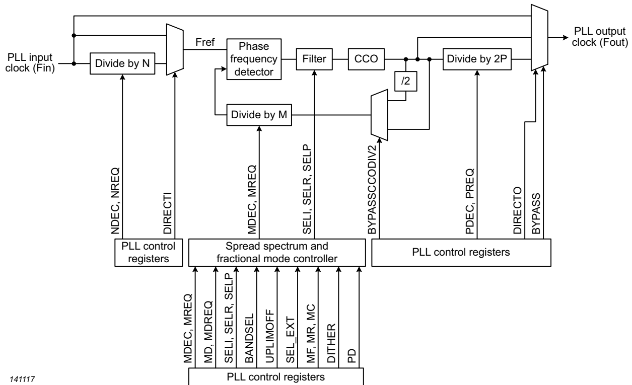
Fig 12. System PLL block diagram showing spread spectrum and fractional divide operation
