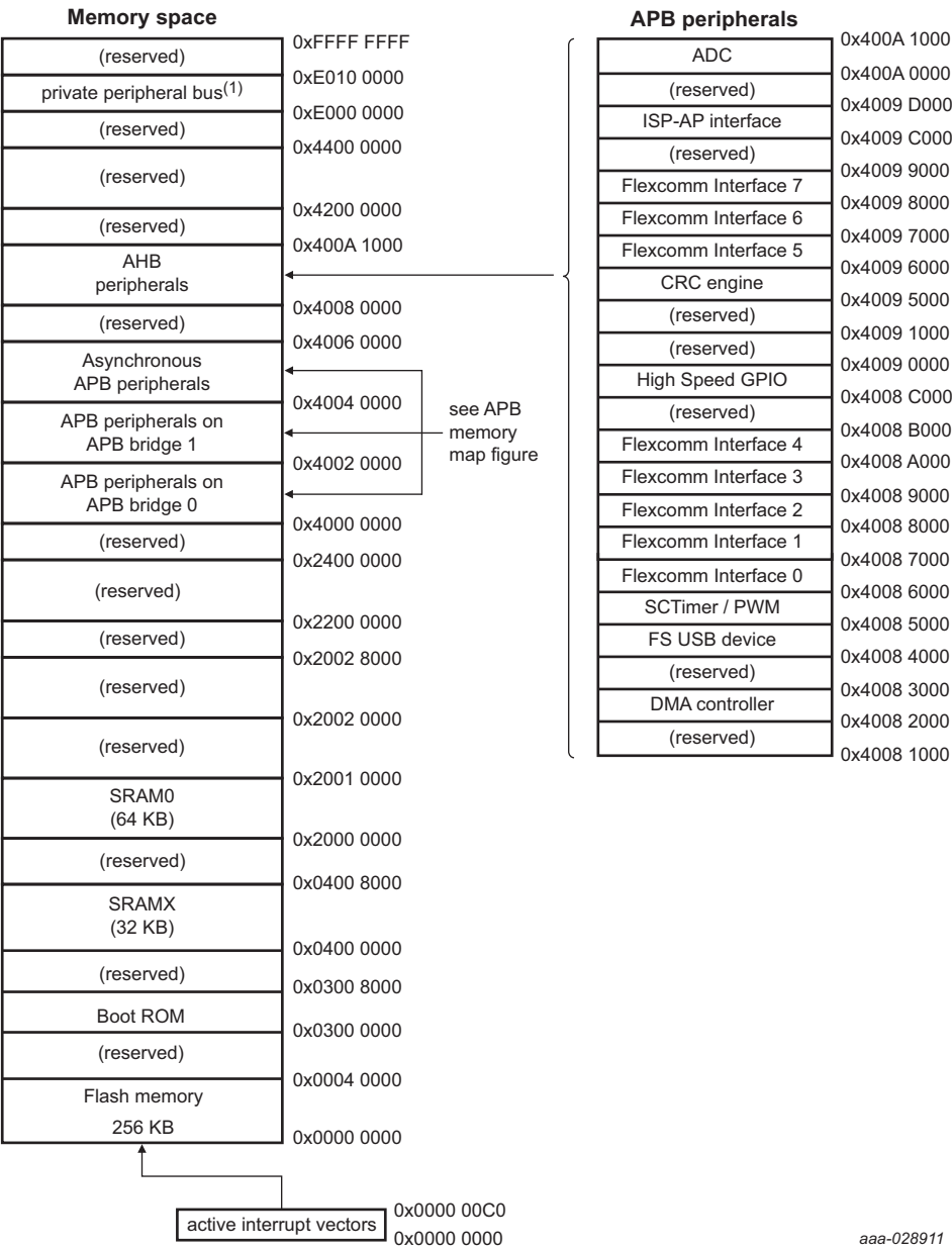
Fig 2. Main memory map
