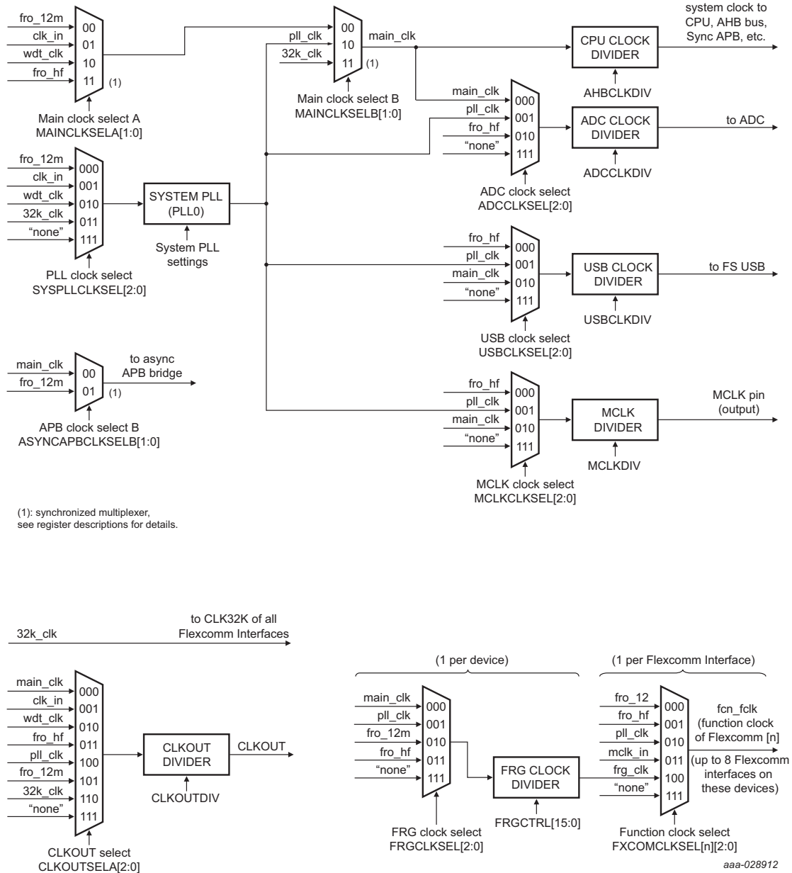
Fig 9. Clock generation
