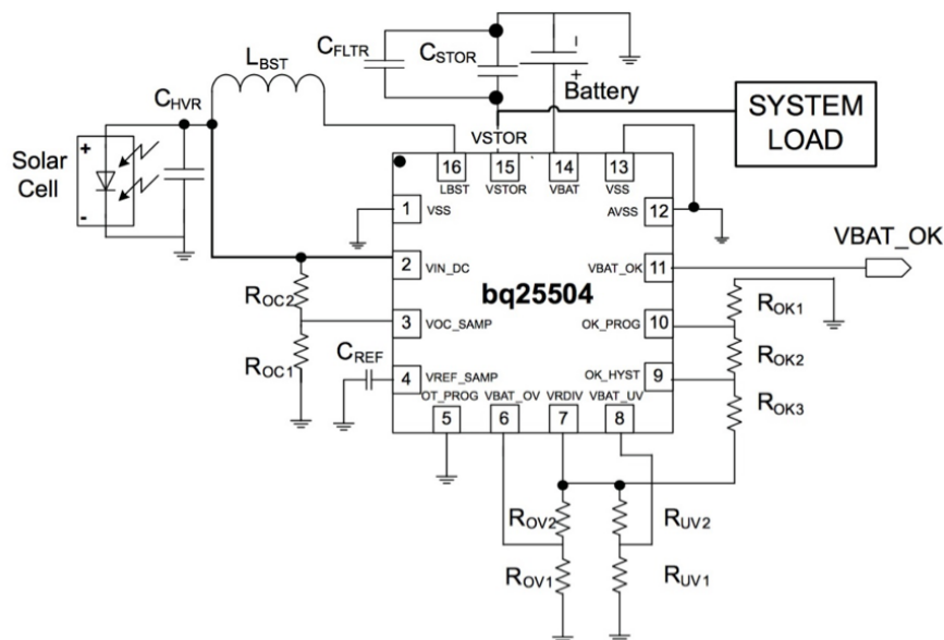
Figure 5: Application circuit for energy-harvested batter charging using TI power management IC. (Source: Texas Instruments)
