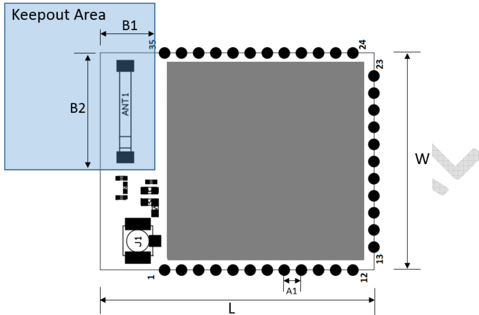
Figure 3: MKW22D Module Physical Dimensions
