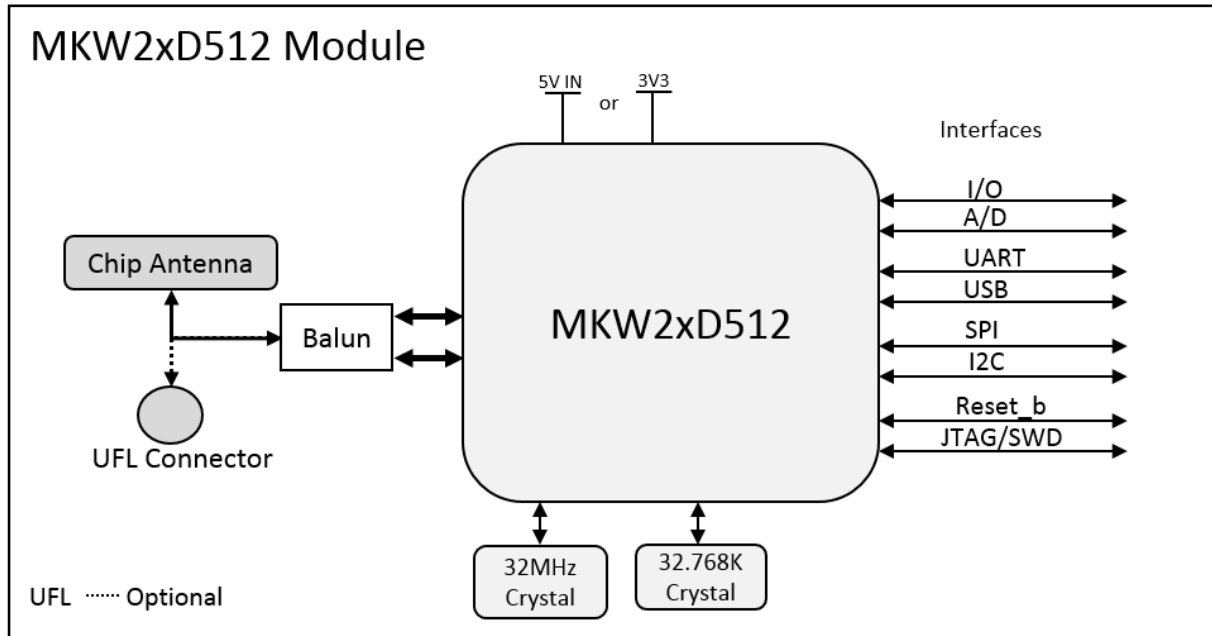
Figure 2: MKW22D Module Hardware Block Diagram
