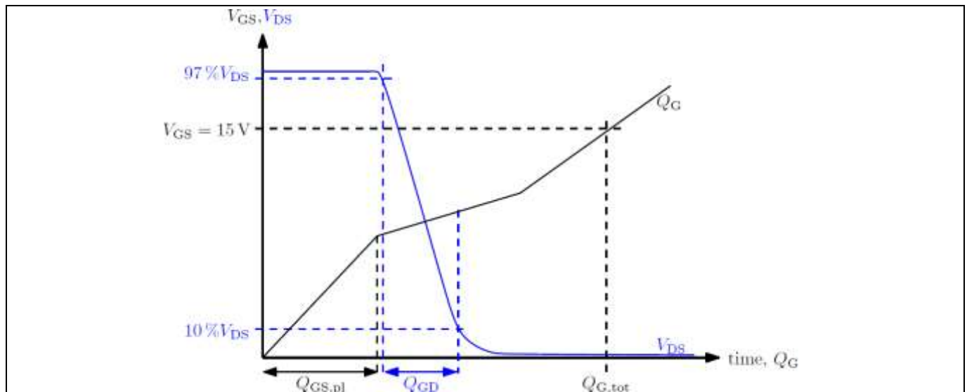
Figure 11 Typical gate charge, V_{GS} = f(Q_G) , I_{DS} = 20\text{ A} , V_{DS} = 800\text{ V} , turn-on pulse
