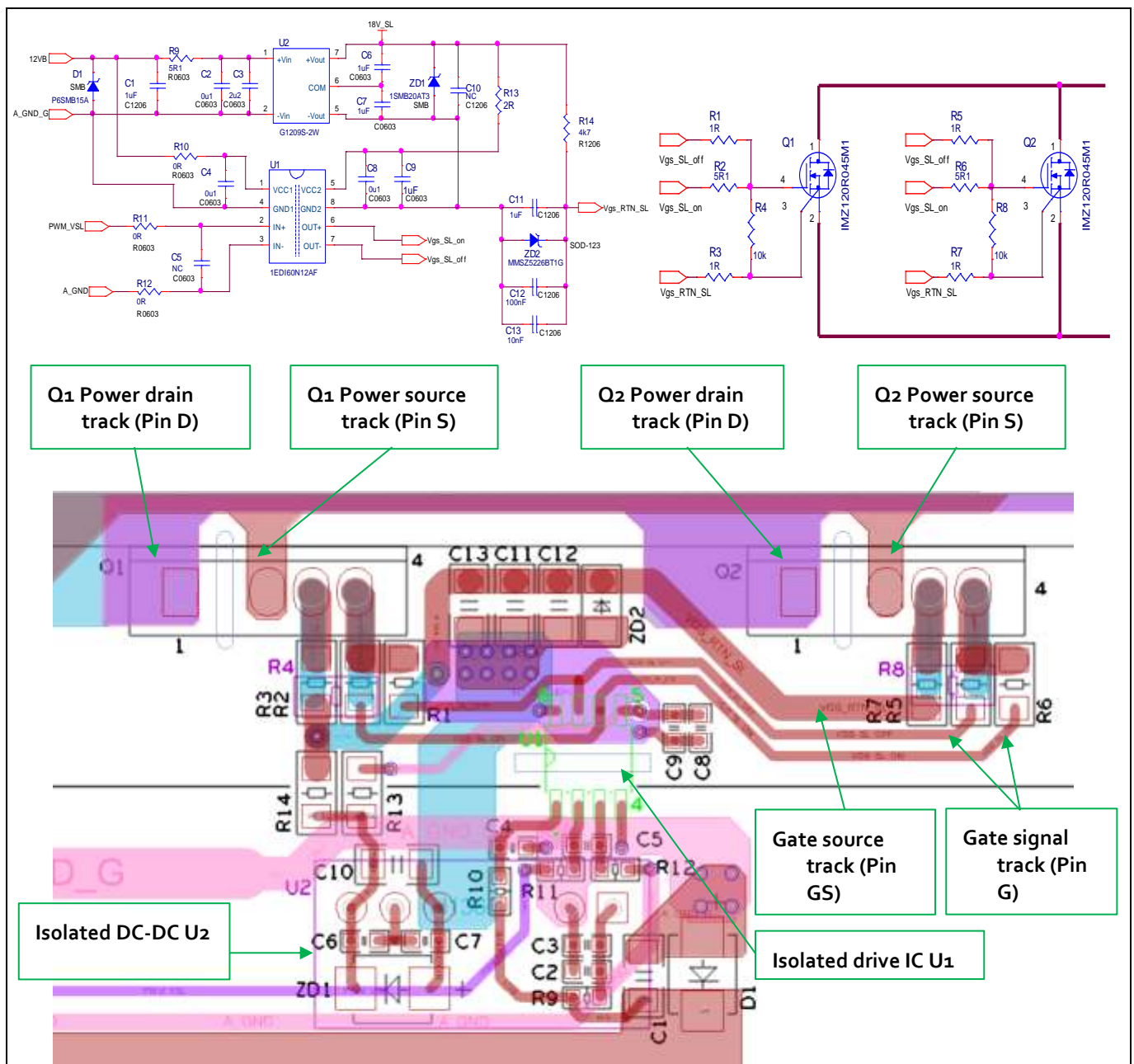
Figure 13 A drive circuit and PCB layout example of 2 units IMZ120R045M1 with TO-247 4pin package
