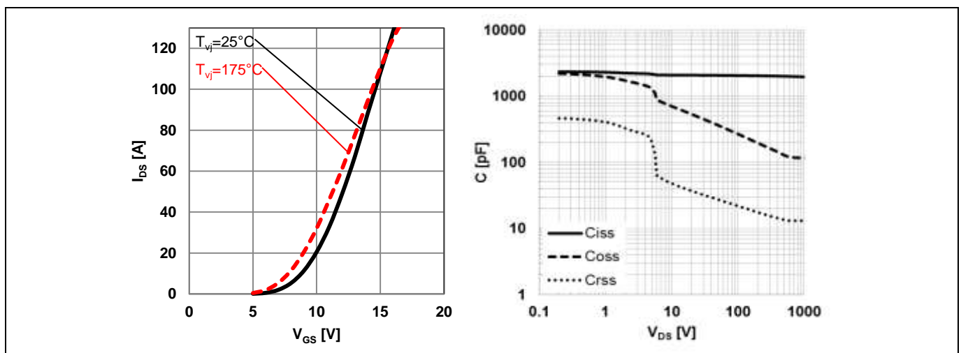
Figure 4 (left) Typical transfer characteristics ( V_{DS}=20 V); (right) Typical capacitance as a function of drain-source voltage
