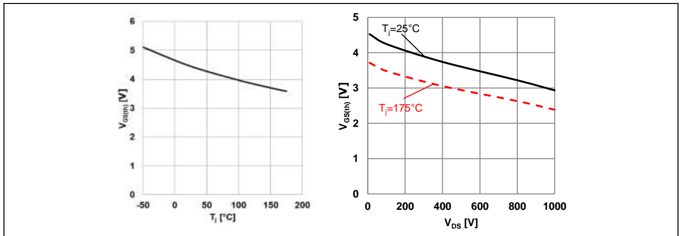
Figure 3 (left) Typical gate-source threshold voltage as a function of junction temperature ( I_{DS}=10 mA, V_{GS}=V_{DS} ); (right) Typical gate-source threshold voltage as a function of drain-source voltage ( I_{DS}=10 mA)
