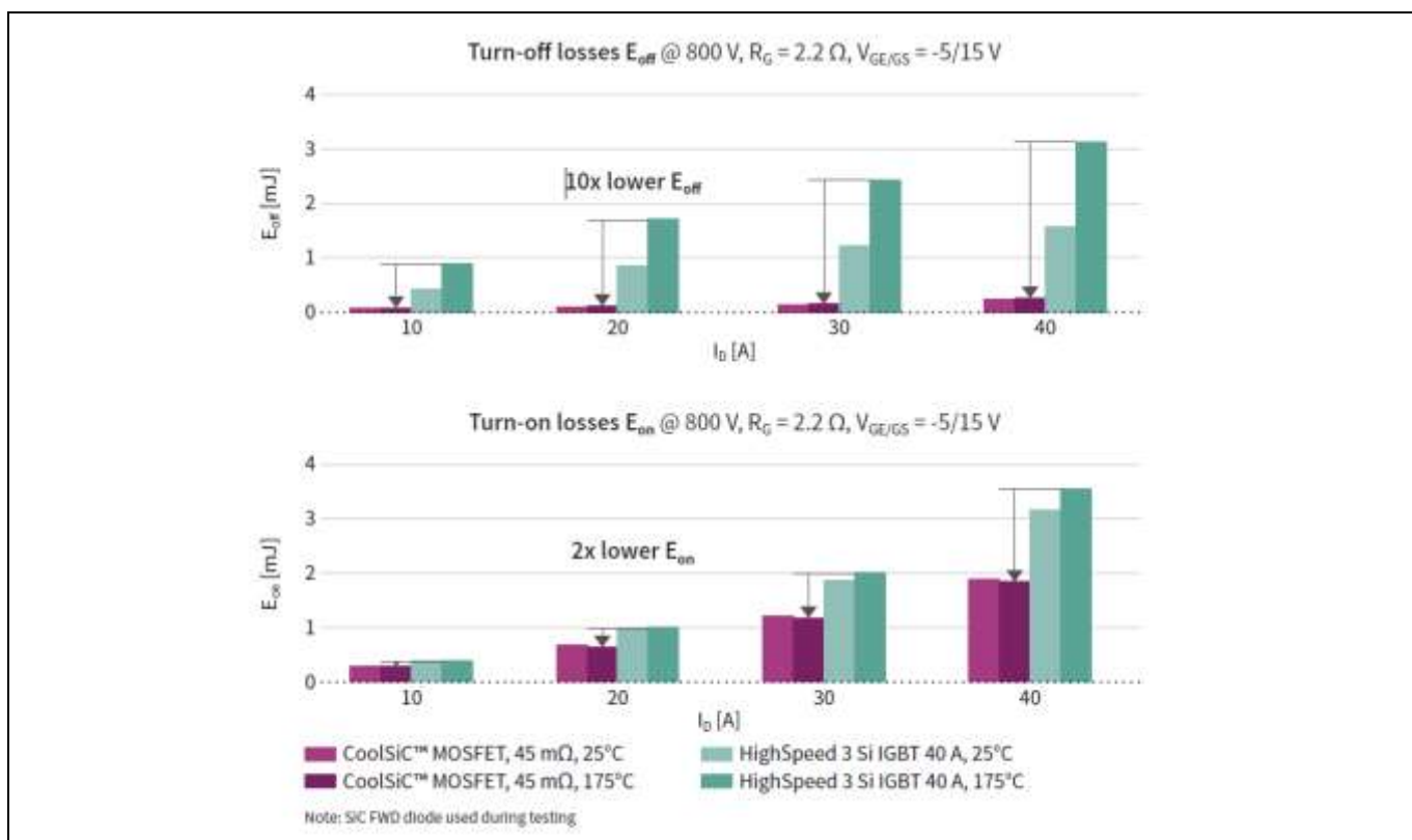
Figure 14 Switching E_{off} and E_{on} comparison between 1200 V H 3 IGBT and CoolSiC™ MOSFET
