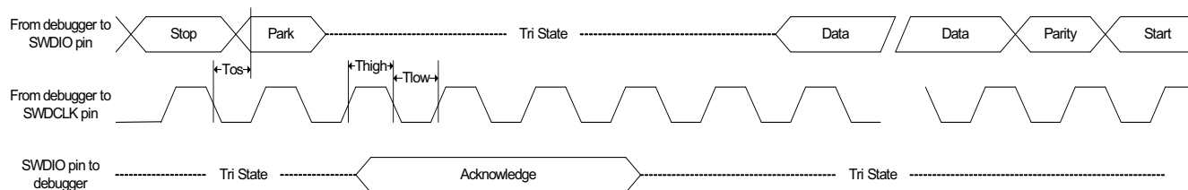
Figure 42-17.SWD Interface Signals
