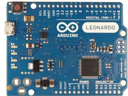
Arduino Leonardo Front without headers
