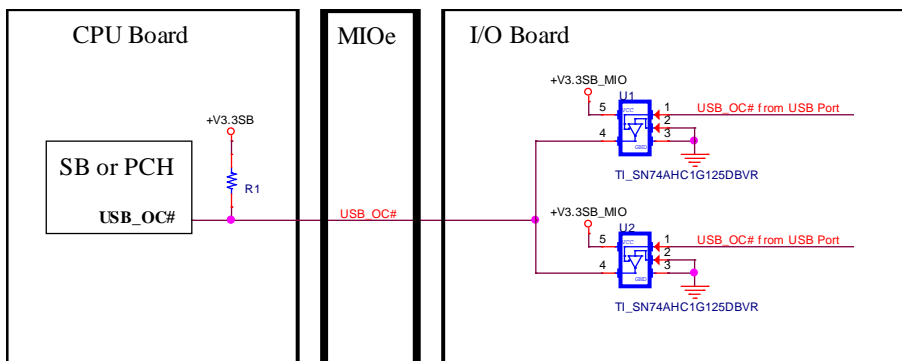
Figure 2.6-1 Demonstration for USB over current sensing
