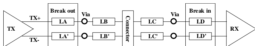
Figure 2.7-4 length matching example
