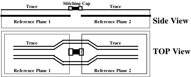
Figure 2.7-1 Trace Crossing Plane Splits
