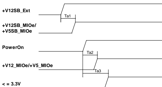
Figure 3.5-2 I/O board power-on sequence
