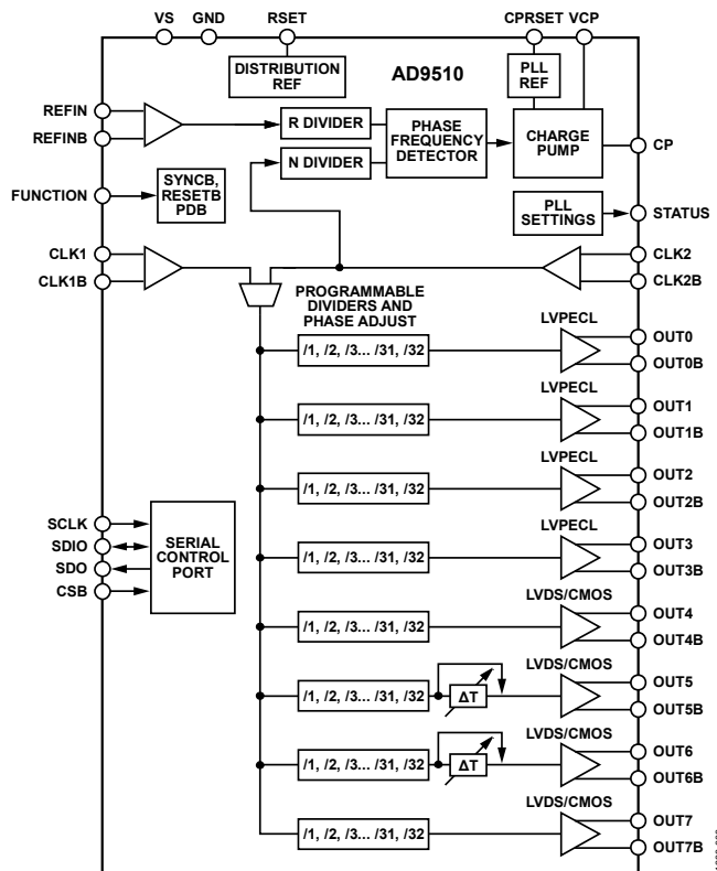
Figure 9. AD9510 Clock Synthesis and Distribution
