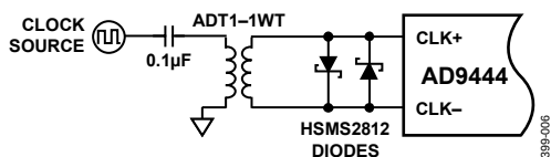
Figure 6. Distribution and Differential Encode Options
