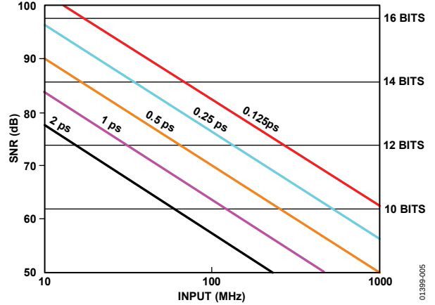
Figure 5. Signal-to-Noise Ratio Due to Aperture Jitter
