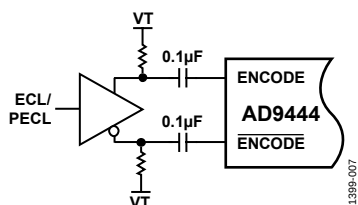
Figure 7. Active Differential Drive Circuit
