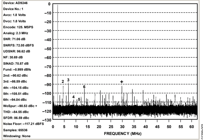
Figure 3. 2.3 MHz FFT
