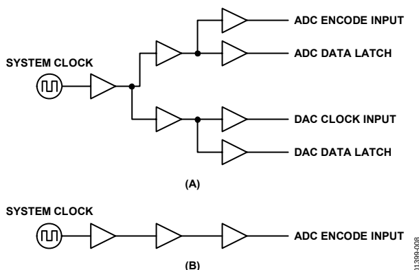
Figure 8. Clock Distribution Chains
