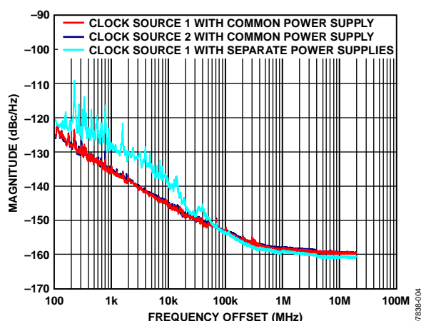
Figure 4. Residual Phase Noise Measurement Displays the Impact from Common and Separate Power Supplies
