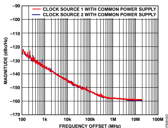
Figure 3. Residual Phase Noise Measurement with Virtually No Impact from Either Clock Source in Figure 2
