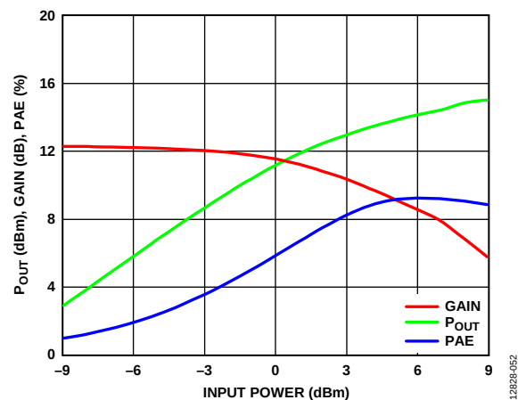
Figure 26. Power Compression @ 18 GHz
