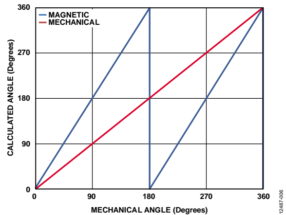
Figure 7. Magnetic vs. Mechanical Angle
