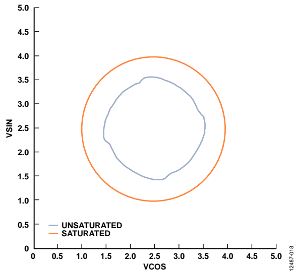
Figure 17. Radius of Unsaturated and Saturated Sensors
