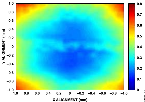
Figure 14. SmCo (24MGOe) with 6 mm Air Gap
