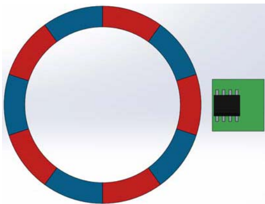
Figure 2. Off Shaft Magnet Configuration
