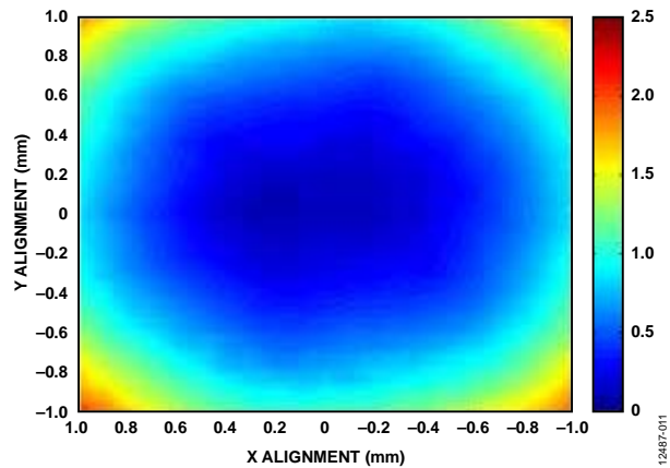
Figure 11. NdFeB (35 MGOe) with 1 mm Air Gap
