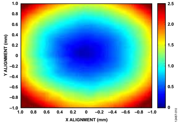
Figure 10. SmCo (32MGOe) with 1 mm Air Gap
