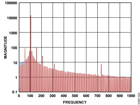
Figure 19. FFT of Misaligned Sensor
