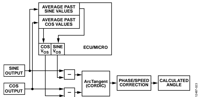
Figure 22. Single Point Calibration Operating Flow Chart
