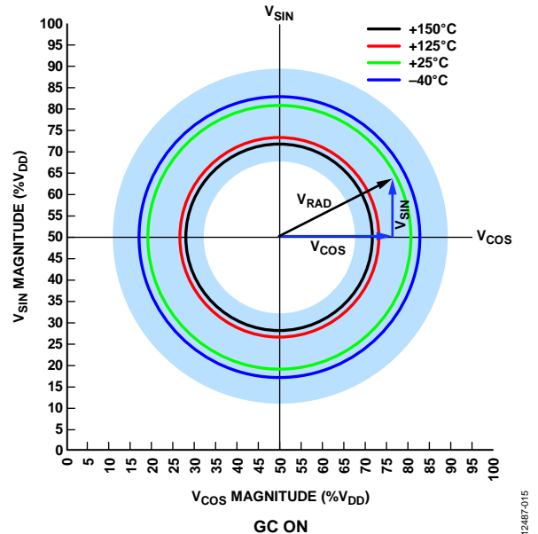
Figure 15. Bounded Radius with GC On
