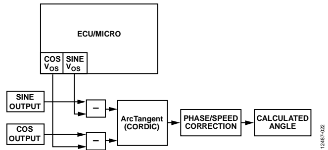
Figure 21. Dynamic Calibration Operating Flow Chart
