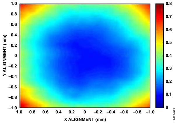
Figure 13. SmCo (24MGOe) with 4 mm Air Gap
