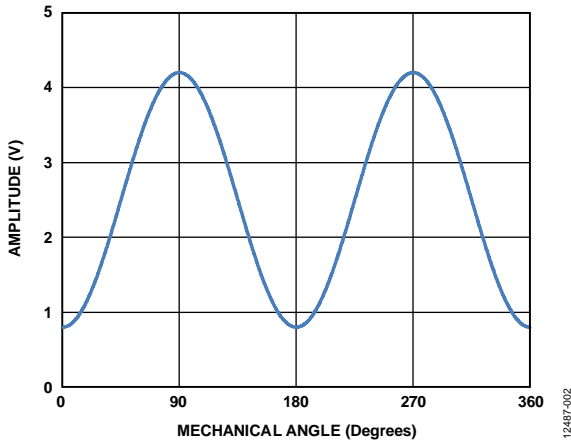
Figure 4. Single Bridge Output
