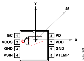
Figure 9. Defined Alignment Directions Relative to the ADA4571 Package
