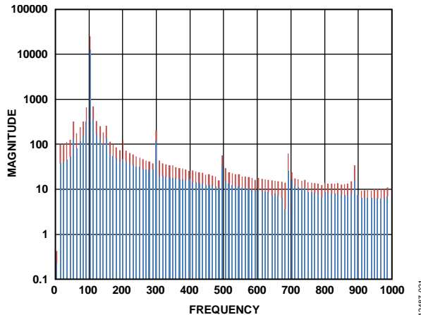
Figure 20. FFT of Unsaturated Sensor
