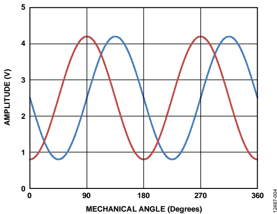
Figure 6. Two Bridge Output
