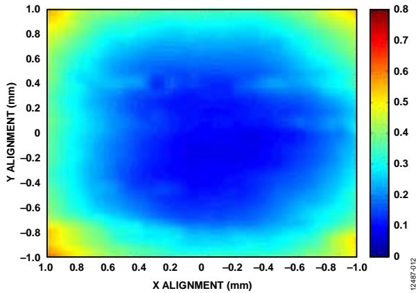
Figure 12. SmCo (24MGOe) with 2 mm Air Gap
