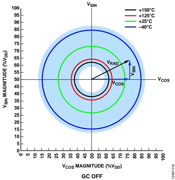
Figure 16. Bounded Radius with GC Off
