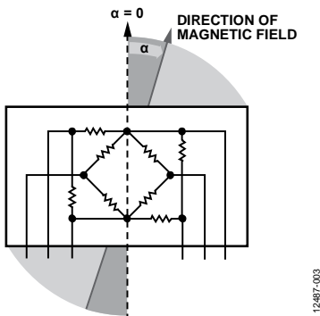
Figure 5. Simplified Circuit Diagram for Double Wheatstone Bridge Sensor
