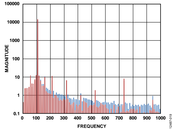
Figure 18. FFT of Well Aligned Sensor
