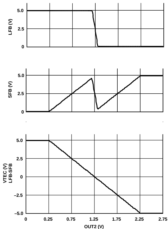
Figure 21. OUT2 Voltage vs. TEC Voltage
