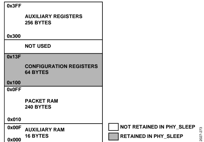
Figure 40. Memory Map
