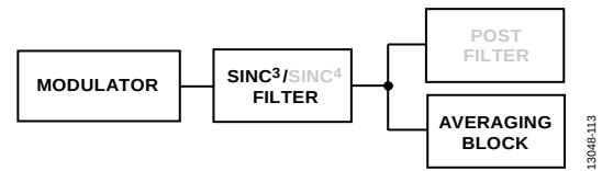
Figure 103. Fast Settling Mode, Sinc 3 + Sinc 1 Filter
