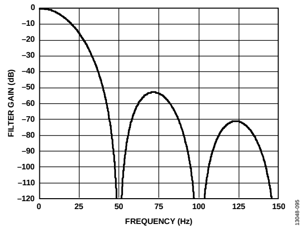
Figure 85. Sinc 4 Filter Response (50 SPS Output Data Rate, Zero Latency Disabled or 12.5 SPS Output Data Rate, Zero Latency Enabled)
