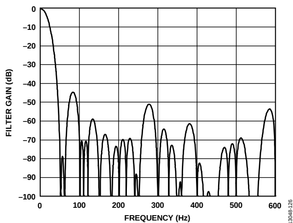
Figure 116. DC to 600 Hz, 16.667 SPS Output Data Rate, 60 ms Settling Time
