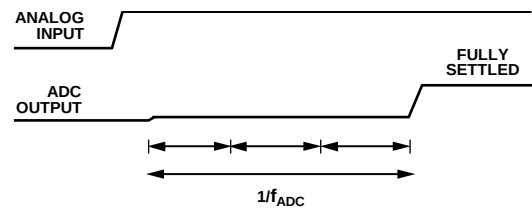
Figure 92. Sinc 3 Zero Latency Operation
