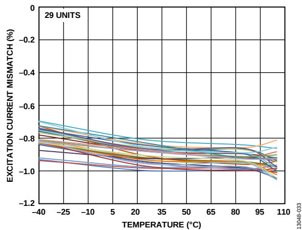
Figure 33. Excitation Current Drift Matching (500 \mu A)
