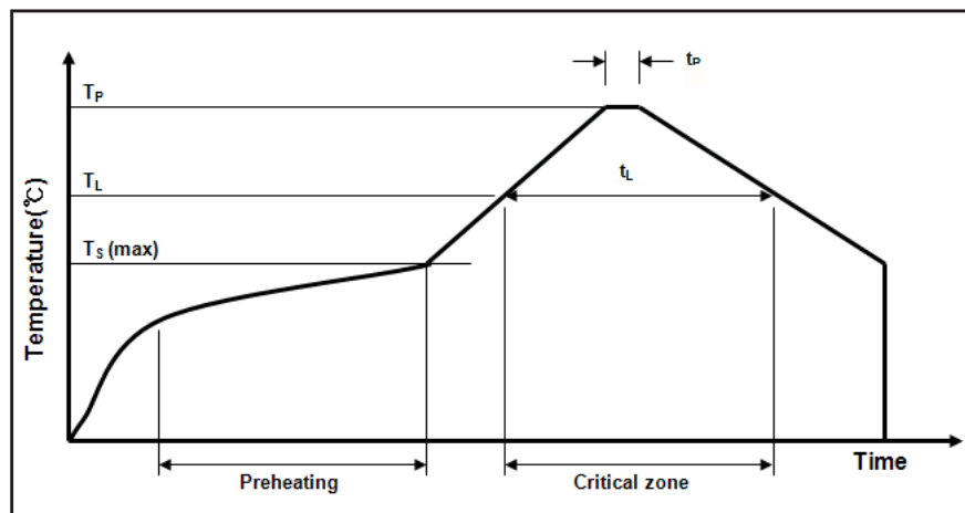
Figure 2: Soldering Profile
