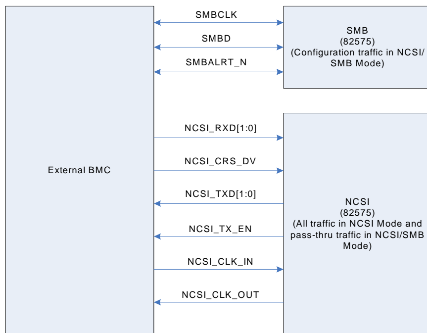
Figure 3. External BMC Connections with NC-SI and SMB
