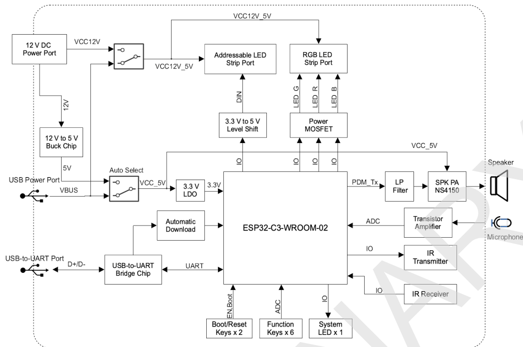
ESP32-C3-Lyra Block Diagram (click to enlarge)
