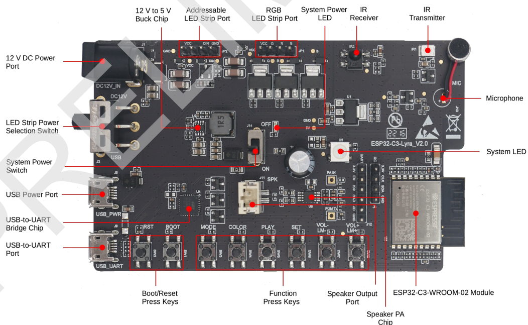
ESP32-C3-Lyra - front (click to enlarge)
