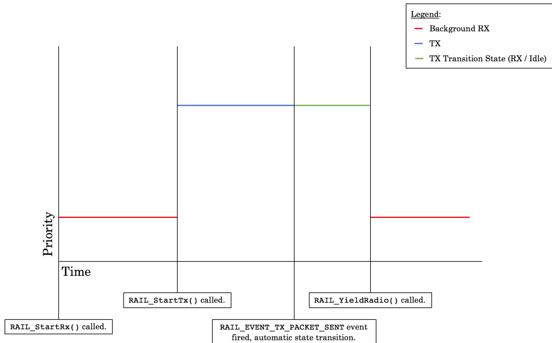
Figure 6.1. State Transitions with Calls to RAIL_StartTx() , RAIL_StartRx() , RAIL_YieldRadio() with a Single Protocol
