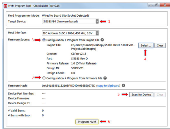
Figure 4.18. Programming In-system, Firmware Based Devices
