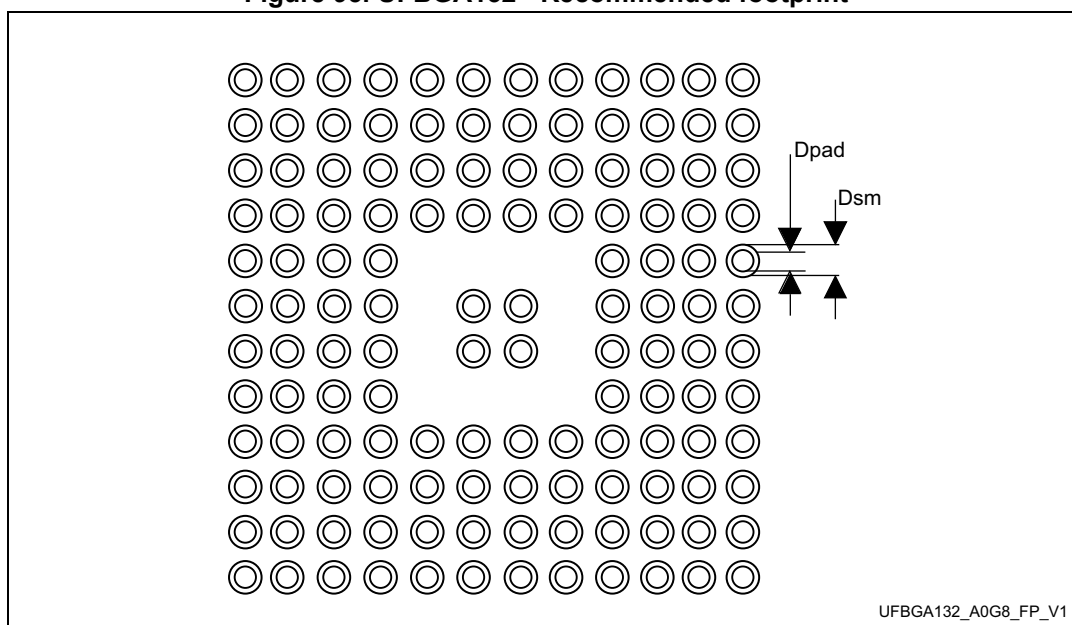
Figure 95. UFBGA132 - Recommended footprint
