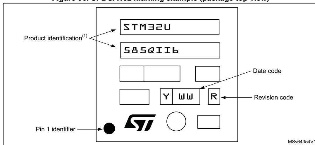
Figure 96. UFBGA132 marking example (package top view)
