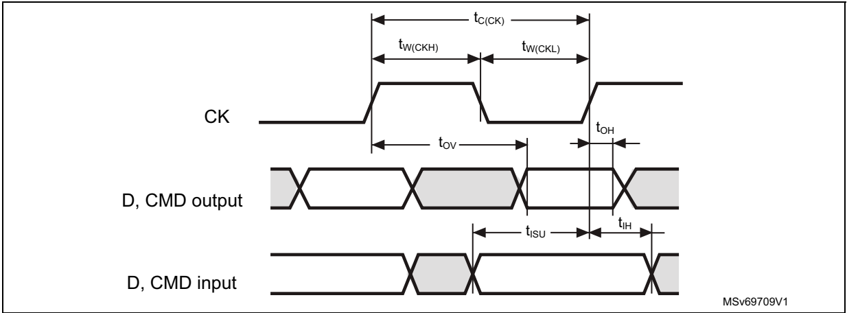
Figure 67. SD high-speed mode
