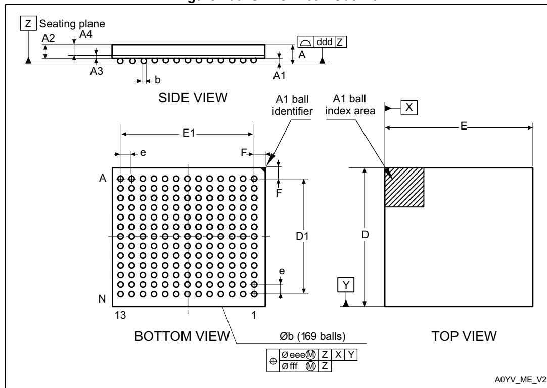
Figure 100. UFBGA169 - Outline
