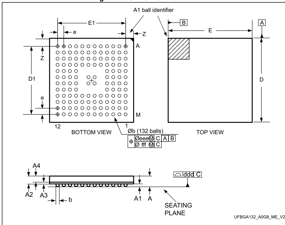
Figure 94. UFBGA132 - Outline
