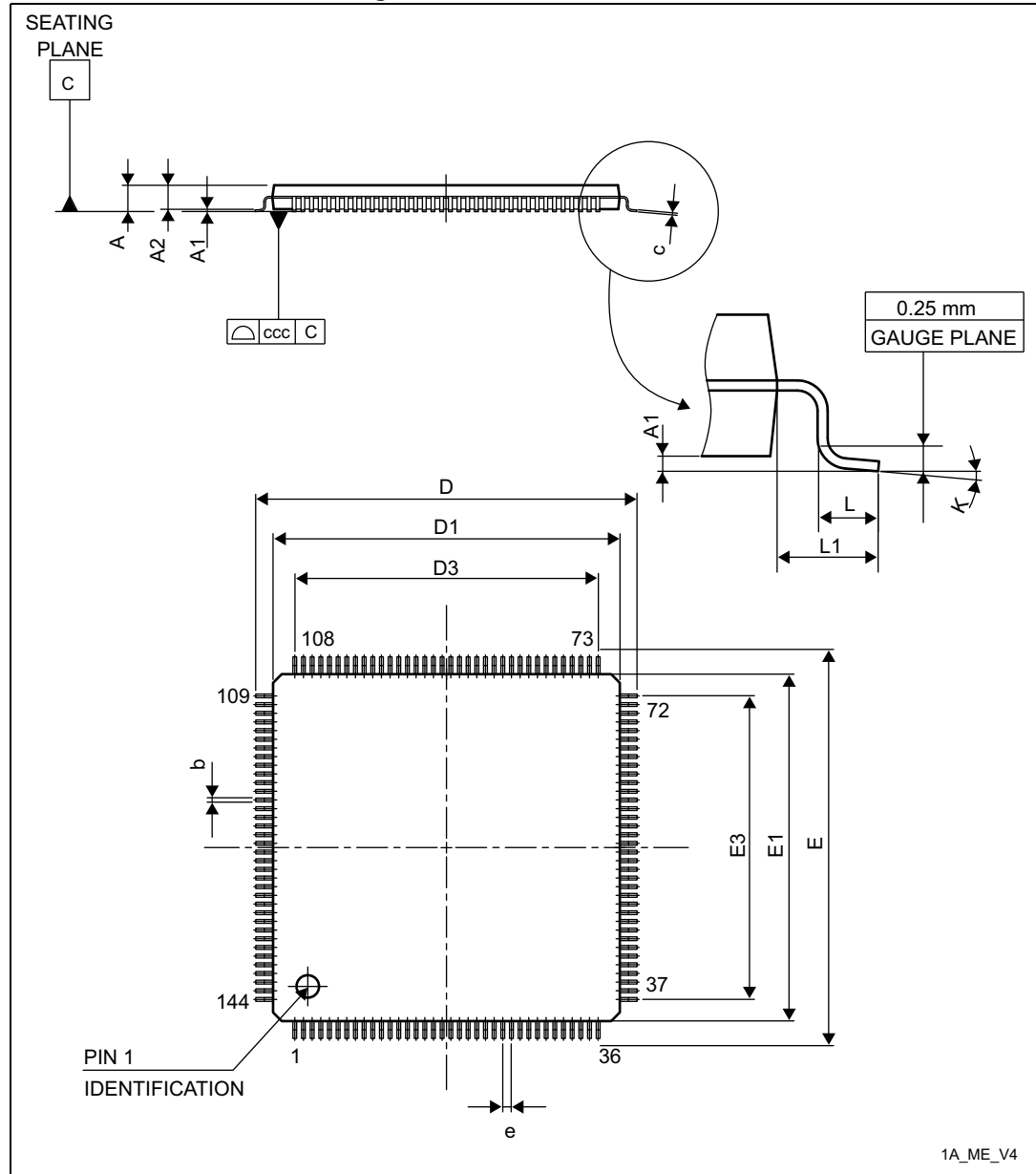
Figure 97. LQFP144 - Outline
