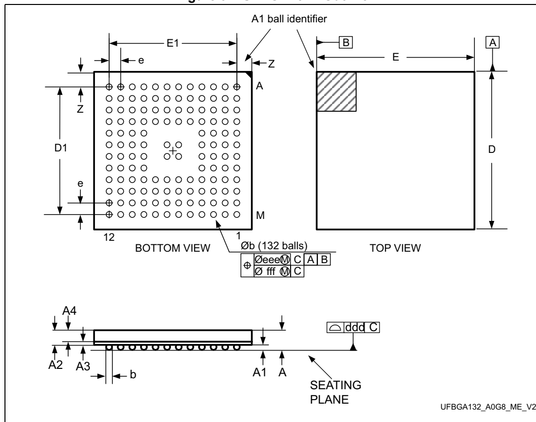
Figure 94. UFBGA132 - Outline
