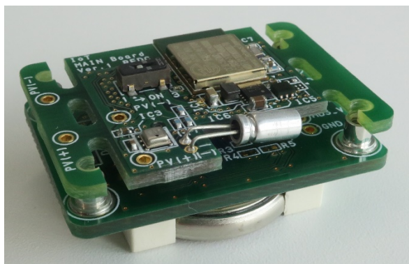
Picture: Connection with the RIOT-001 (The lower board is the RIOT-C01.)
