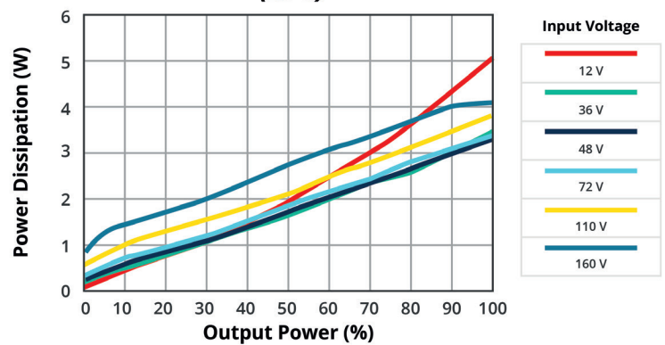
POWER DISSIPATION VS OUTPUT POWER PRFE20W-072-S5-D (25°C)
