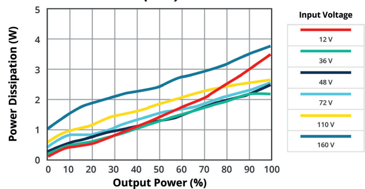
POWER DISSIPATION VS OUTPUT POWER PRFE20W-072-S12-D (25°C)
