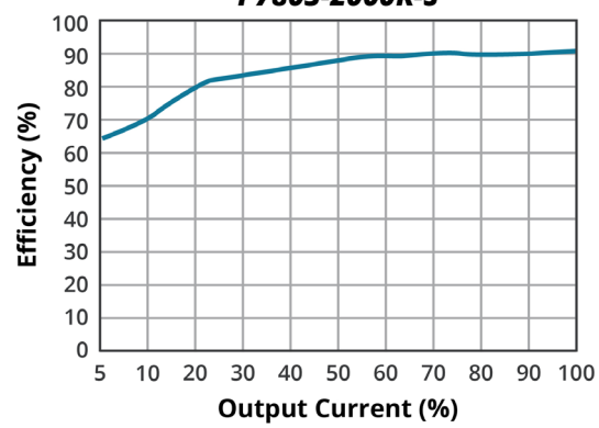
EFFICIENCY VS OUTPUT CURRENT ( V_{in} = 24V ) P7805-2000R-S
