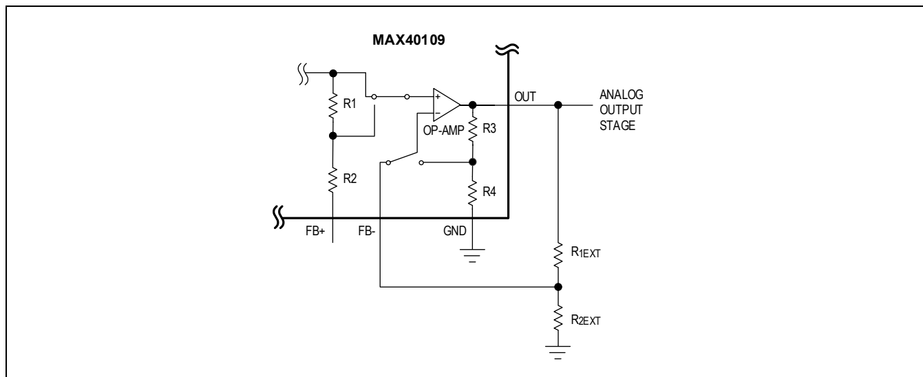
Figure 26. Ratio-Metric Voltage Output with External Resistors Setting
