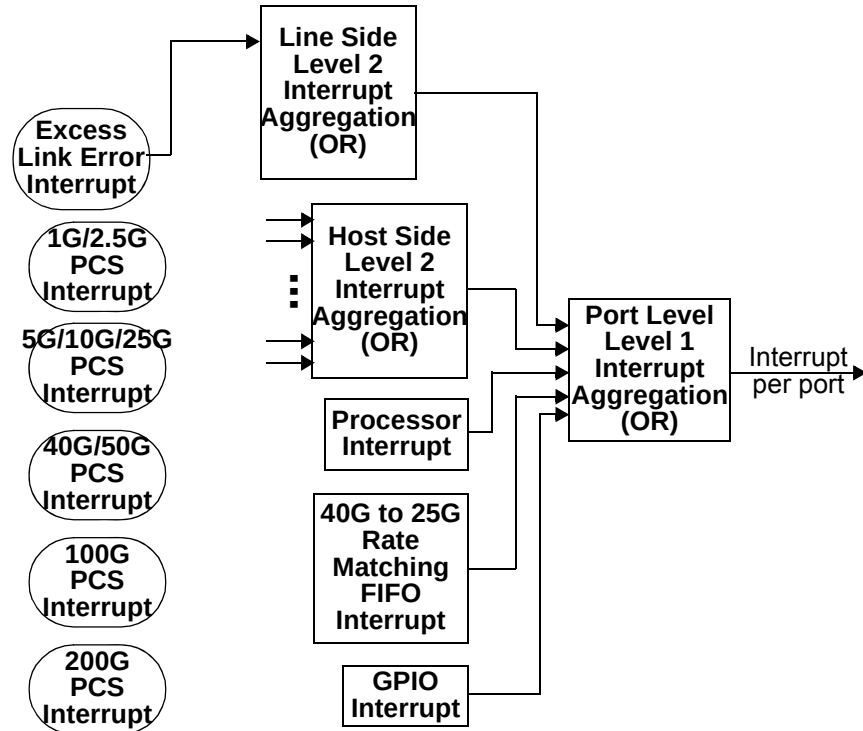
Figure 19: Interrupt Hierarchy and Aggregation from Different Blocks
