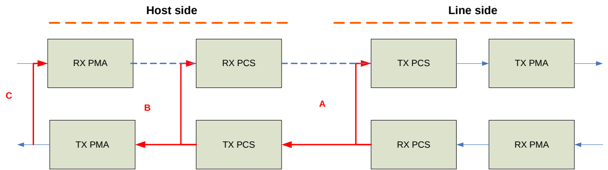
Figure 26: Line-side Loopback
