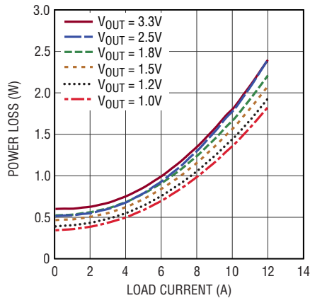
Figure 38. 5V IN Output Power Loss for Channel 0 and 3
