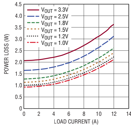
Figure 39. 12V IN Output Power Loss for Channel 0 and 3
