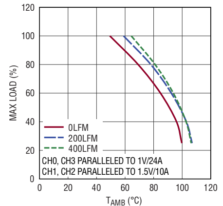
Figure 43. 12V IN Derating Curve, with Heat Sink
