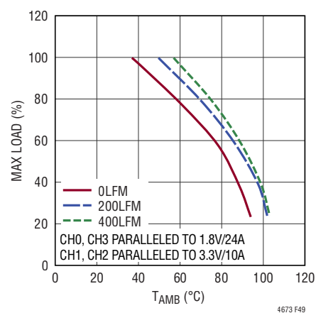
Figure 49. 12V IN Derating Curve, with Heat Sink
