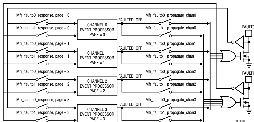
Figure 31. Channel Fault Management Block Diagram
