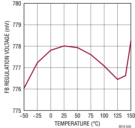
FB Voltage: LT8618
