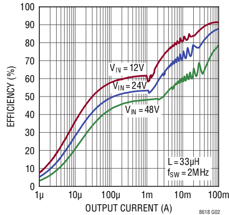
Efficiency (5V Output)
