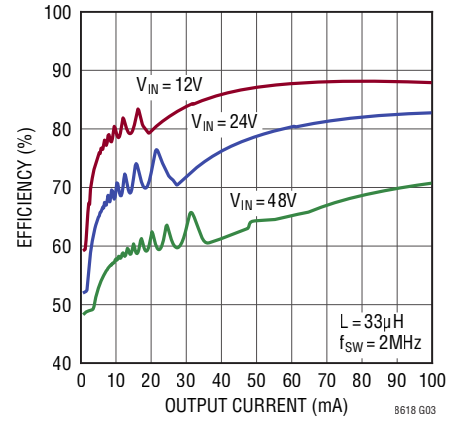
Efficiency (3.3V Output)
