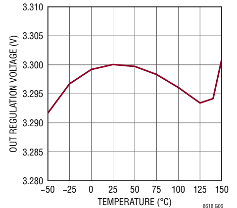
OUT Voltage: LT8618-3.3
