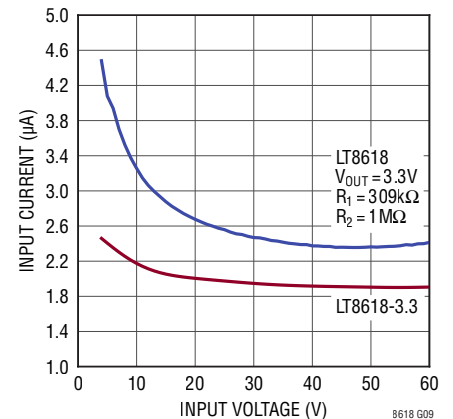
No-Load Supply Current (3.3V Output)
