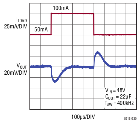
Switching Waveforms
