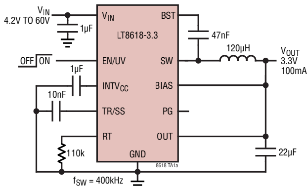
3.3V, Step-Down Converter
