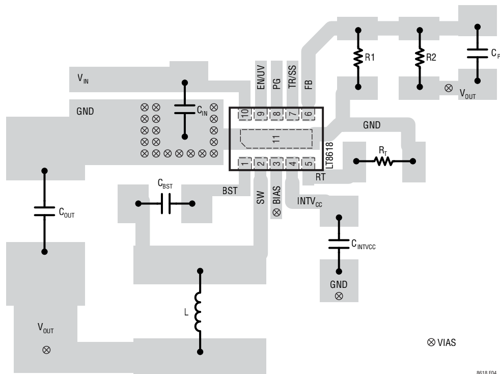
Figure 4. Recommended PCB Layout
