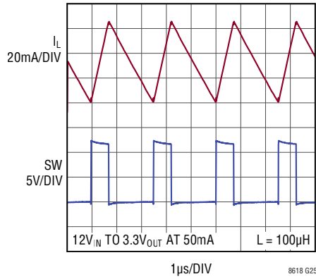
Switching Waveforms
