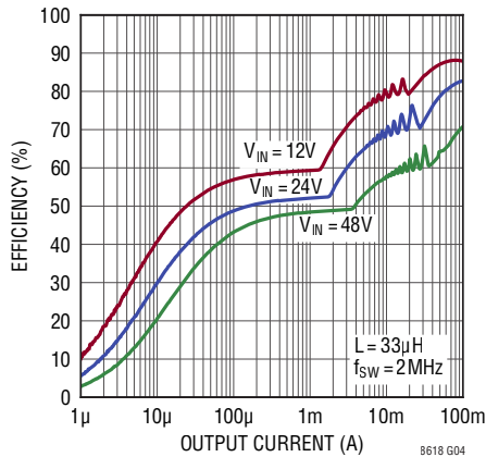
Efficiency (3.3V Output)
