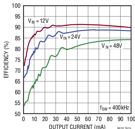
Efficiency at V OUT = 3.3V
