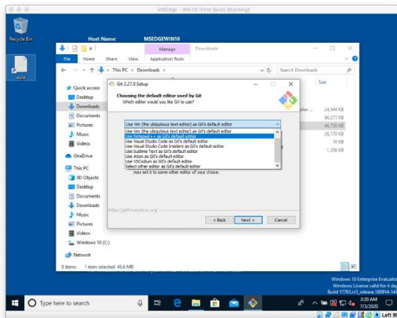
Figure 17. Installing Git
