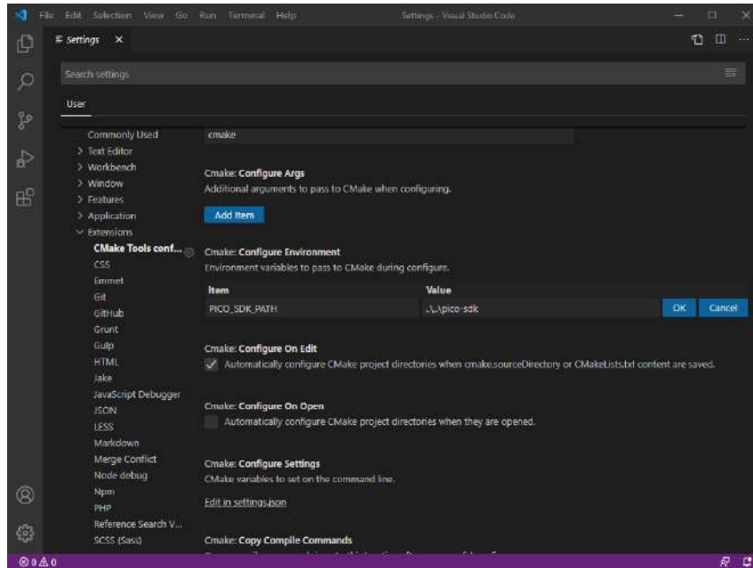
Figure 18. Setting PICO_SDK_PATH Environment Variable in the CMake Extension
