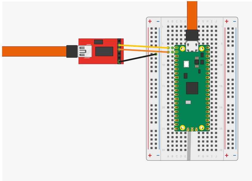
Figure 13. Sparkfun FTDI Basic adaptor connected to the Raspberry Pi Pico
