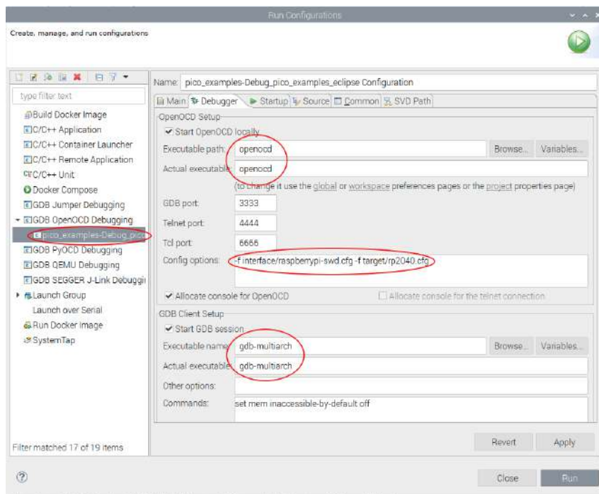
Figure 24. Setting up the Debugger and OpenOCD in Eclipse.
