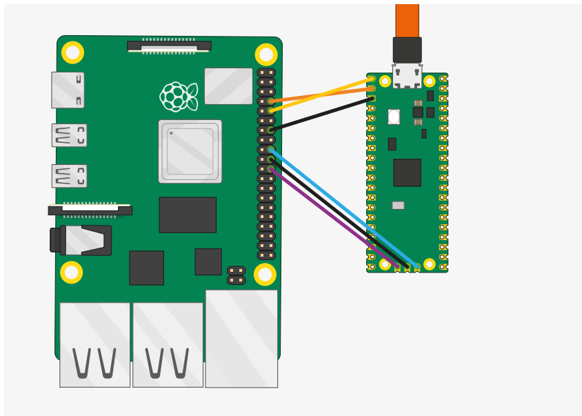
Figure 6. A Raspberry Pi 4 and the Raspberry Pi Pico with UART and SWD port connected together. Both are jumpered directly back to the Raspberry Pi 4 without using a breadboard.
