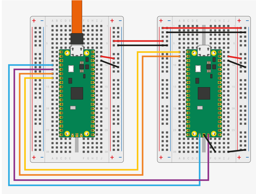
Figure 34. Wiring between Pico A (left) and Pico B (right) configuring Pico A as a debugger. Note that if Pico B is a USB Host then you'd want to hook VBUS up to VBUS so it can provide 5V instead of VSYS to VSYS.
