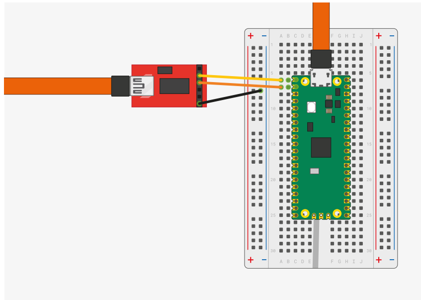
Figure 20. Sparkfun FTDI Basic adaptor connected to the Raspberry Pi Pico
