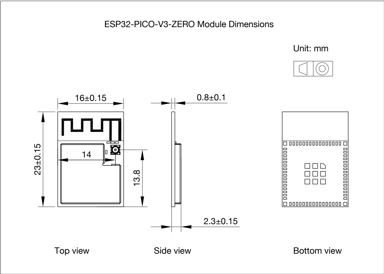
Figure 6: Physical Dimensions
