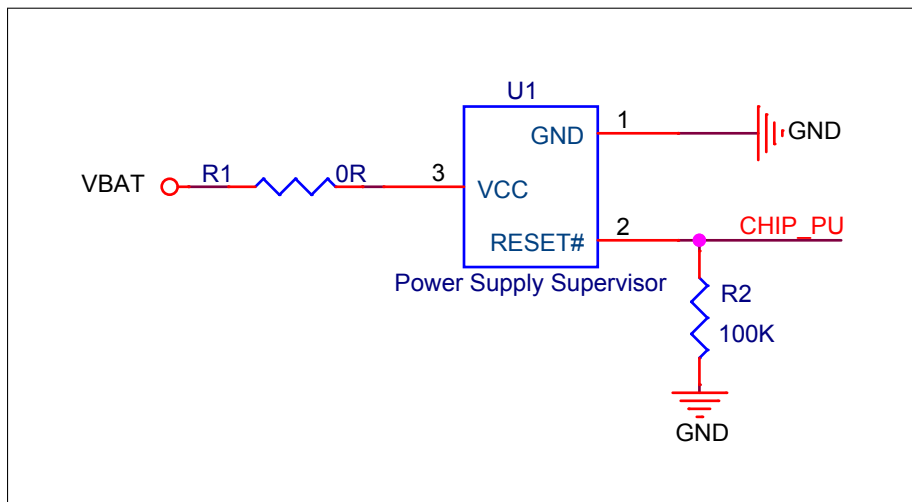
Figure 5: Reset Circuit
