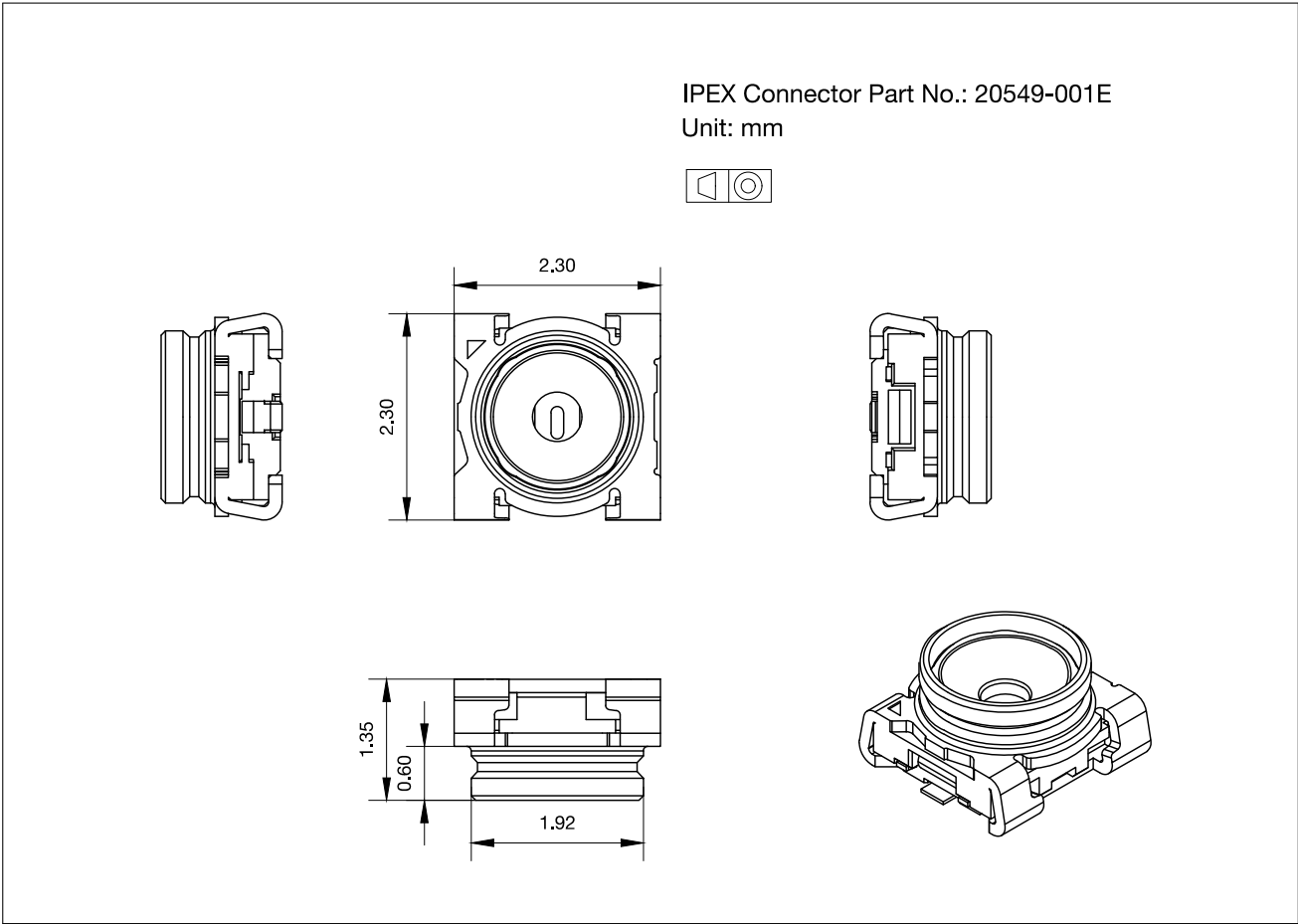
Figure 10: IPEX Connector Dimensions
