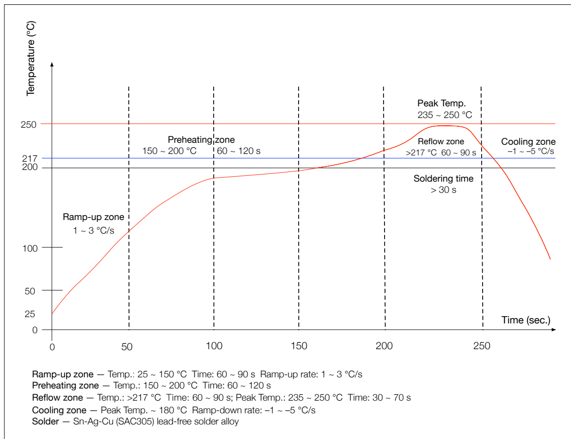
Figure 11: Reflow Profile
