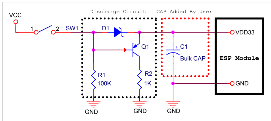
Figure 4: Discharge Circuit for VDD33 Rail
