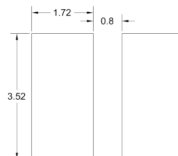
Recommended Stencil Pattern
