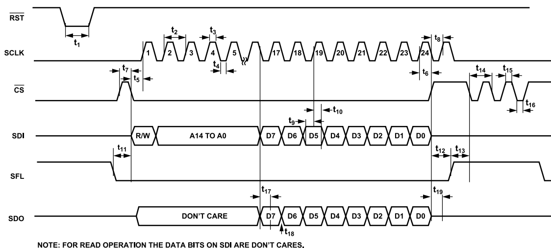
Figure 2. Timing Diagram
