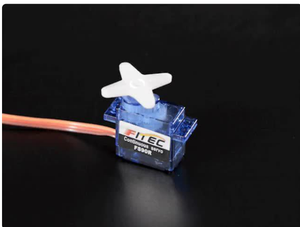
Continuous Rotation Micro Servo Need to make a tiny robot? This little micro servo rotates 360 degrees fully forward or backward, instead of moving to a single position. You can use any servo code, hardware,... https://www.adafruit.com/product/2442
