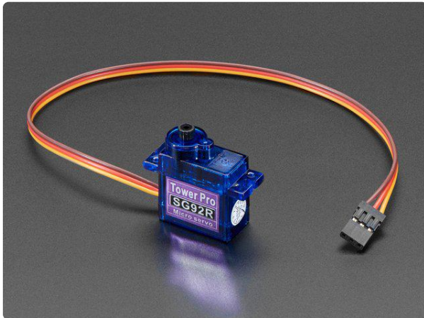
Micro servo Tiny little servo can rotate approximately 180 degrees (90 in each direction) and works just like the standard kinds you're used to but smaller. You can use any servo... https://www.adafruit.com/product/169
