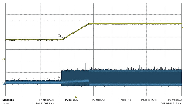
Fig. 8 - Pre-Bias Start-Up
