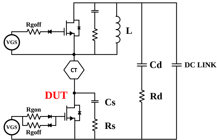
(a) Hard-switching snubber configuration
