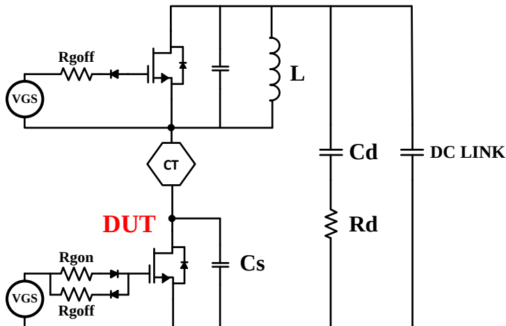
(b) Soft-switching snubber configuration
