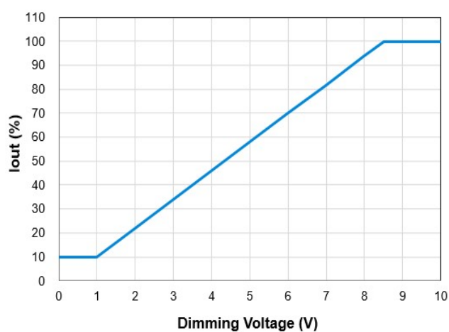
Dimming Curve
