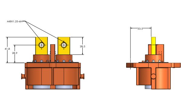
Busbar Type 1
