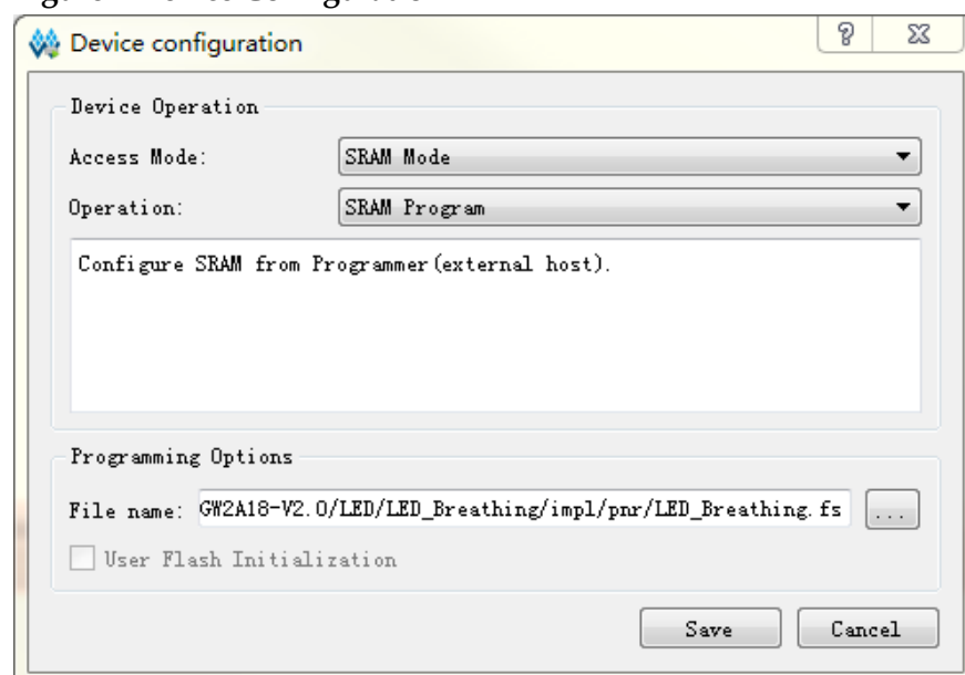
Figure 7 Device Configuration
