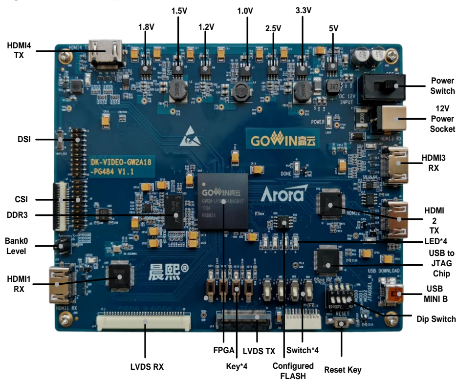
Figure 1 PCB Components
