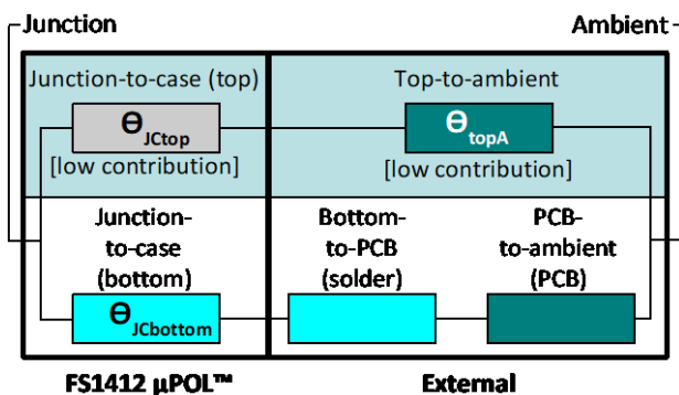
Figure 29 Thermal resistances of the FS1412
