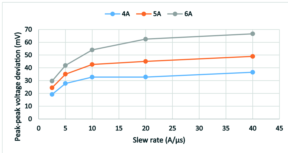
Figure 16 Peak-peak voltage deviation ( PV_{IN} = 12V , V_{OUT} = 1.8V , C_{OUT} = 4 \times 47 \mu F )
