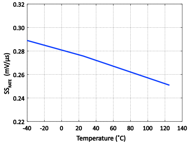
Soft-Start Rate
