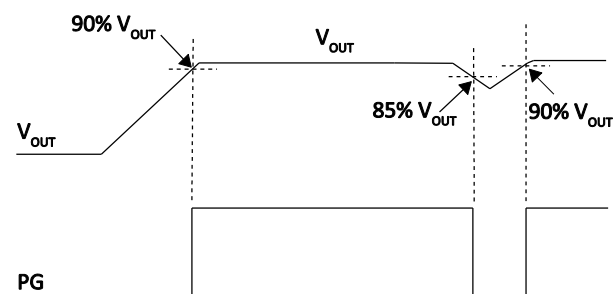
Figure 12 PG signal when PGControl bit=1
