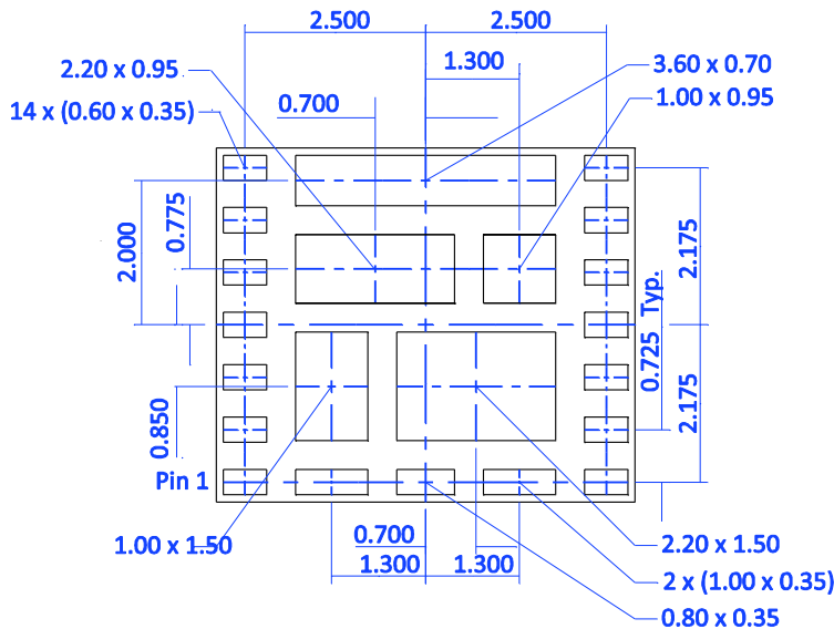
Figure 30 Dimensioned drawings
