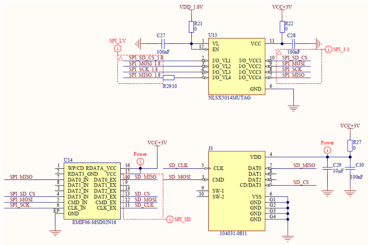
Figure 14. micro SD card connection
