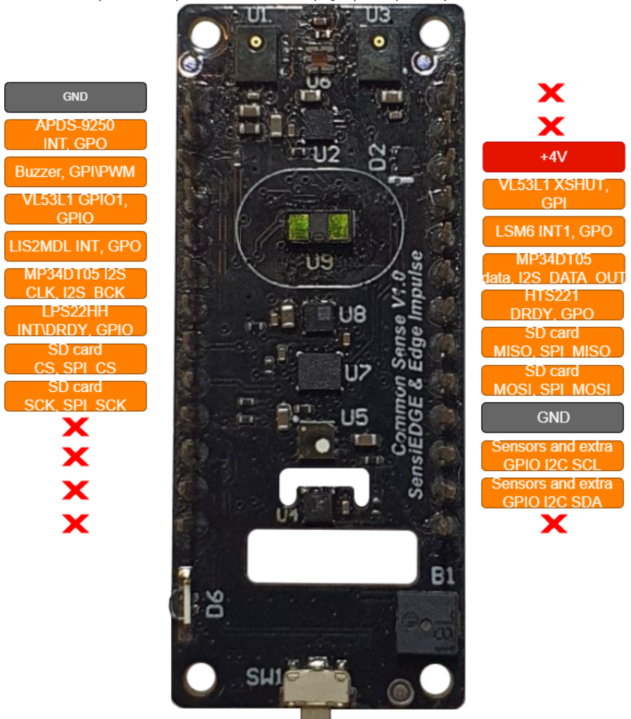
Figure 3. Sensors board pinout
