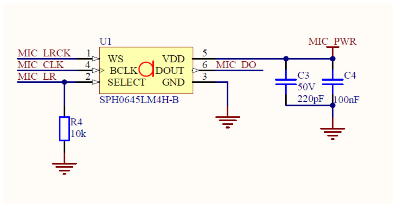
Figure 17. SPG0645LM4H connection
