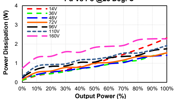
EC7AW18-72S15-ECRT Pd Vs Po @25 Deg. C
