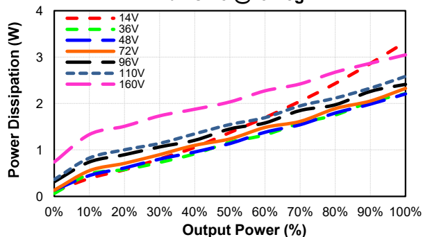
EC7AW18-72D05-ECRT Pd Vs Po @25 Deg. C
