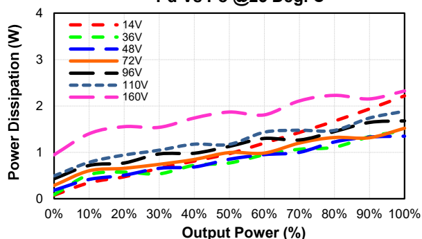
EC7AW18-72S12-ECRT Pd Vs Po @25 Deg. C
