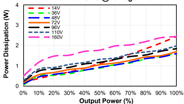
EC7AW18-72D12-ECRT Pd Vs Po @25 Deg. C
