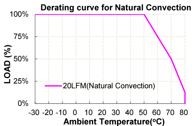
Power Derating
