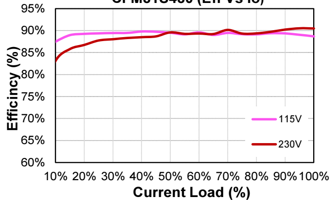
CFM81S480 (Eff Vs Io)
