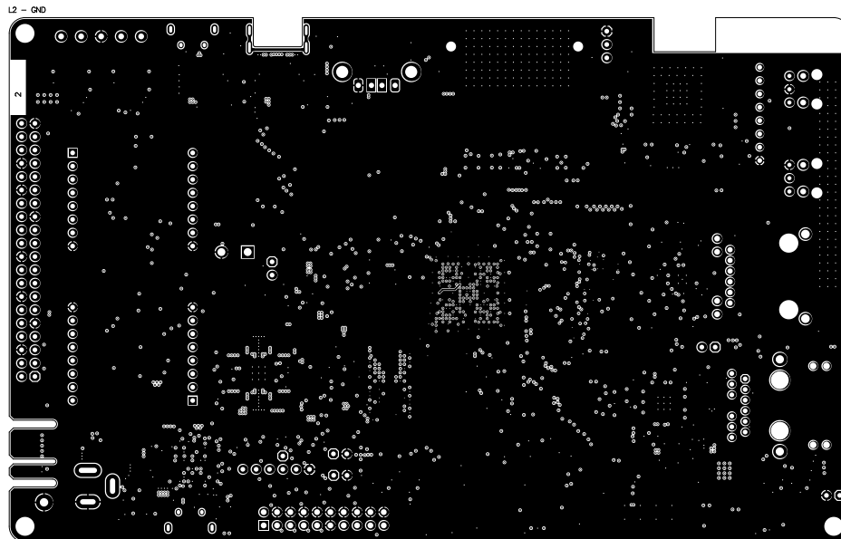
Figure 6-17. SAMA7G54-EK: Layer 2
