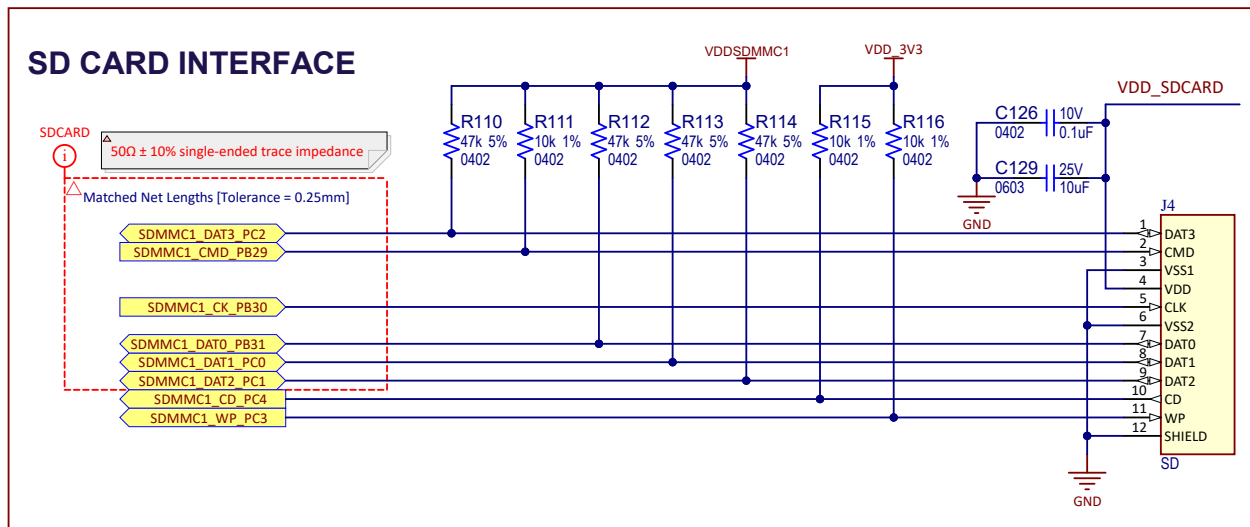
Figure 3-48. SD Card Interface Schematic
